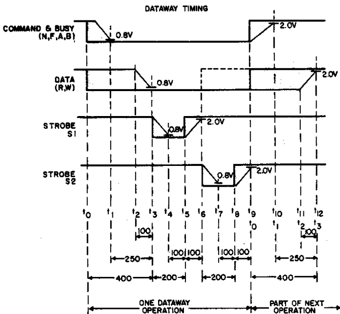
Times given are maximum values in nsec timing of a Dataway operation.
