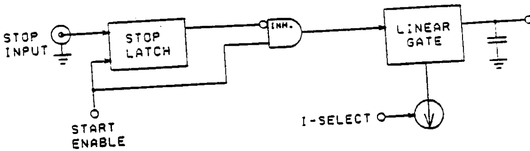
BLOCK DIAGRAM - STOP INPUT AND TAC SECTION
