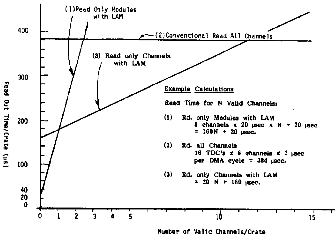
READ OUT TIME vs. VALID CHANNELS/CRATE
