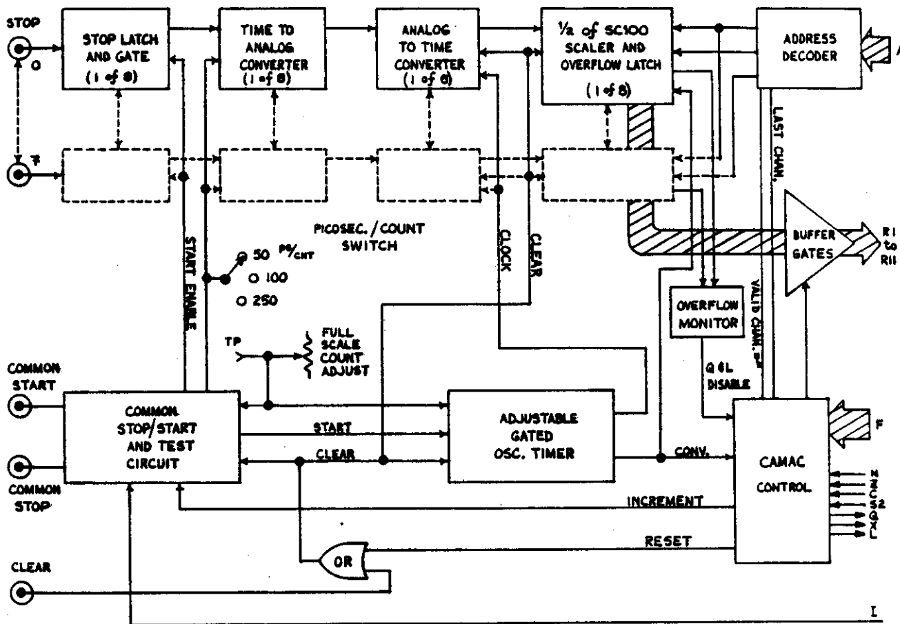
BLOCK DIAGRAM - MODEL 2228A TIME-TO-DIGITAL CONVERTER
