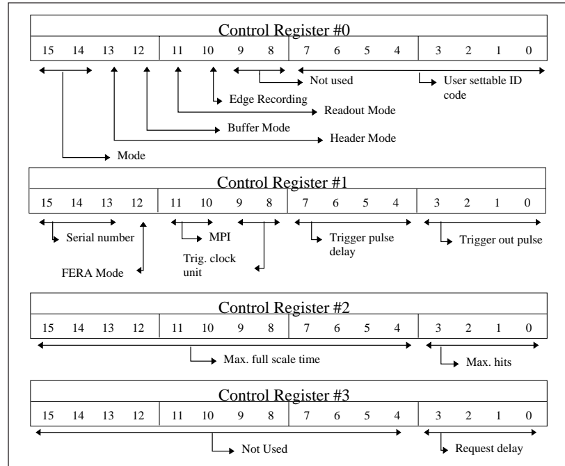
Mode 2 Control Registers
