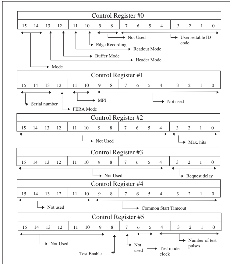
Mode 3 Control Registers
