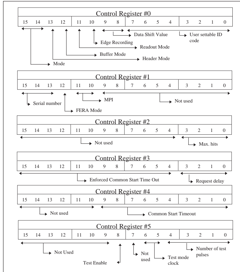
Mode 1 Control Registers
