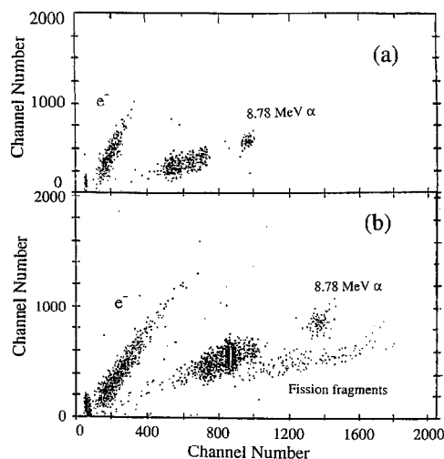
Fig. 6. Scatter plot showing the PID resolution by pulse shape discrimination. (a) shows the separation of \alpha particles and electrons or \gamma -rays from a source of ^{232}\text{U} . A prototype preamplifier and electronics module were used. (b) Separation by PSD of electrons, \alpha particles and fission fragments from a ^{252}\text{Cf} source is seen. The detector was covered by 0.29 \text{mg}/\text{cm}^2 aluminized Mylar.
