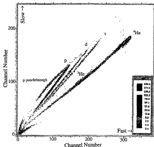
Fig. 7. Color scatter plot showing the PID resolution by pulse-shape discrimination using a 1.9 mm detector. The reaction was 43 MeV ^4\text{He} on ^{197}\text{Au} . The p, d, t separation is clearly seen. The separation of \alpha particles from the hydrogen isotopes is apparent for all energies down to very low energy. The proton punchthrough energy here is 19.9 MeV. The data were from the calibration run of an experiment in Gammasphere.
