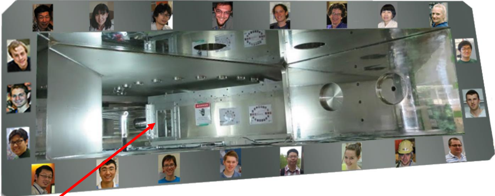
\pi RIT TPC inserted inside the SAMURAI Magnet Chamber 7/23/2014
