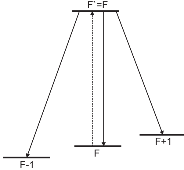
Figure 2.6: Schematic diagram of the hyperfine pumping effect. Electrons are excited from F to F' and subsequently decay to F - 1 , F , or F + 1 .
