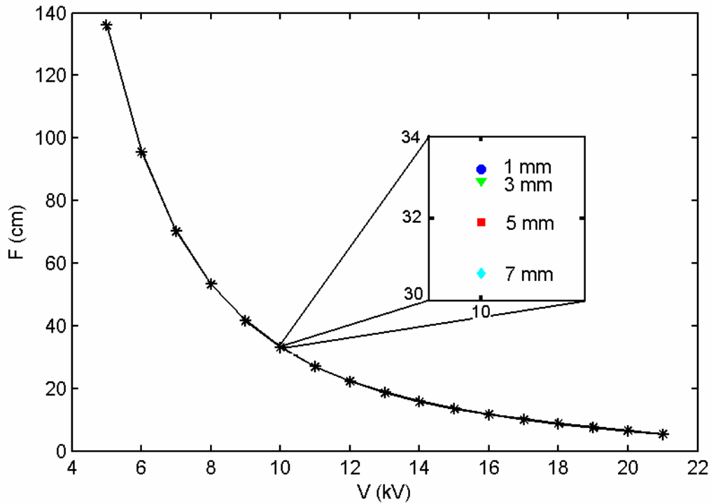
Figure 8: Focusing distance of the Einzel lens when biased to different voltages for a 20 keV beam. The picture was expanded for 10 kV. The non-linear effects of the lens can be observed in the dispersion of the focusing distances for ions entering the source 1, 3, 5 and 7mm away from the beam axis.
