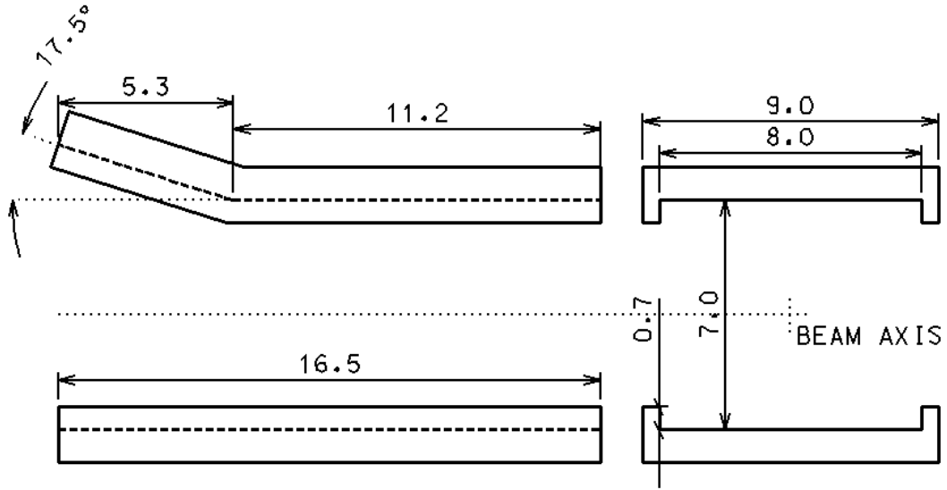
Figure 21: Front and side view of the Inflector Plates where main dimensions (in cm) are specified.
