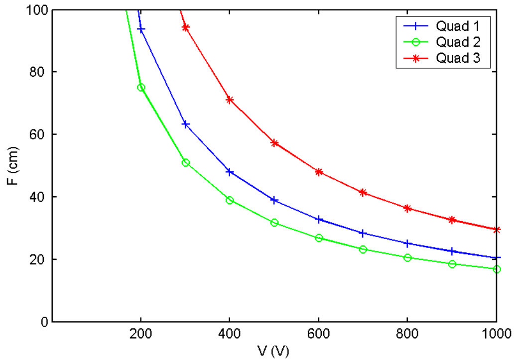
Figure 15: Focusing length for a 20 keV beam of the three quadrupoles used in the injection line of SIR.
