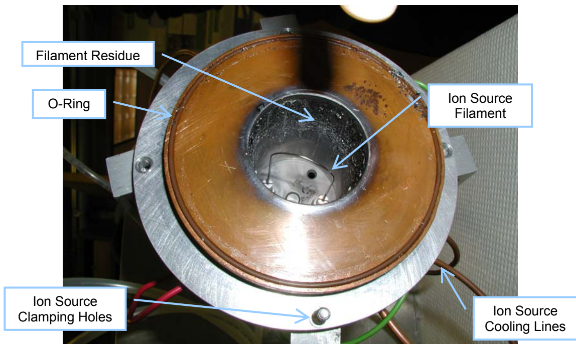
Figure 103: Picture of the broken filament in the ion source
