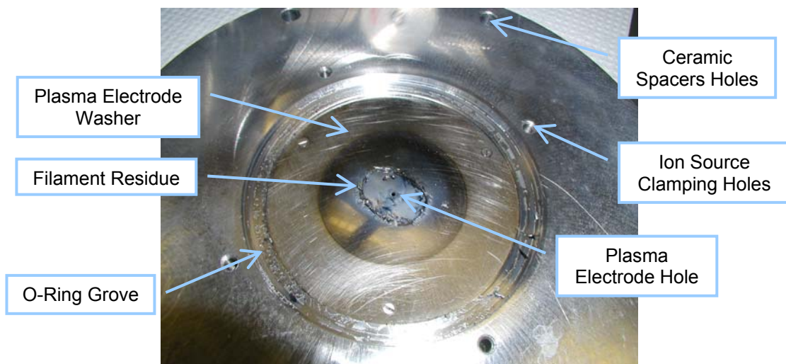
Figure 102: Picture of the flange that holds the ion source and the plasma electrode washer.
