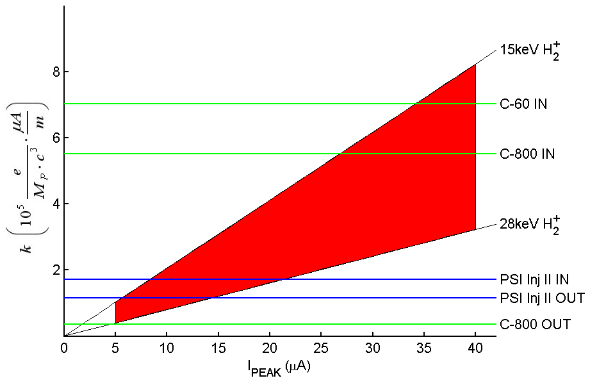
Figure 2: The space charge regime, defined by the scaling factor k , in which SIR can operate is displayed in shaded red. The value of the scaling factors for other machines described in section 1.1 are represented by horizontal lines. The tag IN refers to the first revolution in those machines, while the tag OUT refers to the last revolution.
