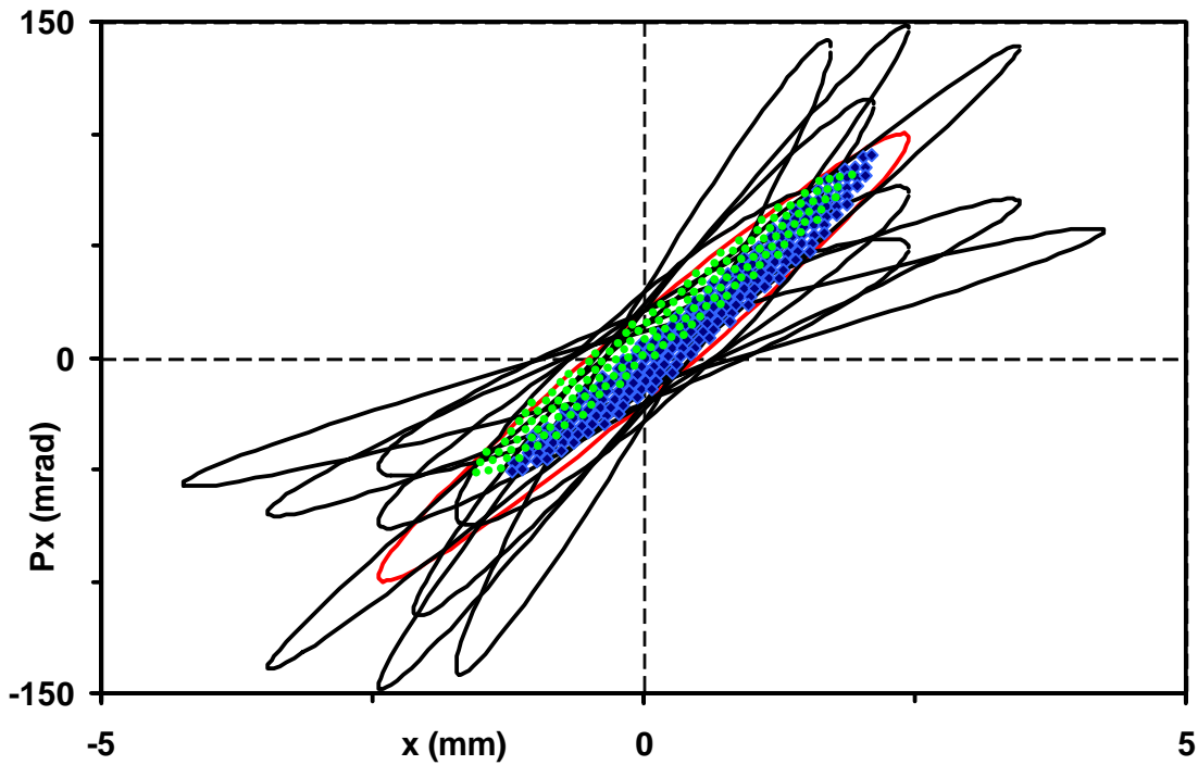
Figure 23: Ions representing different points of the phase space (measured with the emittance measurement system) were tracked back to the source and plotted in green and blue. An ellipse representing this ensemble in red and variations on this ellipse in black can be accommodated by the injection line and matched to the closed orbit solution of the ring when injected.
