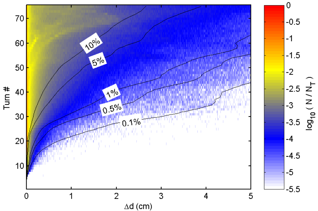
Figure 82: Effect in the evolution of the position of the macroparticles when one of them is removed from the initial ensemble. The percentage of particles that have been displaced \Delta d at a given turn number is represented with different colors. The percentage of particles that have been displaced more than \Delta d at a given turn number is represented by contour lines.
