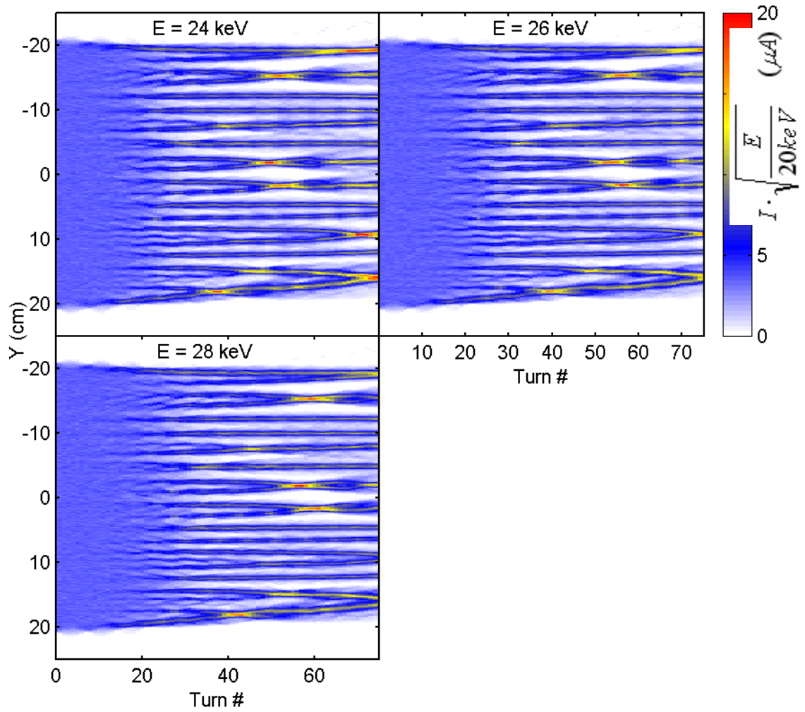
Figure 76: Waterfall diagrams representing the evolution of the longitudinal bunch profile for energies ranging from 24 keV to 28 keV. The other parameters that characterize the bunch are listed in Table 12.
