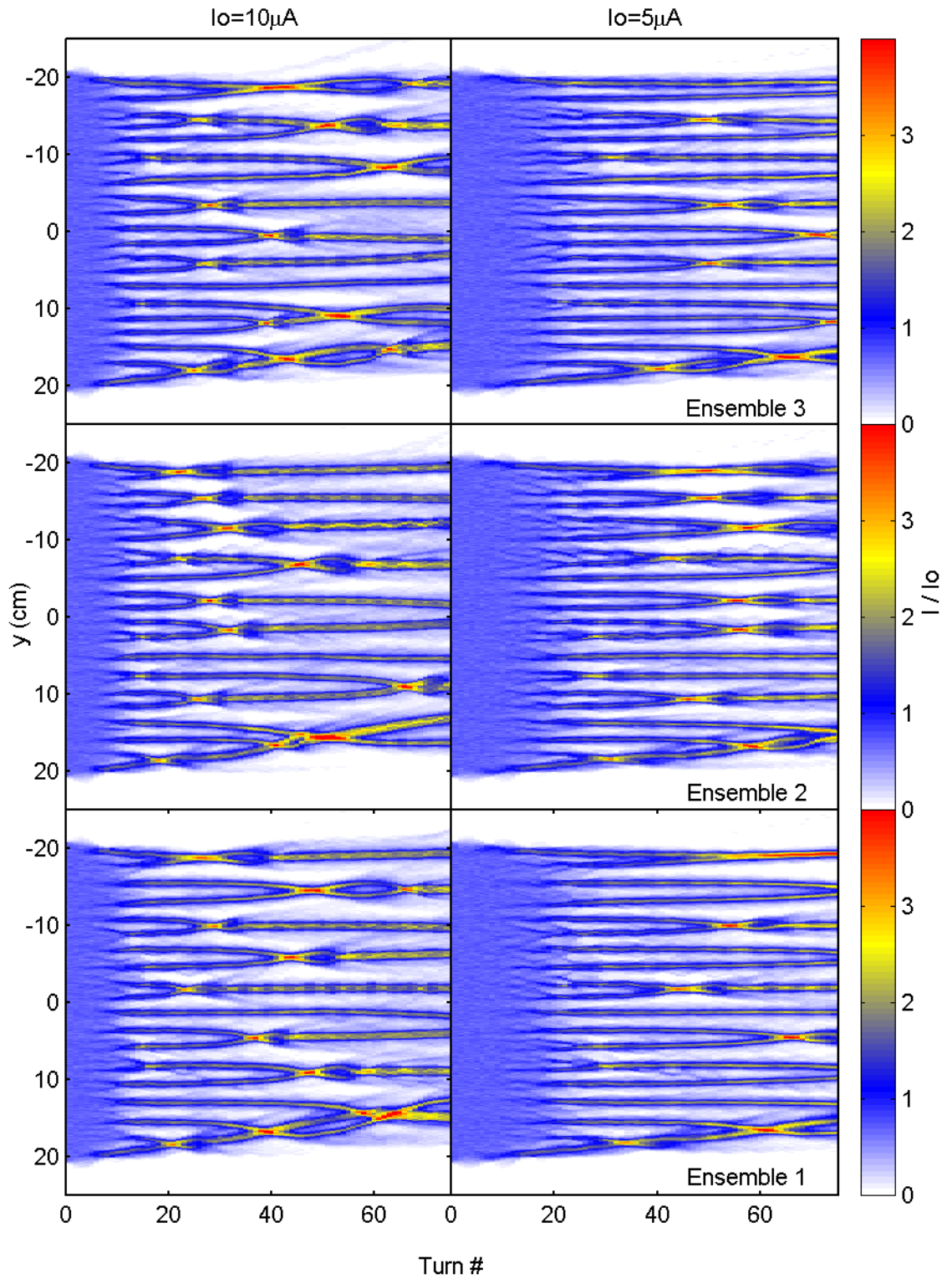
Figure 65: Evolution of the longitudinal profile of three different microscopic representations of a bunch with the characteristics listed in Table 8. Two different peak currents were used to compare characteristics of the evolution.
