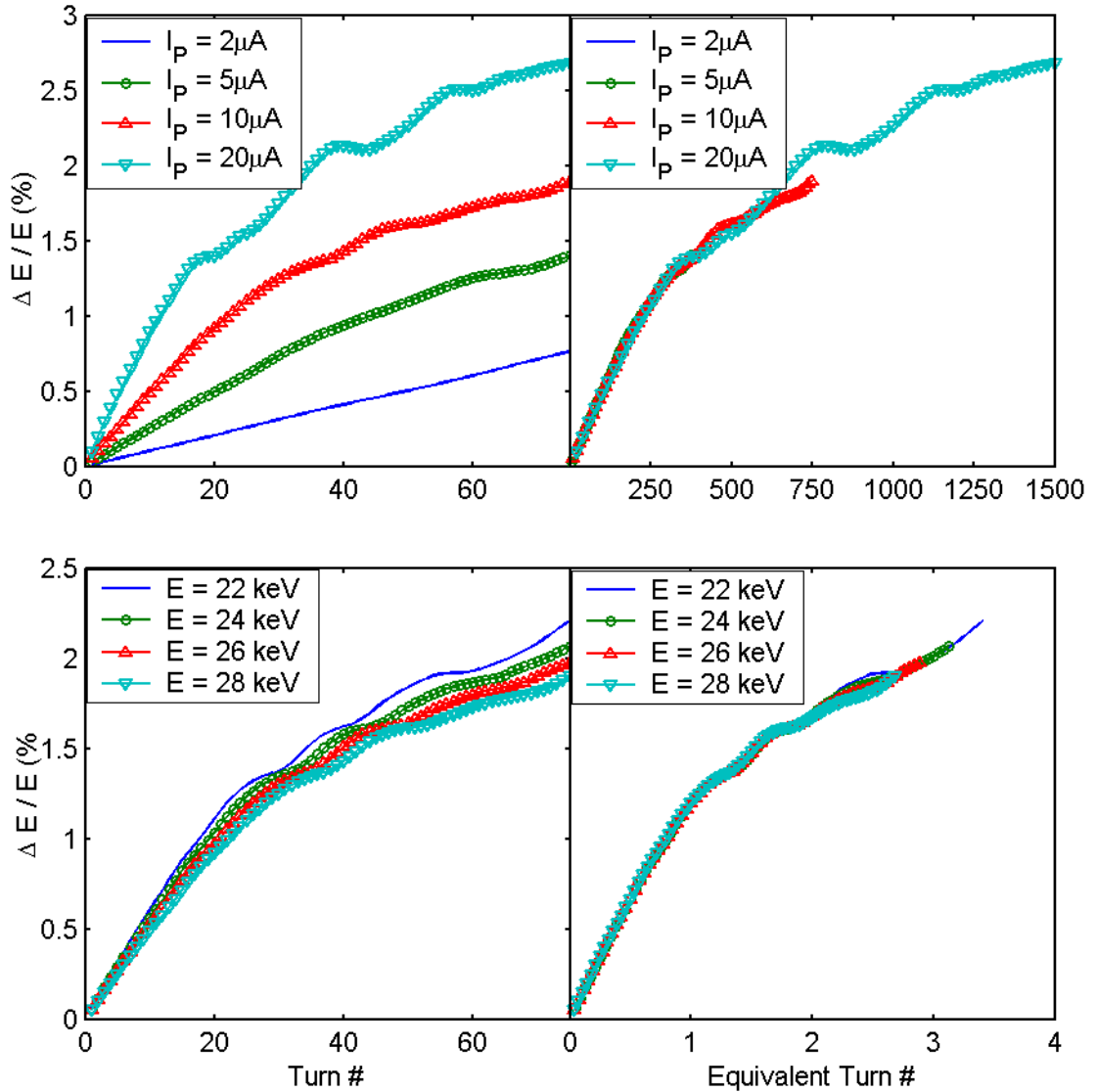
Figure 83: Energy spread induced by space charge forces as a function of the turn number for different beam energies (bottom of figure) and different beam currents (top of figure). The same data is displayed on the right as a function of the equivalent turn number. The rest of the parameters of the bunches are specified in Table 17.
