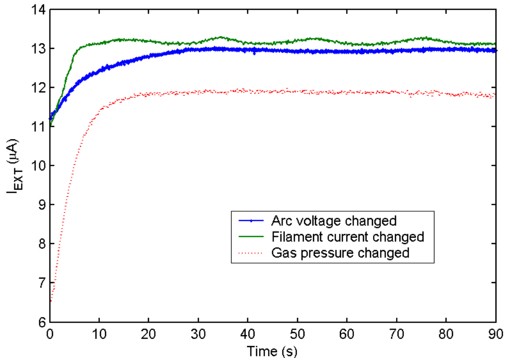
Figure 48: Variability of the extracted beam current when the conditions in the ion source are changed.
