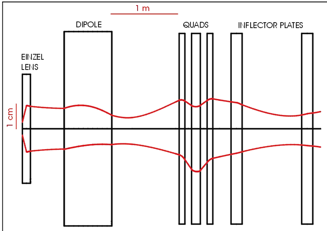
Figure 24: Envelope of the beam as it moves in the injection line of the SIR. The curve on top is the vertical beam envelope (perpendicular to the medium plane of the ring). The bottom curve corresponds to the beam envelope in the horizontal plane.
