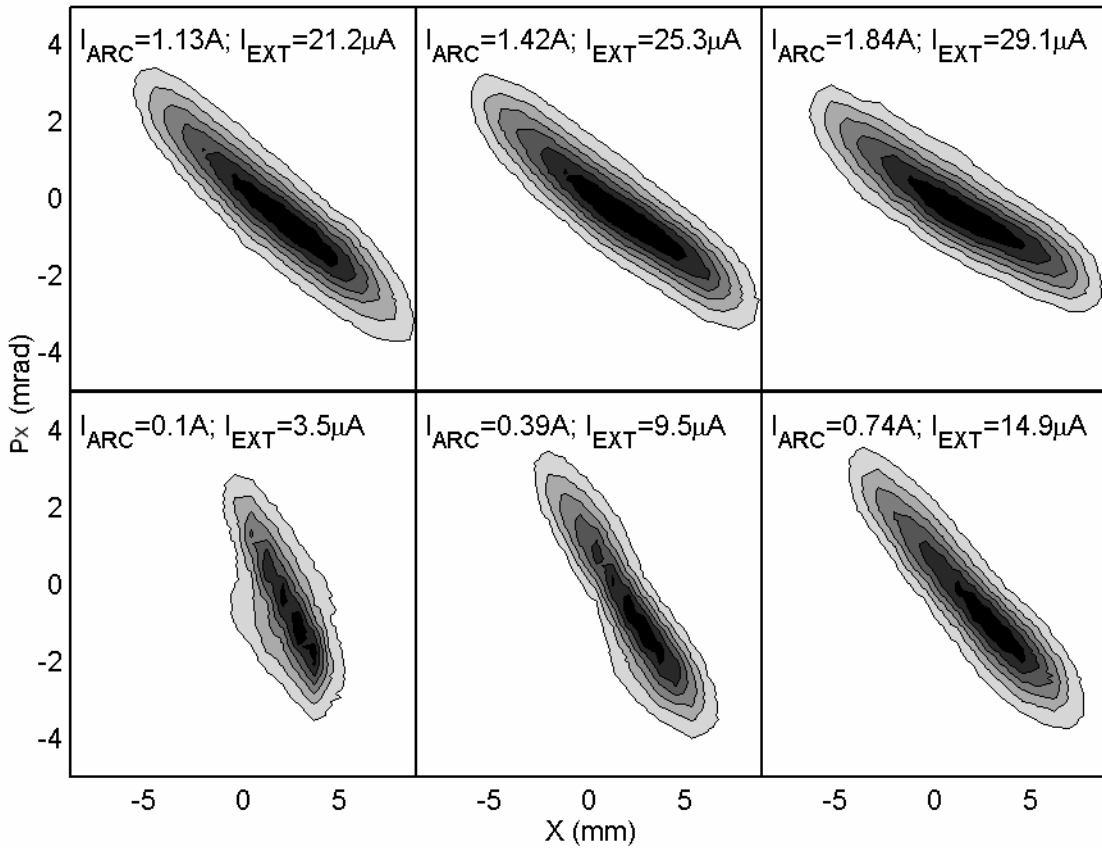
Figure 53: X-Px phase space measurements for different extraction currents. (We define the x plane as that parallel to the medium plane of the ring.) The corresponding arc current and extracted beam current are shown in the figure. The rest of the source parameters are listed in Table 5. Growth in the emittance and in the tilt of the beam when the extracted current is increased (due to stronger transverse space charge effects in the extraction region) can be observed.
