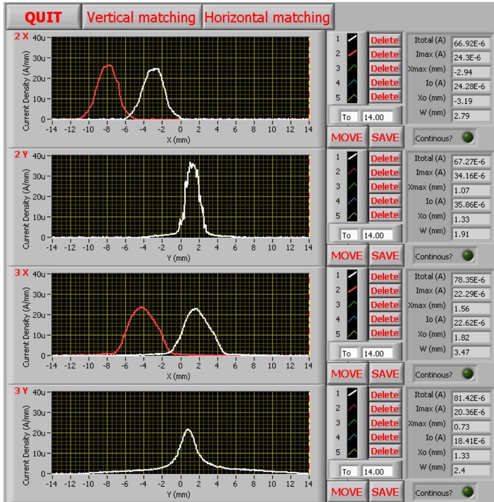
Figure 34: Front panel of the LabVIEW program used to control de scanning wires.
