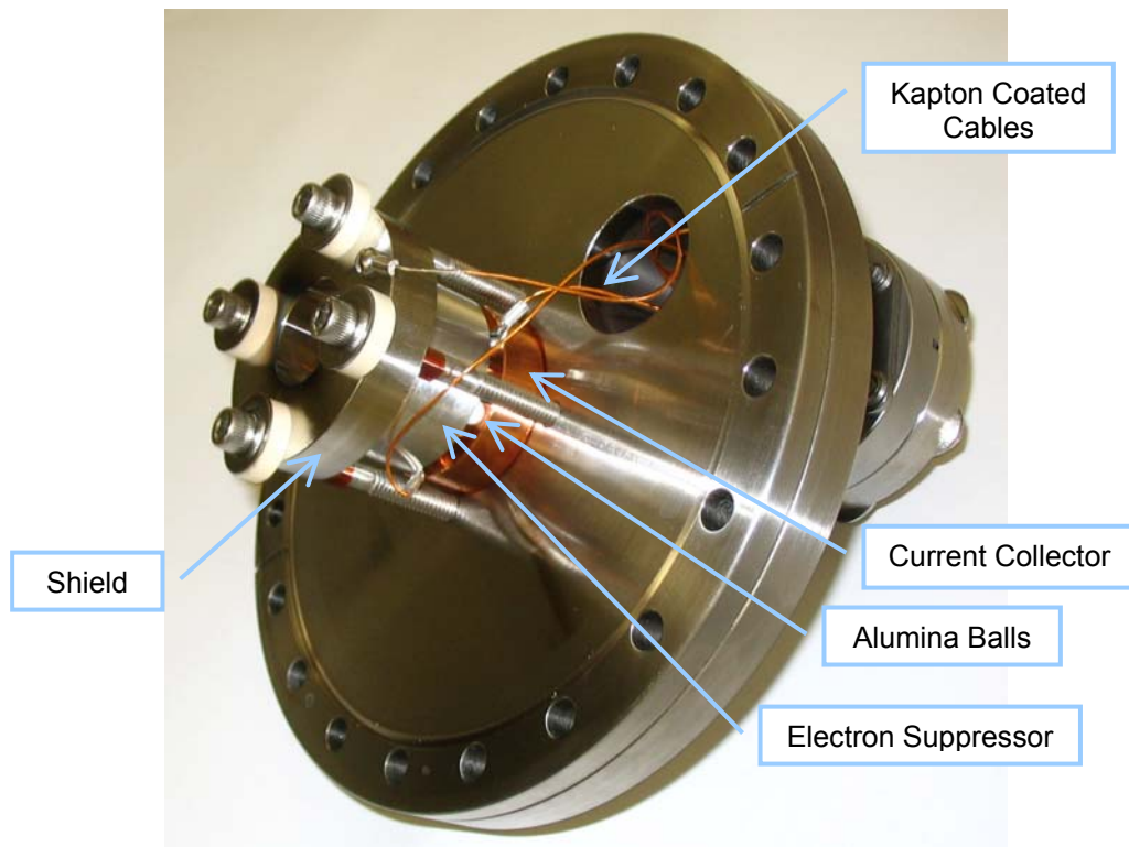
Figure 22: Picture of the Faraday cup at the end of the injection line of SIR.
