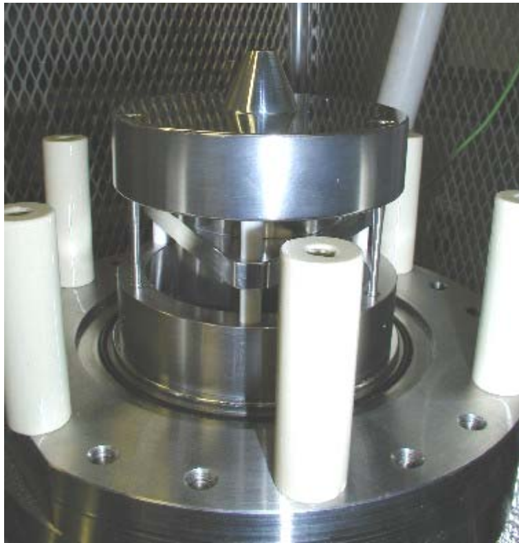
Figure 6: Picture of the Einzel lens and puller of the ion source used in the injection line of SIR.
