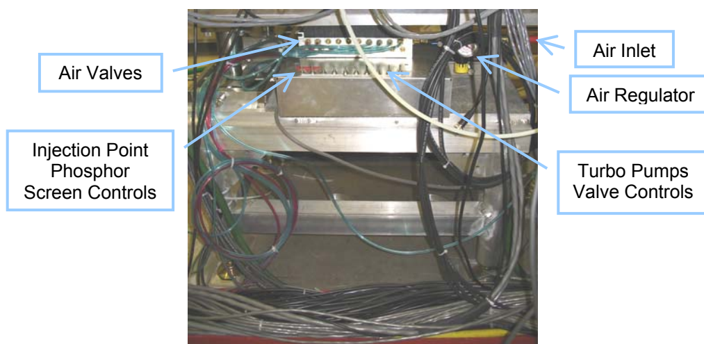
Figure 100: Picture of the compressed air control system. The two furthest left switches are used to position the injection point phosphor screen. The four furthest right switches open or close the valves in between turbo pumps and mechanical pumps.
