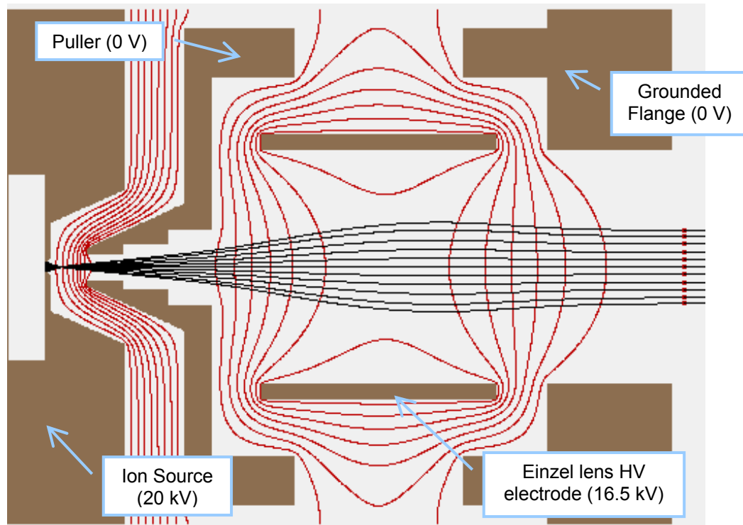
Figure 7: Simion model of the Einzel lens and source extraction region of the injection line of SIR. Equipotential lines are shown in red. Several ions were tracked and their trajectories are displayed in black.
