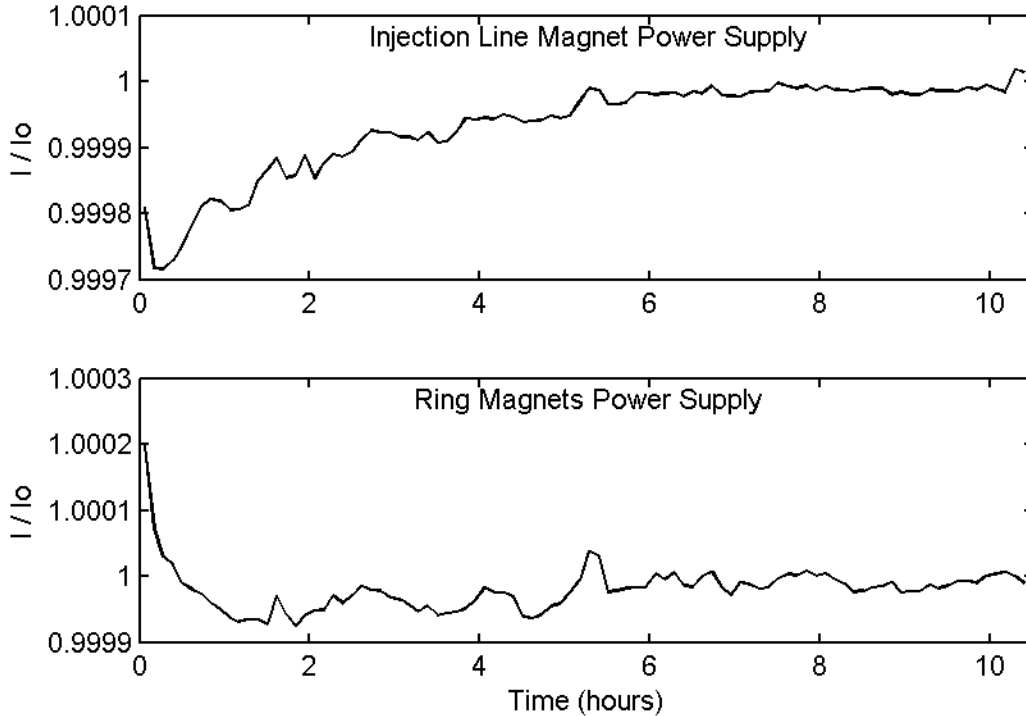
Figure 46: Long term variability of the injection line and ring dipoles power supply. I_0 is 109 A that corresponds to a 21 keV H_2^+ beam. Deviations around this value were monitored over a 10 hour period of time.
