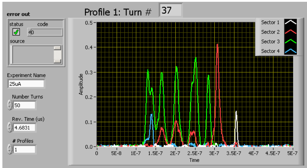
Figure 41: Front panel of the LabVIEW program used for the data acquisition of the sector faraday cup.
