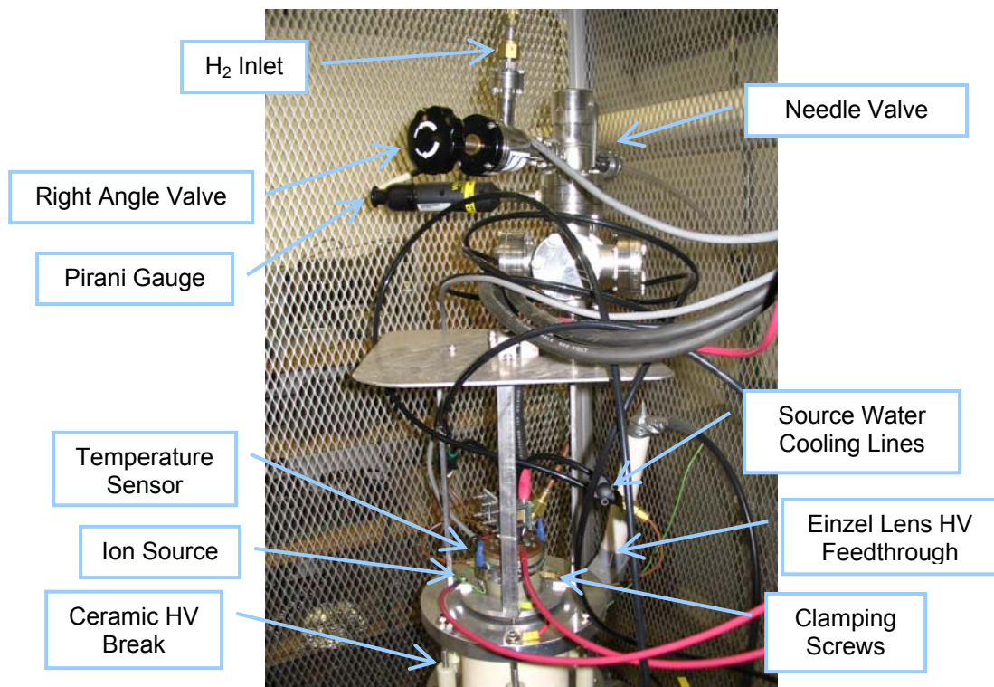
Figure 94: Picture of the ion Source and its associated gas handling system.
