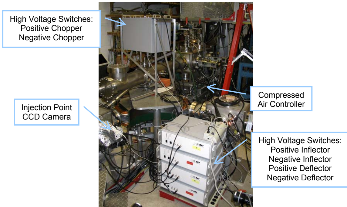
Figure 101: Picture of the fast high voltage switches used to pulse the chopper, second pair of inflector plates and deflector plates.
