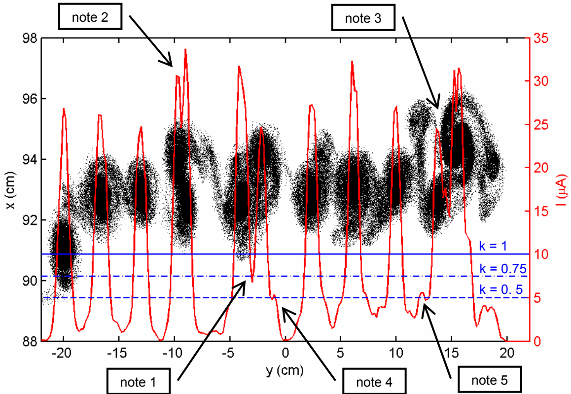
Figure 59: Top view (in black) and longitudinal profile (in red) of a \text{H}_2^+ bunch 60 turns after being injected. The energy when it was injected was 20 keV, the peak current 10\mu\text{A} , the length 300 ns and the emittance 30\pi\text{ mm mrad} .
