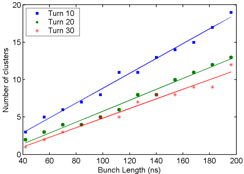
Figure 68: Number of clusters formed after 10, 20 and 30 revolutions for different initial bunch lengths. The computational and physical parameters used in the simulations are listed in Table 10.
