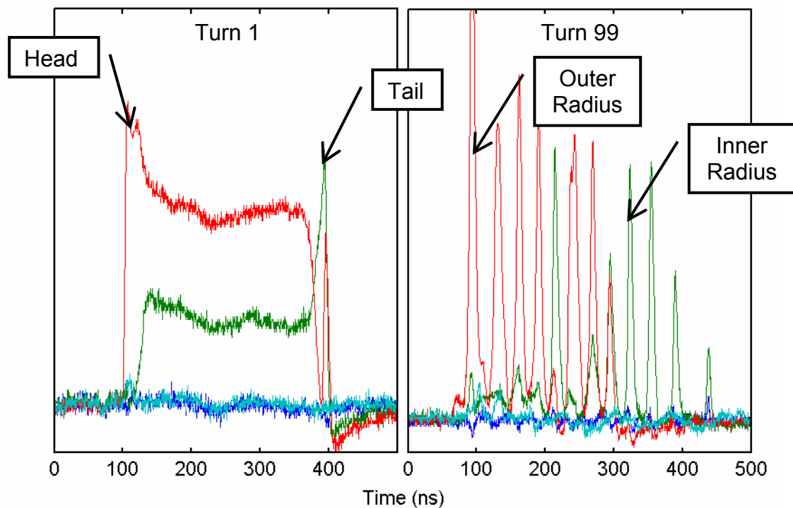
Figure 90: Correlation between energy of the ions and radial position. When the bunch is extracted after \frac{1}{2} a revolution, it hits part of the two central electrodes of sector Faraday cup (green and red). After 99\frac{1}{2} revolutions, those clusters in the head of the bunch hit the outer radius central electrode while those in the tail hit the inner radius electrode.
