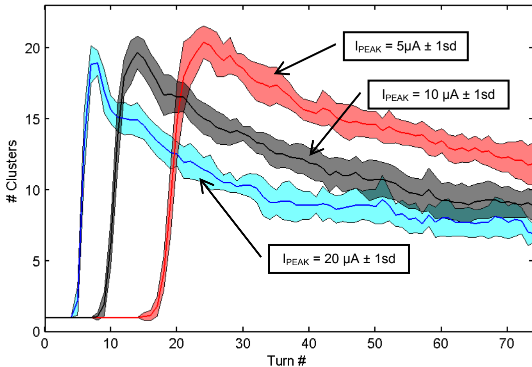
Figure 67: Average value and standard deviation of the number of clusters formed for three different peak currents. The dispersion in values is due to the choice of the microscopic representation of the bunch.
