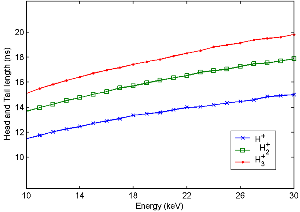
Figure 19: Length of the head and tail of the bunches produced by the chopper for different ion masses and energies.
