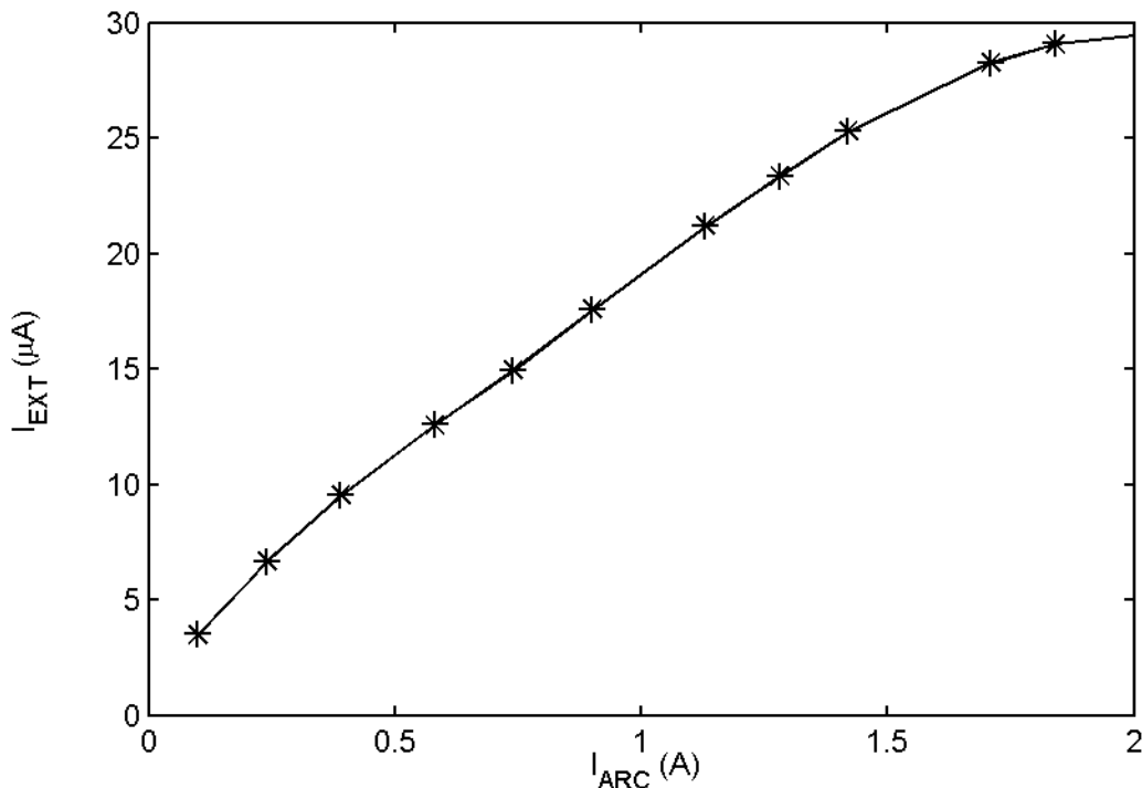
Figure 51: Relationship between arc current and the extraction current of H_2^+ ions when the filament power is changed as shown in Figure 52. The value of the arc voltage, extraction voltage and pressure are kept constant. (Values are listed in Table 5.)
