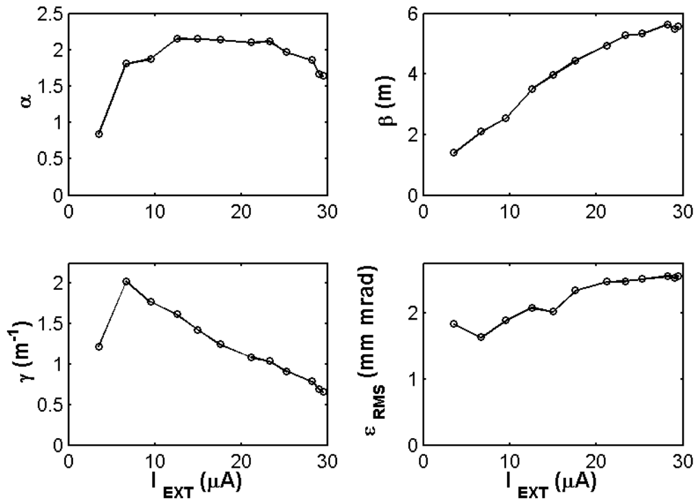
Figure 54: Value of the RMS-emittance and the Courant-Snyder parameters as a function of the extracted beam current for the source conditions listed in Table 5.
