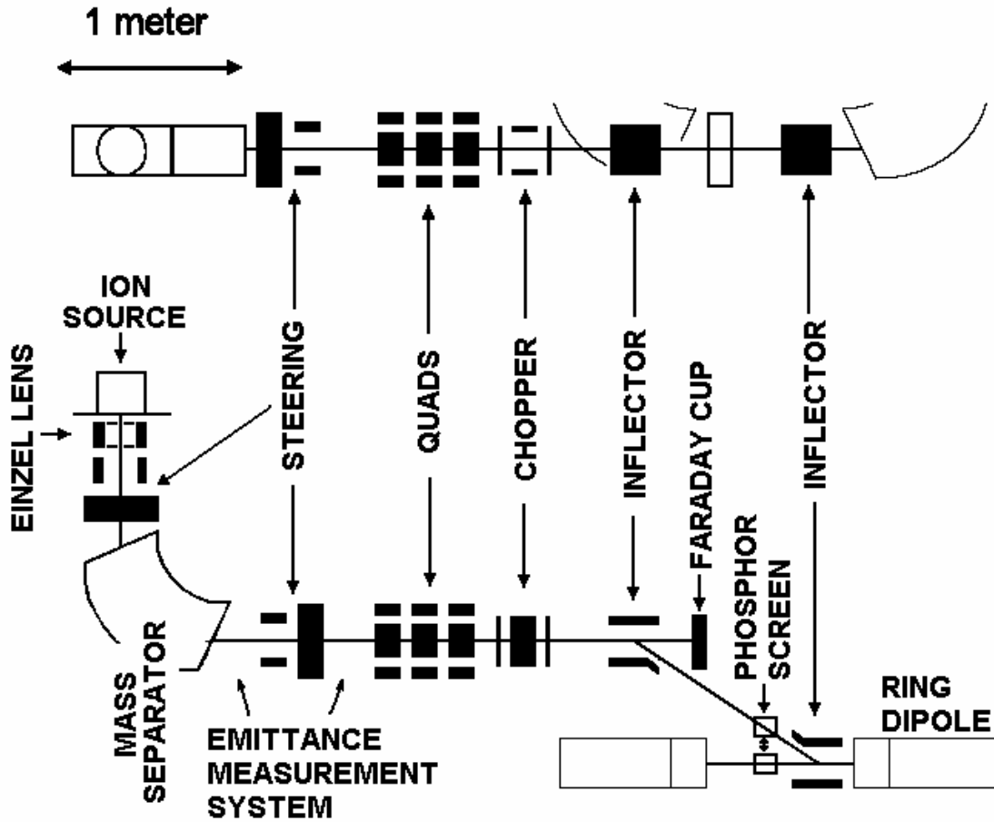
Figure 3: Schematic top and side view of the injection line of SIR.
