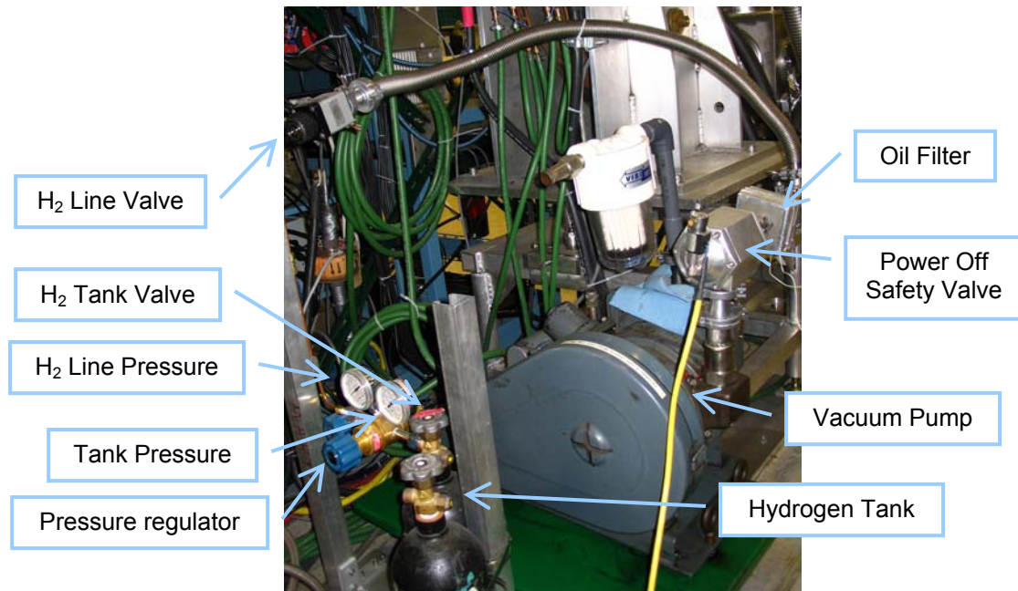
Figure 95: Picture of the hydrogen tank and regulator.
