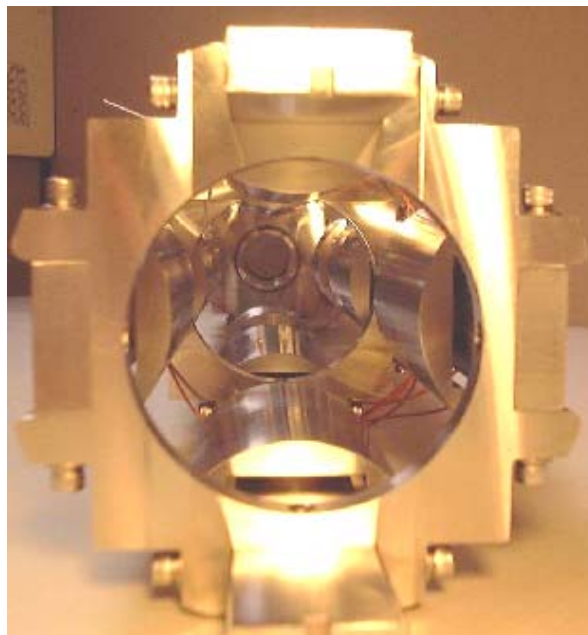
Figure 14: Picture of the triplet of electrostatic quadrupoles used in the injection line of SIR.
