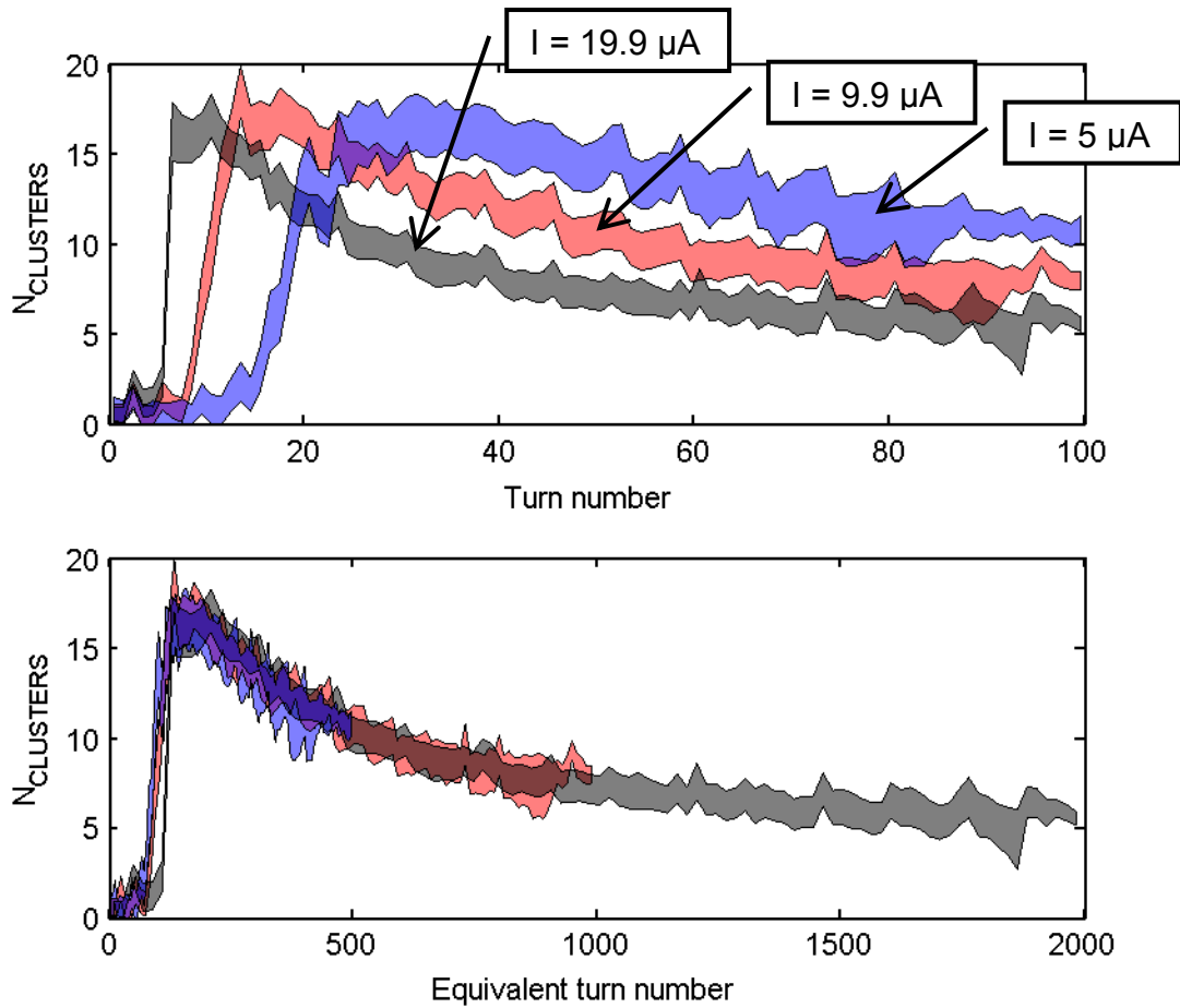
Figure 89: Experimental verification of the scaling law with the bunch current. The number of clusters counted for bunches with characteristics listed in Table 21 scales with the peak current of the bunches as it can be seen in the bottom of the figure where the number of clusters is plotted as a function of the equivalent turn number.
