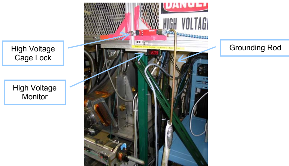
Figure 93: Picture of the high voltage monitor, grounding rod and lock of the ion source high voltage cage.
