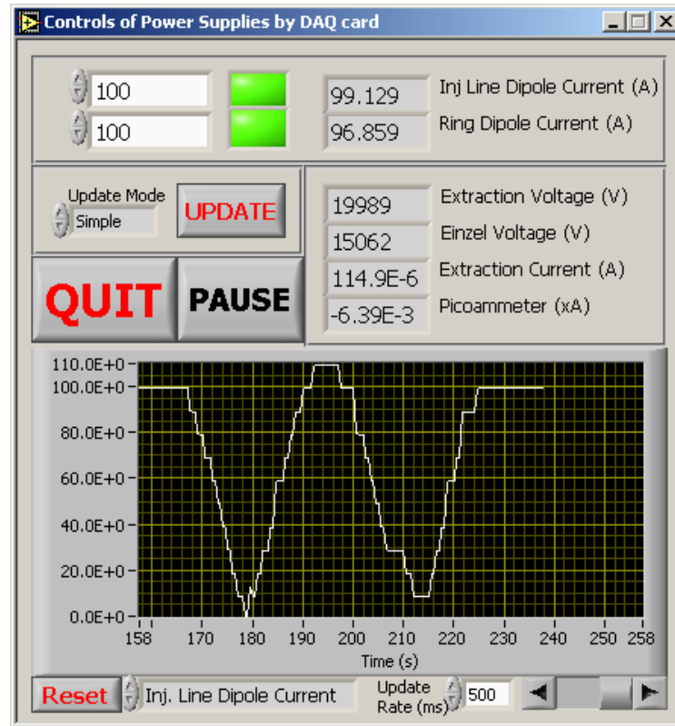
Figure 43: Front panel of the LabVIEW program to control the dipoles, extraction and Einzel lens power supplies.
