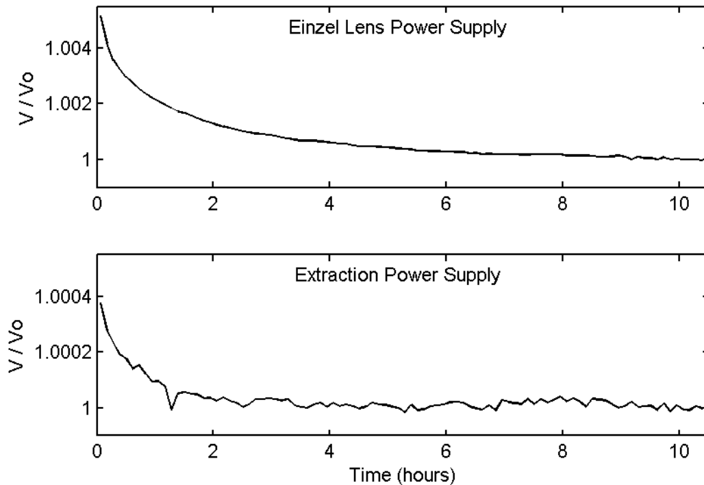
Figure 47: Long term variability of the extraction and Einzel lens power supplies. V_0 for the Einzel lens power supply is 16.5 kV and for the extraction power supply is 20 kV. The variability of these voltages was monitored over a period of 10 hours.
