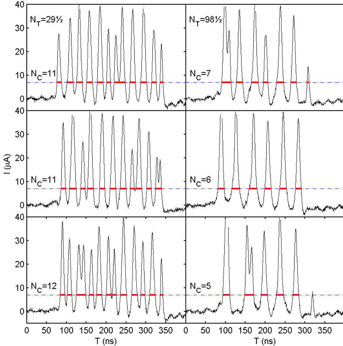
Figure 86: Longitudinal bunch profiles measured with the sector Faraday cup after the bunch was stored for 29 ½ turns (on the left) and 98 ½ (on the right). The characteristics of the bunches, when they were injected, are listed in Table 18. The number of clusters counted ( N_C ) is shown next to the corresponding profile.
