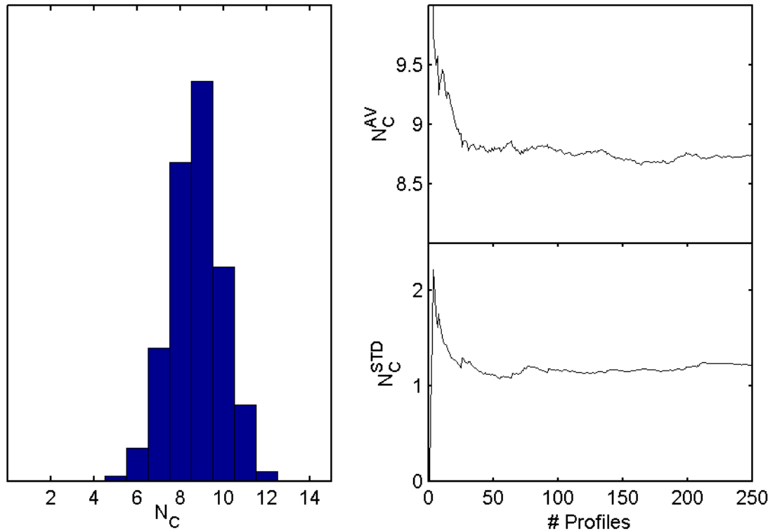
Figure 87: Dispersion in the number of clusters counted ( N_C ) when a bunch with the characteristics listed in Table 19 was extracted after 55 turns (on the left). Convergence in the average ( N_C^{AV} ) and standard deviation ( N_C^{STD} ) of the number of clusters counted as the number of profiles included is increased (on the right).
