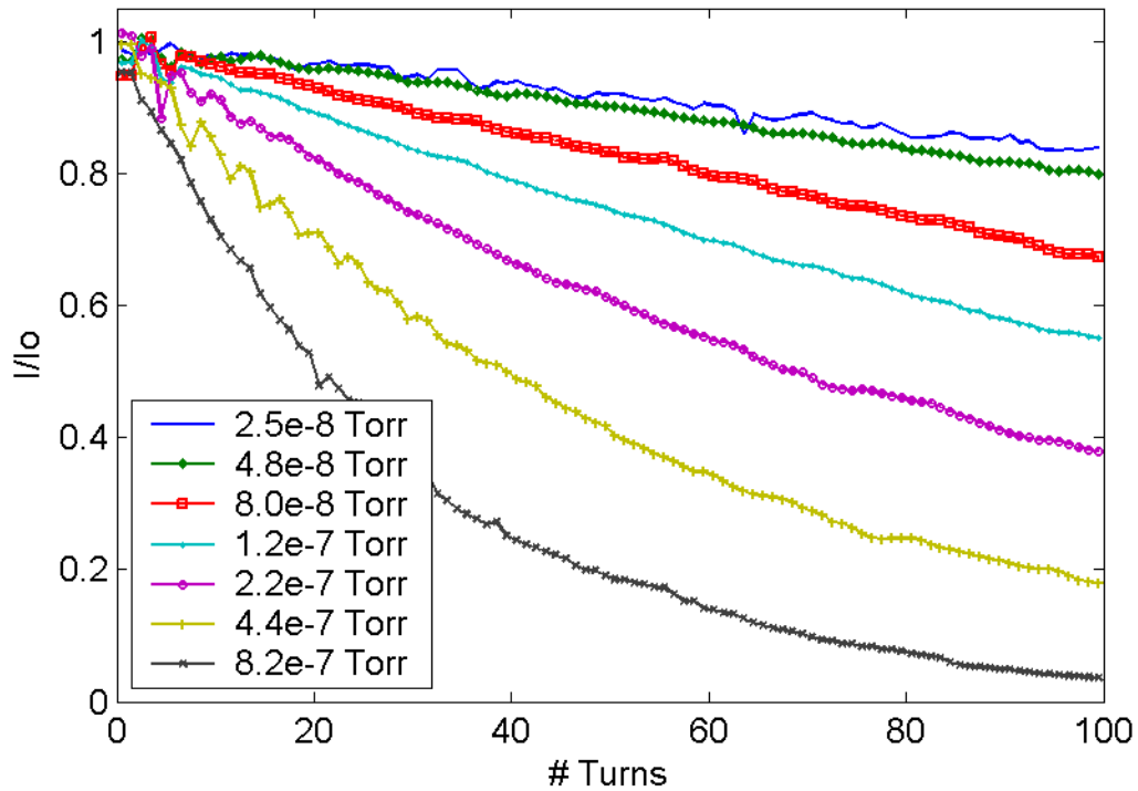
Figure 55: Normalized beam current versus turn number for different gas pressures. (21 keV H_2^+ )
