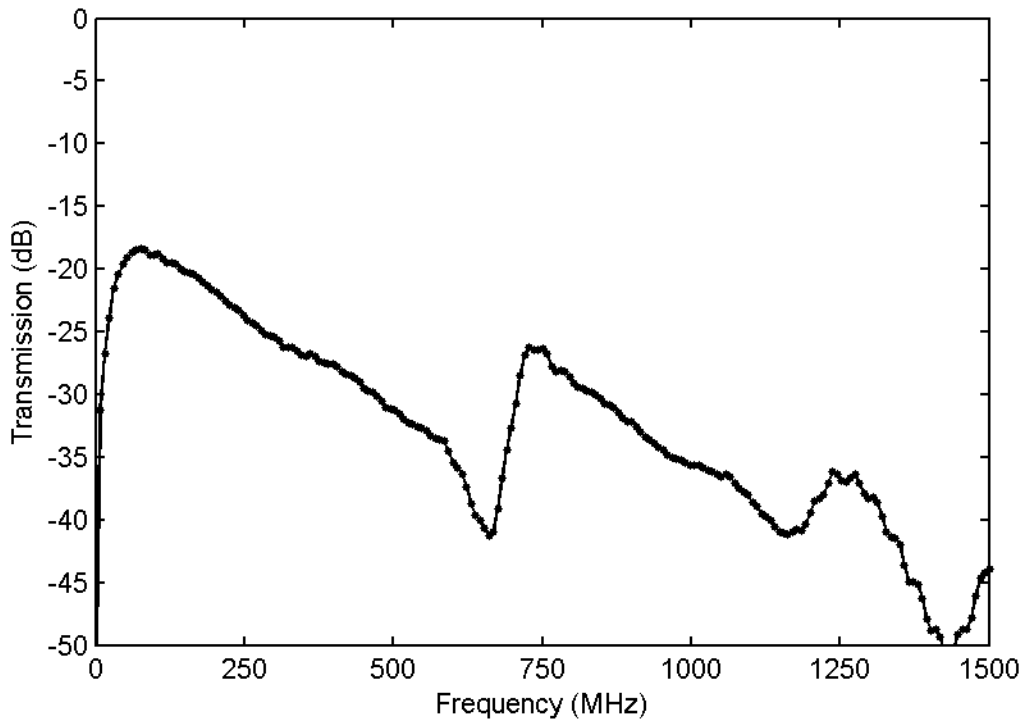
Figure 29: Measurement of the cross talk between central electrodes of the sector fast Faraday cup. The amplitude of the induced signal in one the central electrodes was measured when a signal was sent to the electrode next to it.
