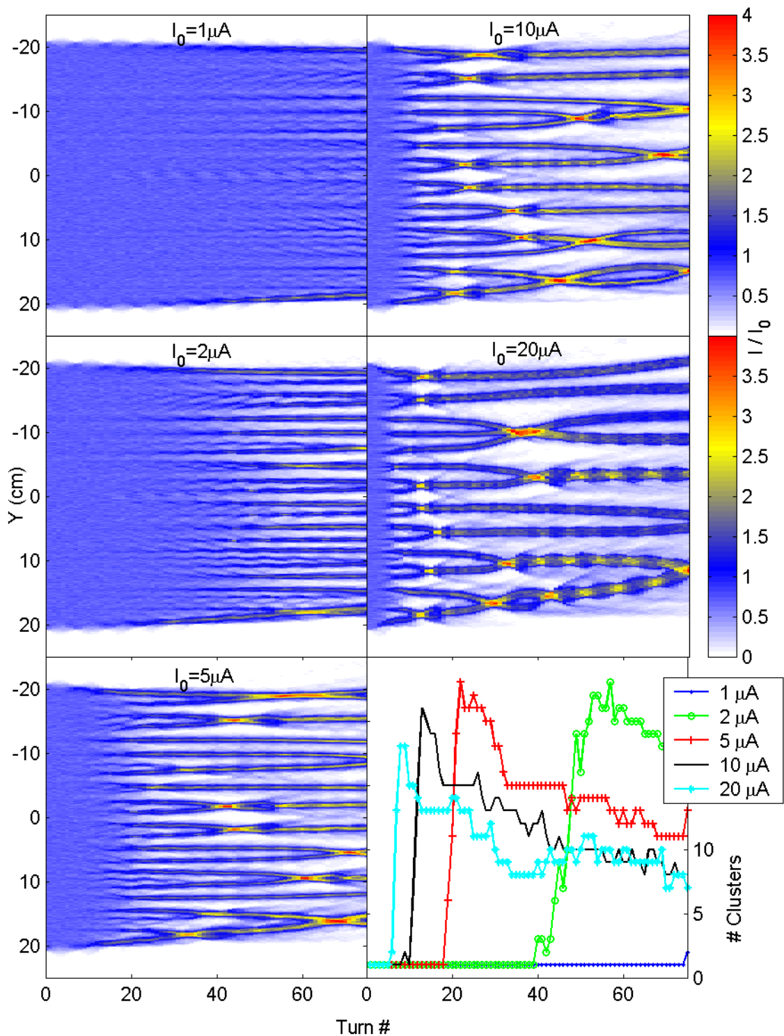
Figure 72: Waterfall diagrams representing the evolution of the longitudinal bunch profile for 1, 2, 5, 10 and 20 \mu\text{A} peak currents. The other parameters that characterize the bunch are listed in Table 9. The number of clusters counted is shown in the lower right corner of the figure.
