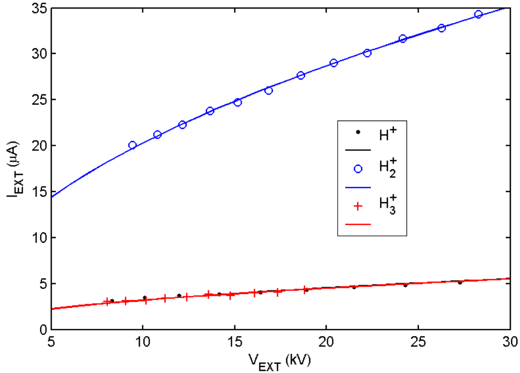
Figure 50: Extraction current versus extraction voltage for different ion masses. The conditions in the source are enumerated in Table 4.
