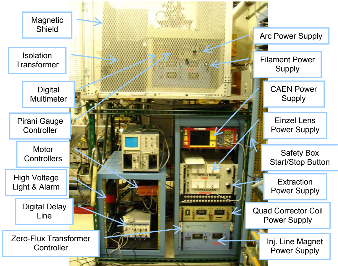
Figure 96: Picture of the ion source and injection line associated electronics.
