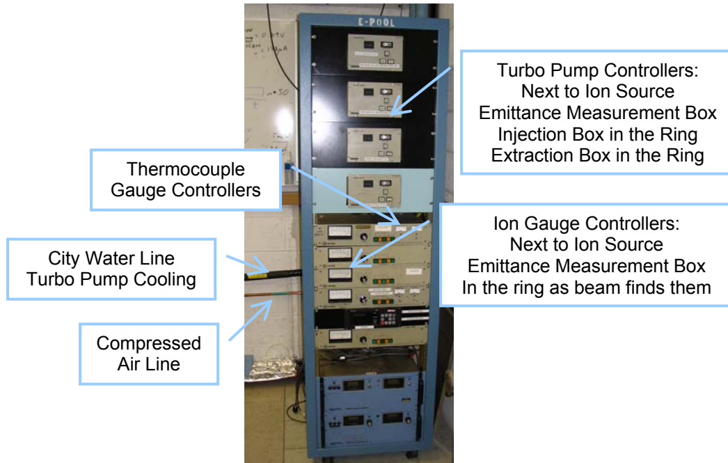
Figure 105: Picture of the vacuum system control area.
