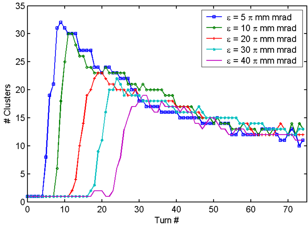
Figure 80: Number of clusters as a function of the turn number for different beam emittances.
