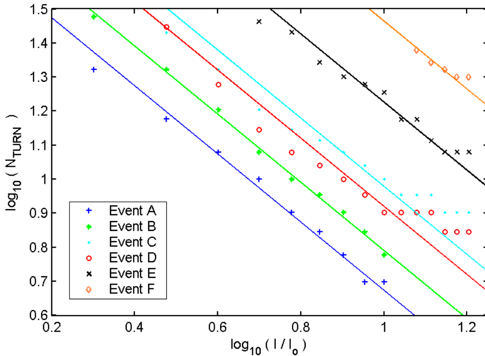
Figure 71: Turn number when the events labeled A thru F in Figure 69 and Figure 70 occur for different peak currents.
