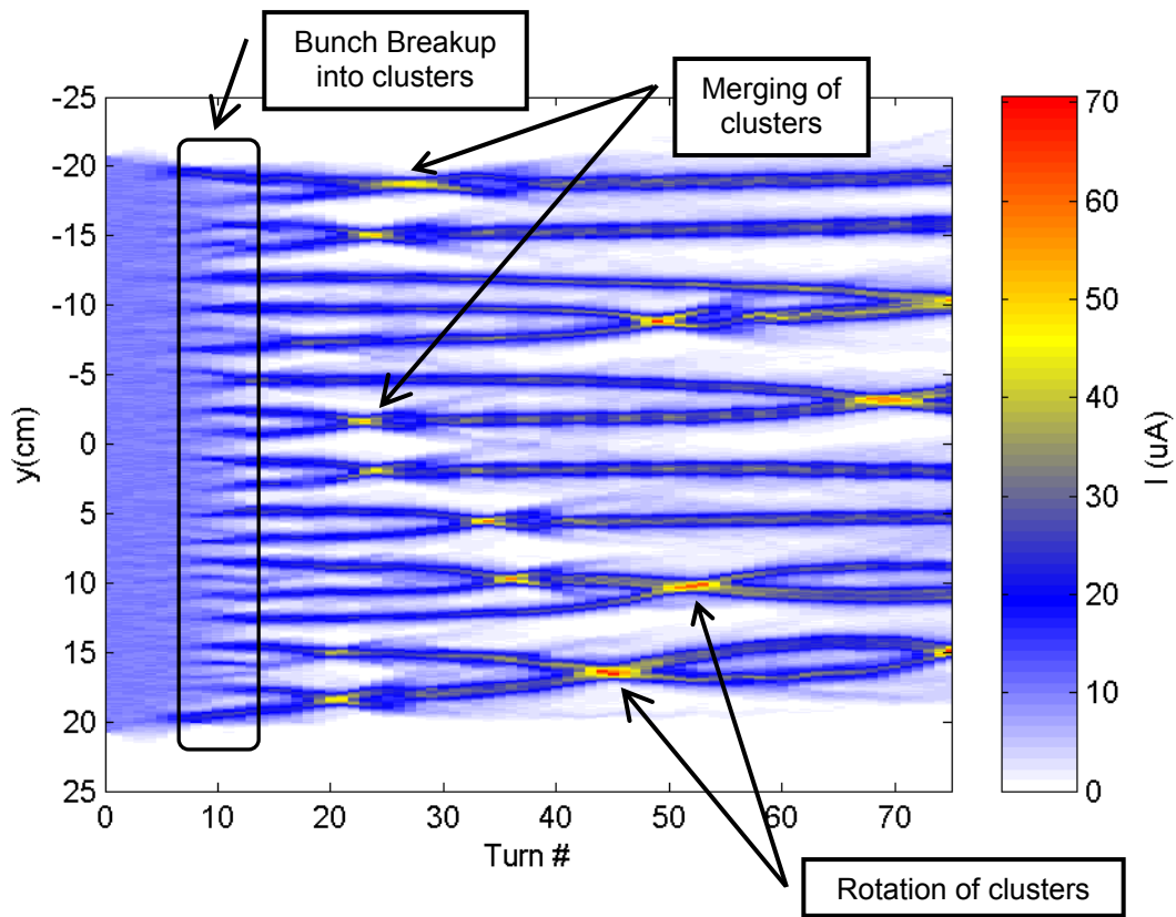
Figure 58: Example of waterfall diagram for a 300 ns long H_2^+ bunch with energy 20 keV, peak current 10 \mu A and emittance 30 \pi mm mrad. The longitudinal bunch profile is plotted after a variable of turns.
