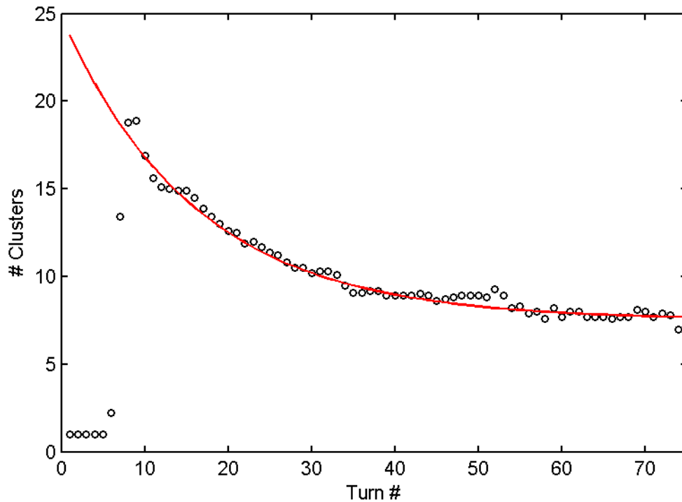
Figure 85: In black circles: number of clusters (averaged over ten initial representations) formed for a 20 \mu\text{A} peak current (rest of bunch characteristics are listed in Table 9). The data was fitted to an offset decaying exponential (solid red line).
