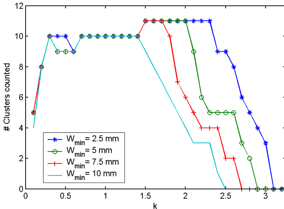
Figure 60: Number of clusters counted in longitudinal profile in Figure 59 for different values of the user defined parameters k and W_{\min} .
