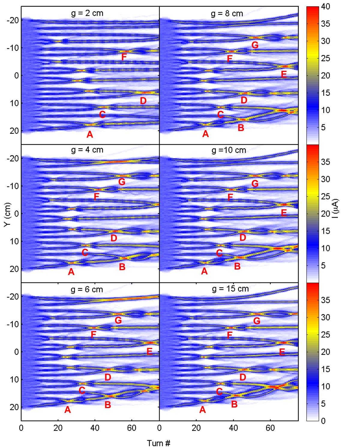
Figure 77: Waterfall diagrams representing the evolution of the longitudinal bunch profile for sizes of the vacuum chamber ranging from 2 cm to 15 cm. The parameters that characterize the bunch are listed in Table 13.
