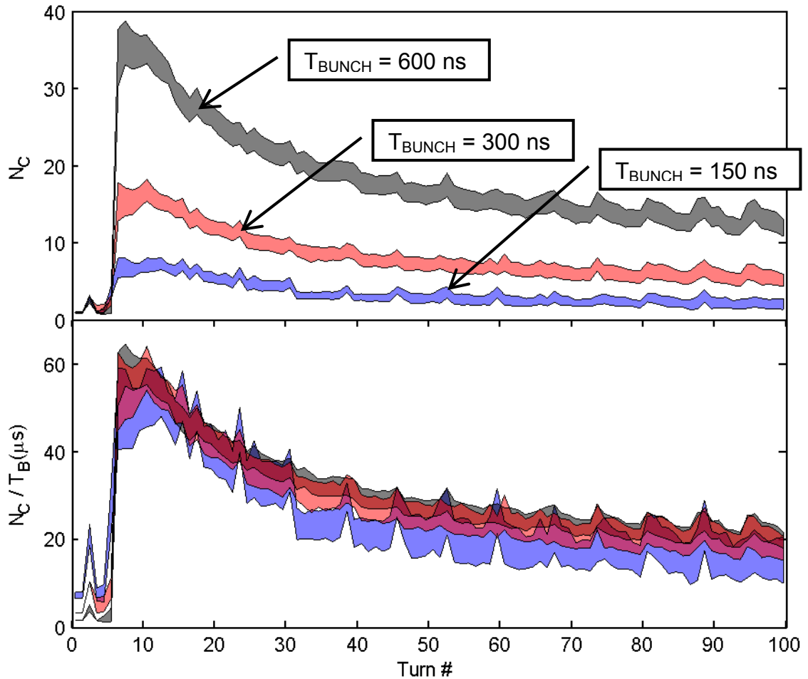
Figure 88: Experimental verification of the scaling law with the bunch length. The number of clusters counted for bunches with characteristics listed in Table 20 scales with the length of the bunches as it can be seen in the bottom of the figure where the density of clusters is plotted.
