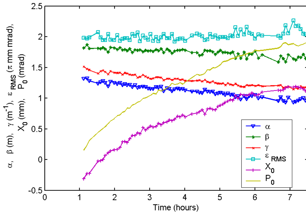
Figure 49: Y-Y' phase space characteristics over a 6 ½ hours period of time 1 hour after turning on the machine. The injection line was set up to be able to inject a 20 keV H_2^+ beam in the ring.
