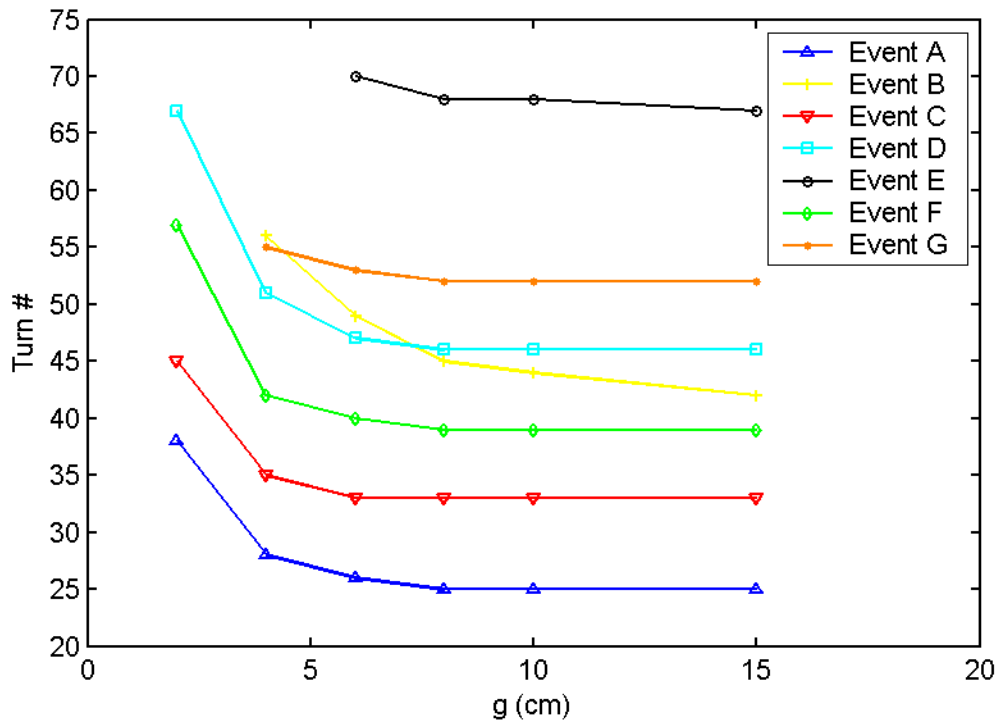
Figure 78: Turn number when the events labeled A thru G in Figure 77 occur when the size of the vacuum chamber is changed.
