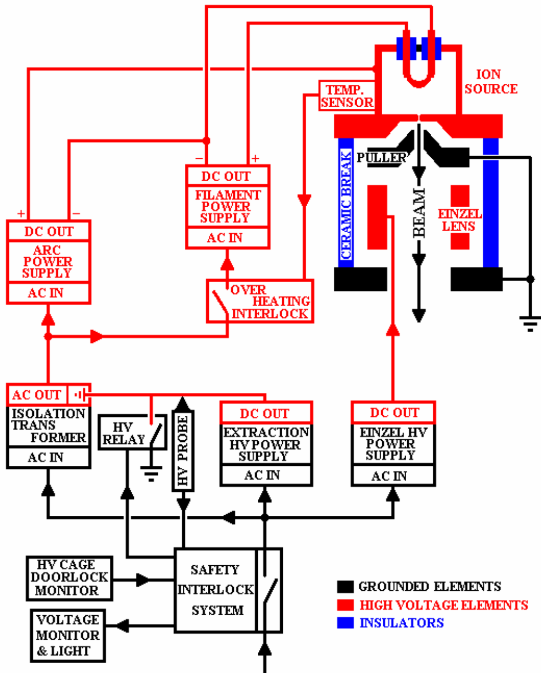
Figure 5: Wiring diagram of the ion source and its associated electronics.
