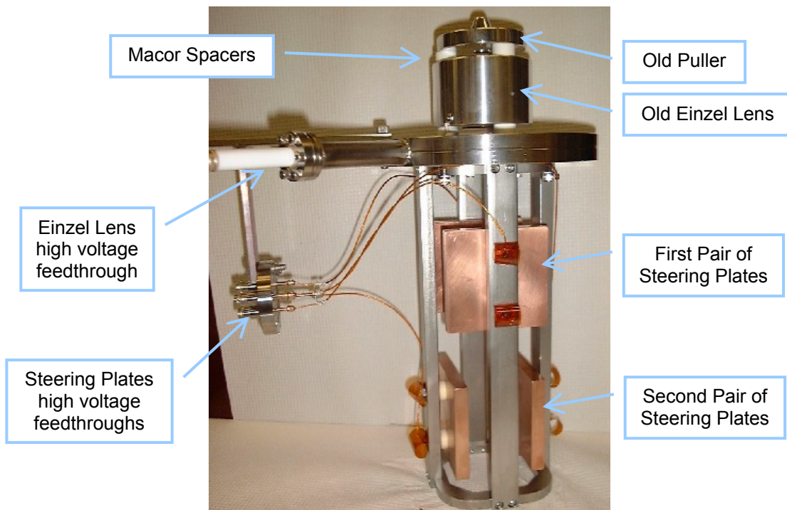
Figure 9: Picture of the first two pairs of steering plates in the injection line of SIR. An old version of the Einzel lens and puller can be seen in top of the 8" flange that supports the whole structure.
