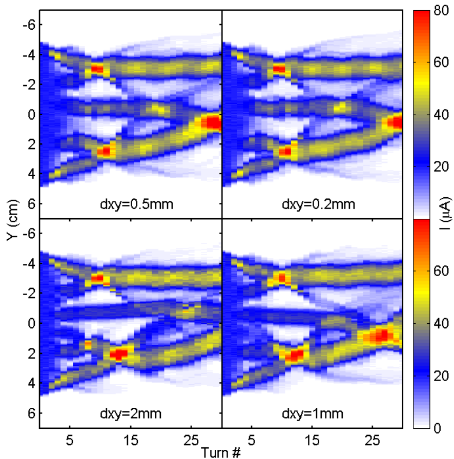
Figure 64: Evolution of the longitudinal profile of a bunch with characteristics listed in Table 7 for different values of dxy (grid size in the FFT algorithm used to calculate the space charge electric field in the x-y plane (parallel to the medium plane of the ring)). The value of N_{xy} is 2^{16} in all cases.
