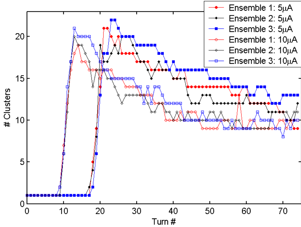
Figure 66: Number of clusters versus turn number for three different initial ensembles representing bunches with two different peak currents. The rest of the bunch characteristics are listed in Table 8.
