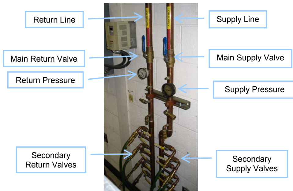
Figure 92: Picture of the low conductivity water manifold used to cool down the ion source, the emittance measurement system and the dipole coils.
