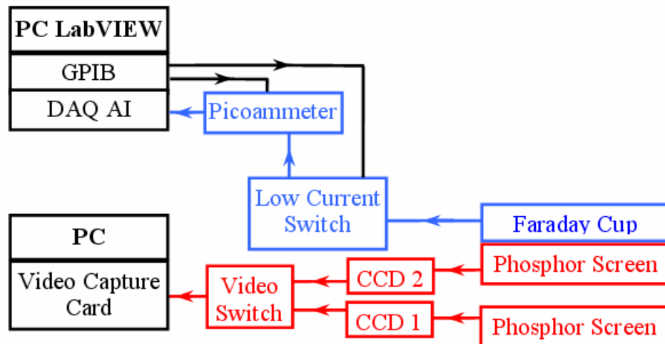
Figure 44: Layout of the phosphor screens and their associated control electronics.
