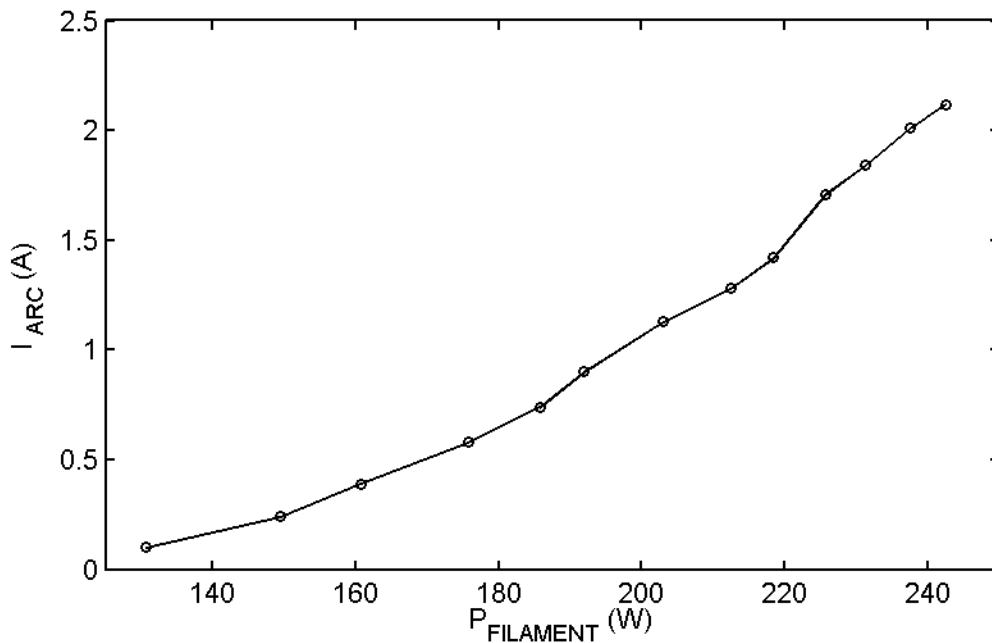
Figure 52: Relationship between arc current and filament power measured for constant value of the arc voltage, extraction voltage and gas pressure. (Values are listed in Table 5.)
