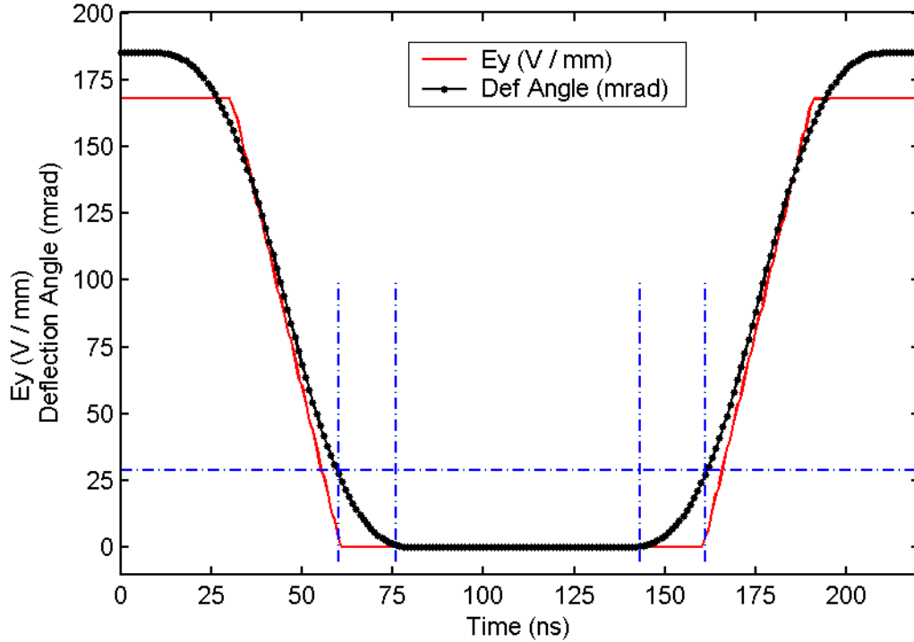
Figure 18: The deflection angle of a 20 keV H_2^+ beam as it goes through the chopper is plotted in black. The value of the electric field in the center of the chopper at the time the ions get there is plotted in red.
