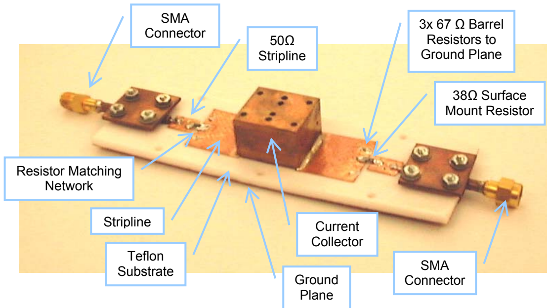
Figure 32: Picture of the back of the prototype stripline fast Faraday cup developed for SIR.
