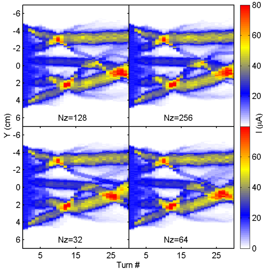
Figure 62: Evolution of the longitudinal profile of a bunch with characteristics listed in Table 7 for different values of Nz (Number of grid points in the FFT algorithm used to calculate the space charge electric field in the z direction (perpendicular to the medium plane of the ring)).
