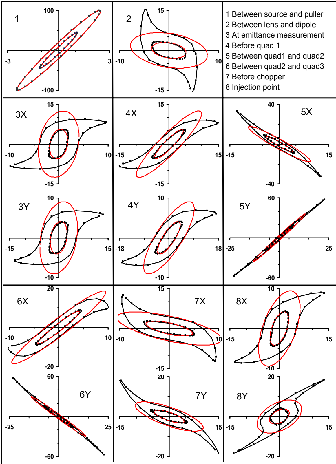
Figure 25: Snap-shots of the phase space of the beam in the injection line. Ellipses using COSY model in red. (Black in the 3D fields). Inner (outer) ellipses 10 (50) \pi mm mrad.
