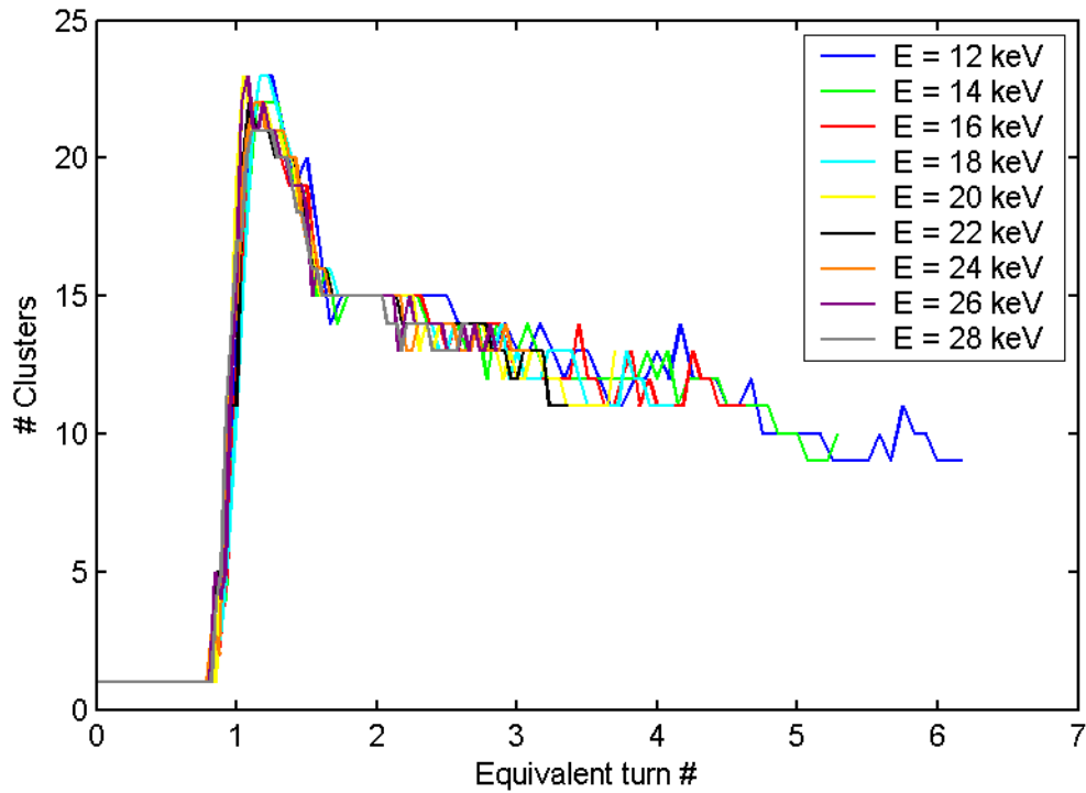
Figure 74: Number of clusters as a function of the equivalent turn number for different energies.
