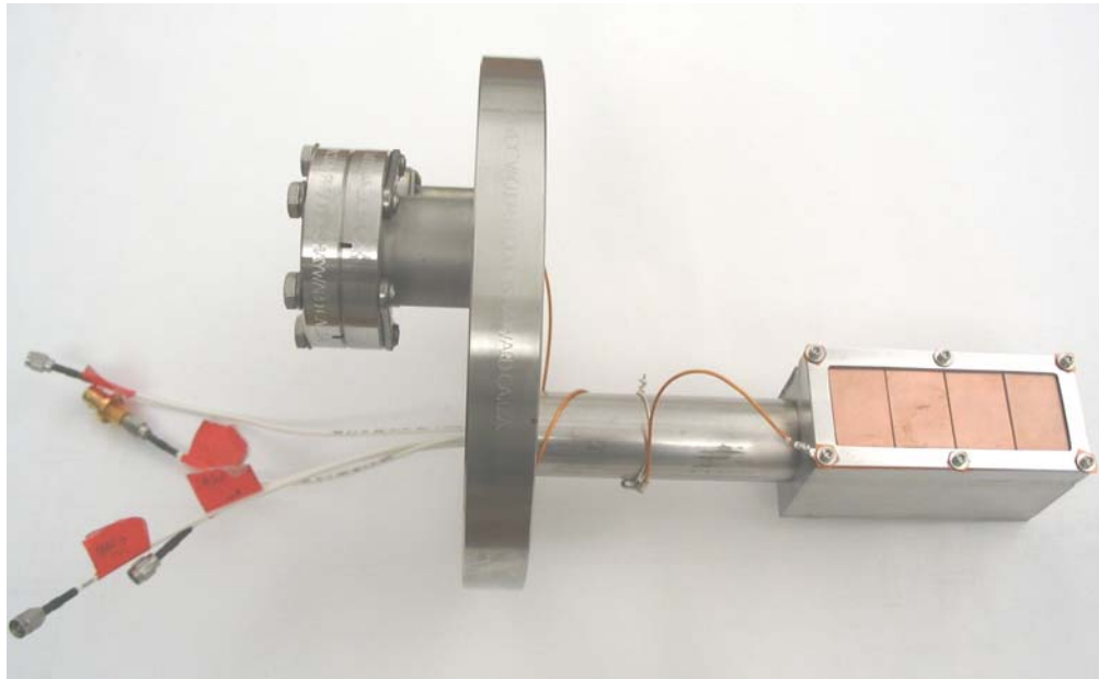
Figure 27: Picture of the sector fast Faraday cup used to measure beam longitudinal profiles when they are extracted from the ring.
