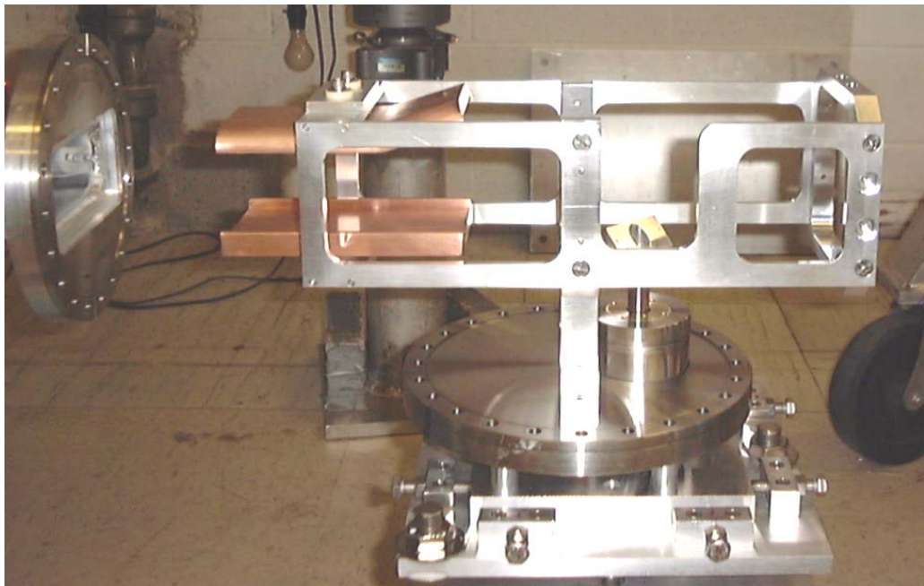
Figure 20: Picture of the second pair of inflector plates located in between two of the dipole magnets of the ring.
