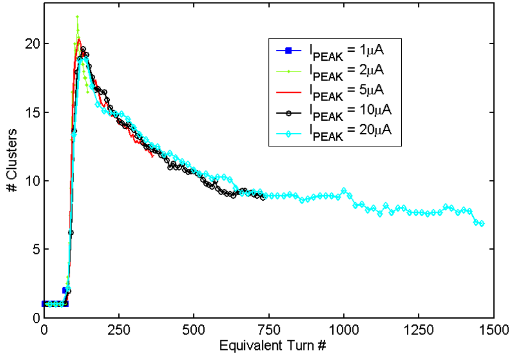
Figure 73: Number of clusters as a function of the equivalent turn number ( N_{EQ} ) for different peak currents.
