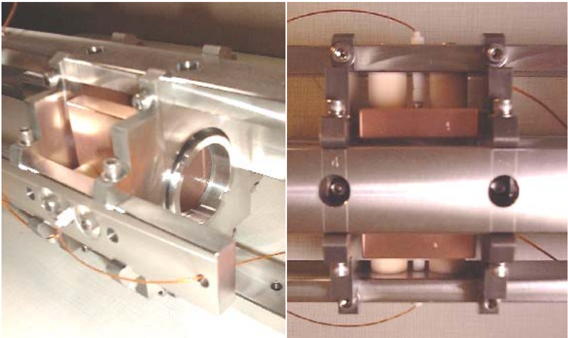
Figure 16: Pictures of the system used to chop the beam in the injection line of SIR.
