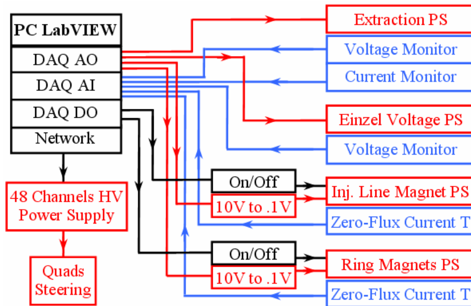
Figure 42: Layout of some of the power supplies used in SIR and their associated control electronics.
