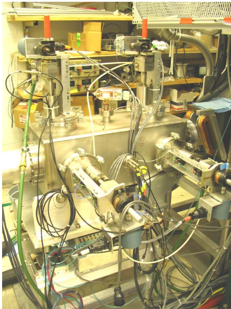
Figure 12: Picture of the emittance measurement system used to transversely characterize the beam coming from the ion source.
