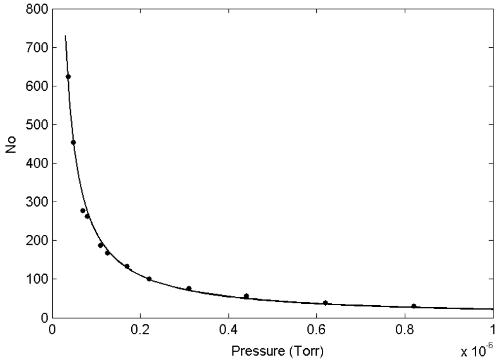
Figure 56: N_o as a function of the pressure in the ring for a 21 keV H_2^+ beam.
