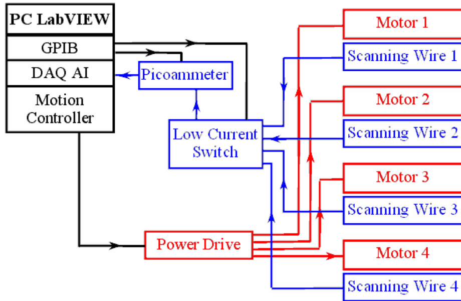
Figure 33: Layout of the scanning wires and their associated control electronics.
