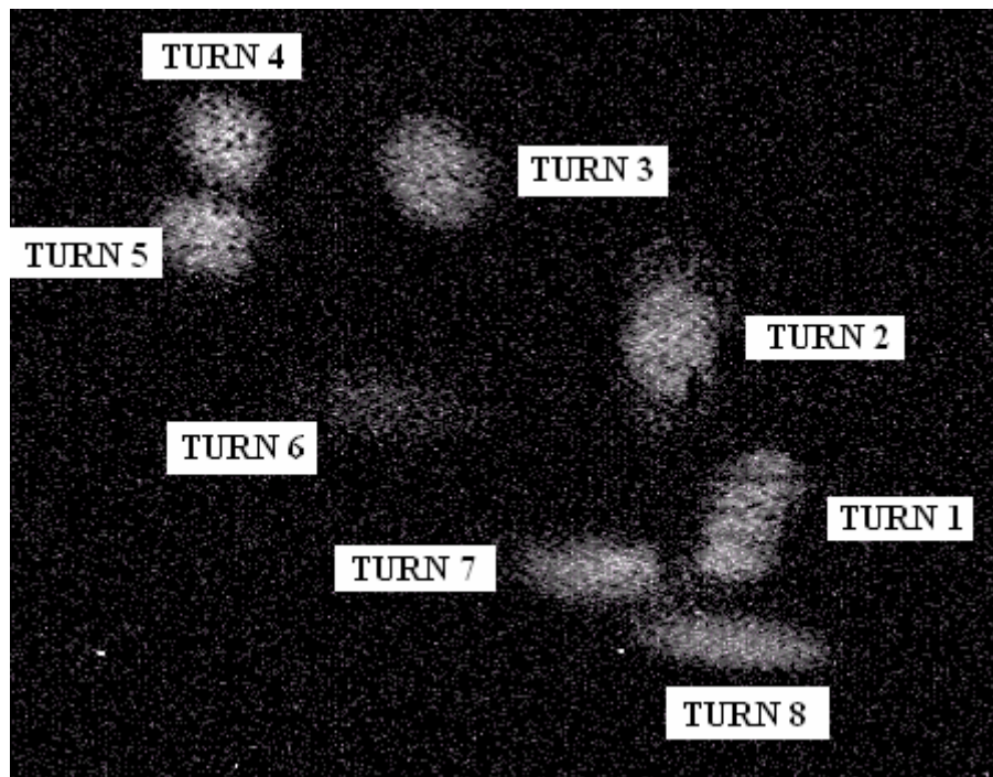
Figure 38: Superposition of pictures of extracted beam as seen in the phosphor screen before matching is performed.
