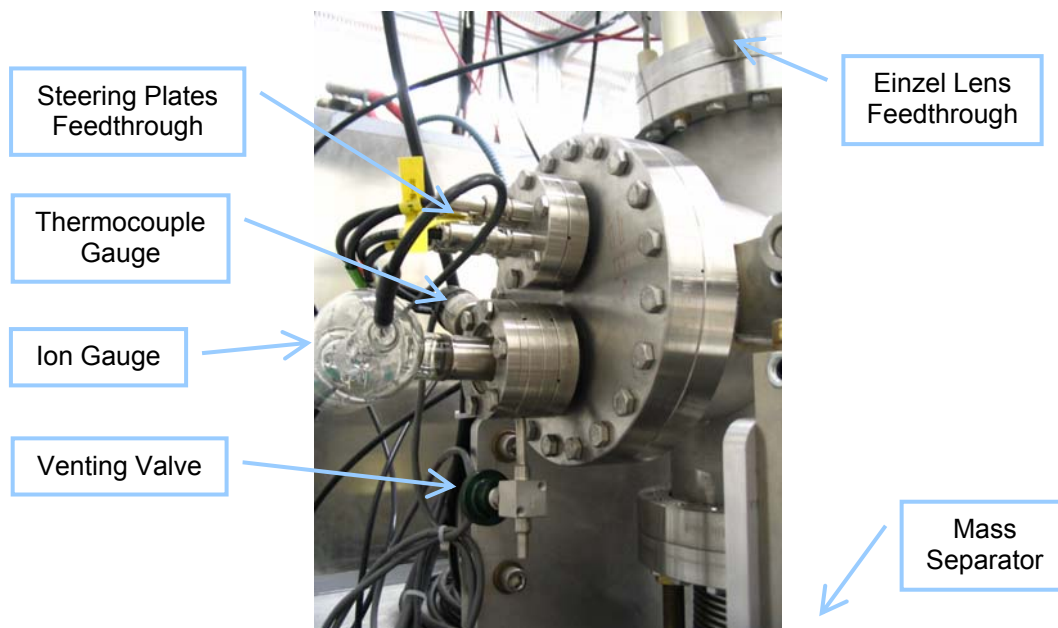
Figure 106: Picture of the venting valve and one of the thermocouple gauges used in the injection line of SIR.
