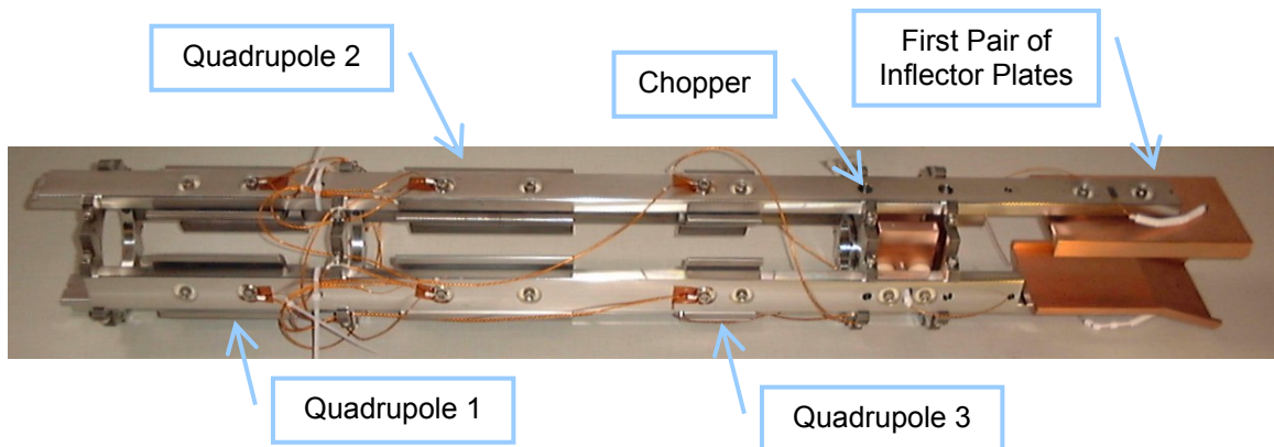
Figure 13: Picture of the quadrupole triplet, chopper and first pair of inflector plates held by a support frame before being assembled in the injection line of SIR.
