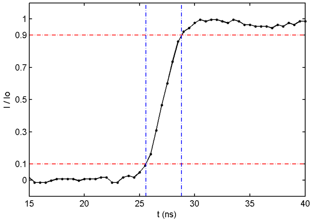
Figure 28: Measured rise time of the signal in one of the sectors of the fast faraday cup when a bunch hits it.
