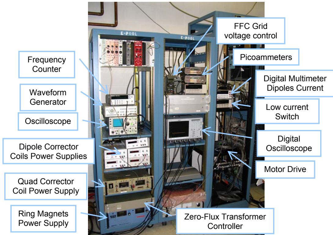
Figure 98: Picture of the ring and extraction line associated electronics.
