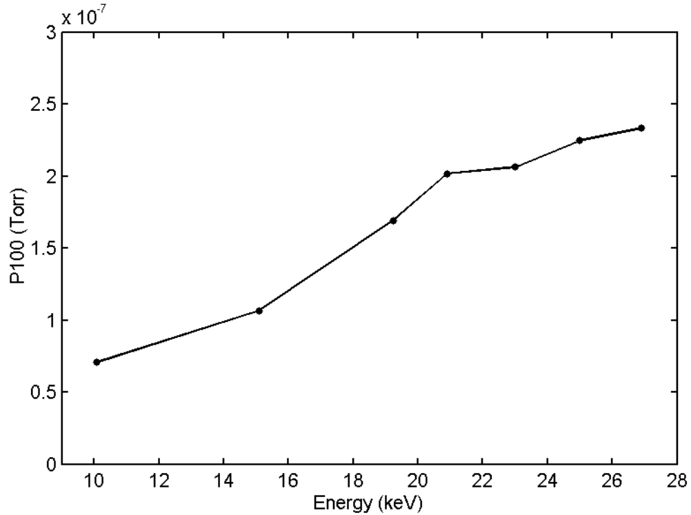
Figure 57: P_{100} as a function of the beam energy.
