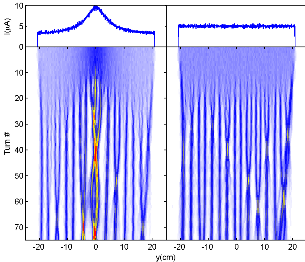
Figure 81: Waterfall diagrams representing the evolution of the longitudinal bunch profile for two bunches with different initial longitudinal profile (top left and right). The initial microscopic representation of the bunch in the left was generated by displacing macroparticles toward the center of the bunch. The parameters that characterize the bunch are listed in Table 15.
