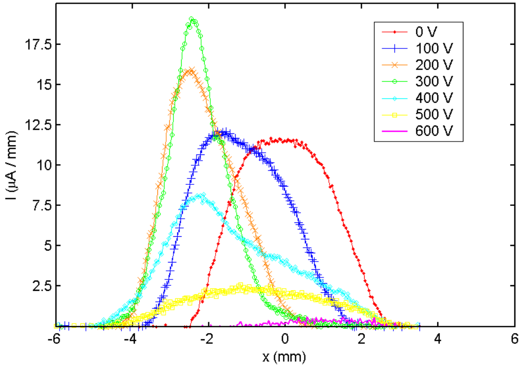
Figure 17: Transverse beam profiles measured with the first horizontal scanning wire for different voltages in the chopper. When the plates are biased to more than \pm 600V , the beam is deflected and is not injected.
