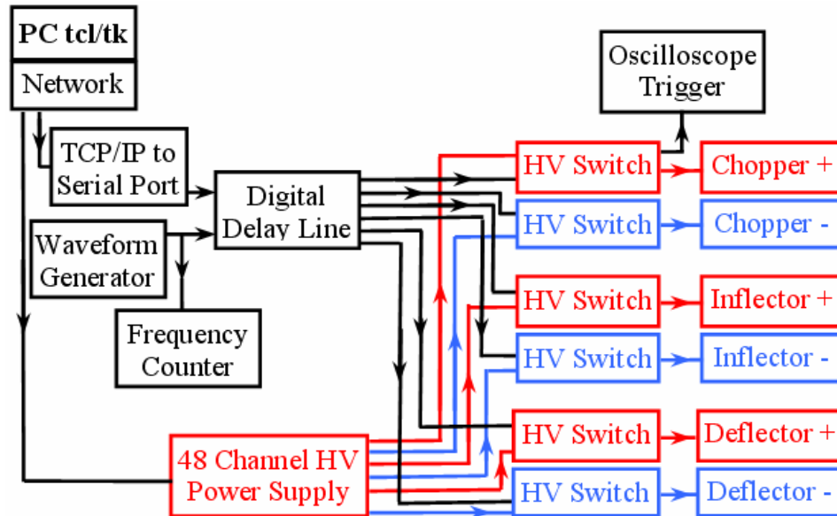
Figure 37: Layout of the chopper, inflector and deflector and their associated control electronics.
