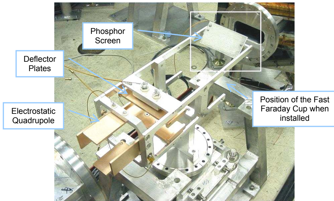
Figure 26: Picture of the extraction box of SIR during assembly.
