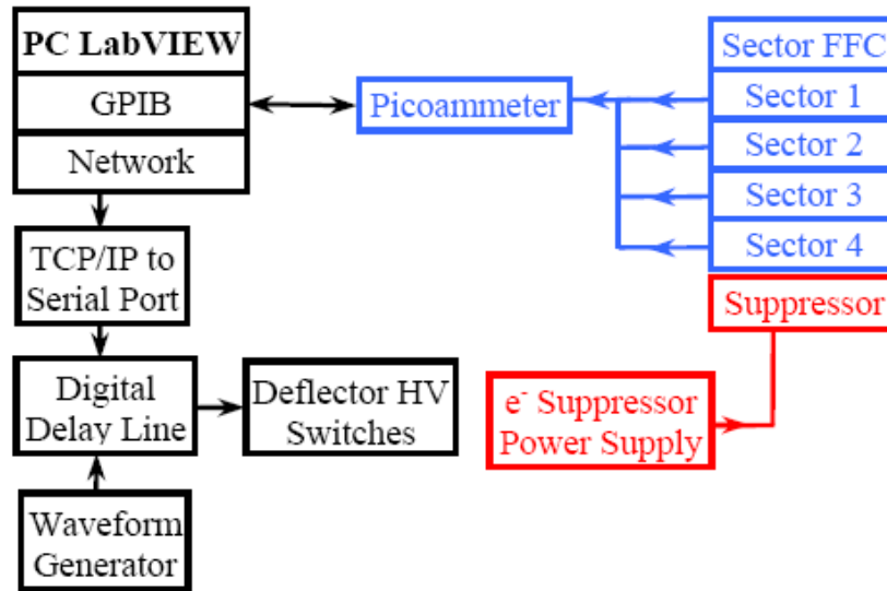
Figure 45: Layout of the beam lifetime measurement electronics and their control electronics.
