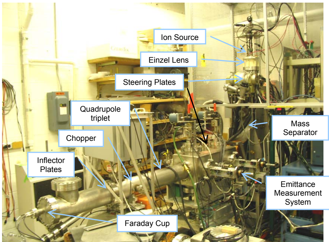
Figure 4: Picture of the injection line of SIR.
