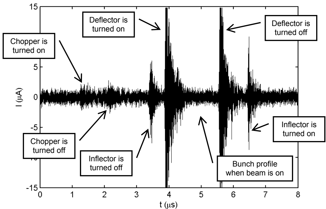
Figure 30: Noise induced in one of the electrodes of the sector Faraday cup when the chopper, inflector and deflector plates are turned on and off.
