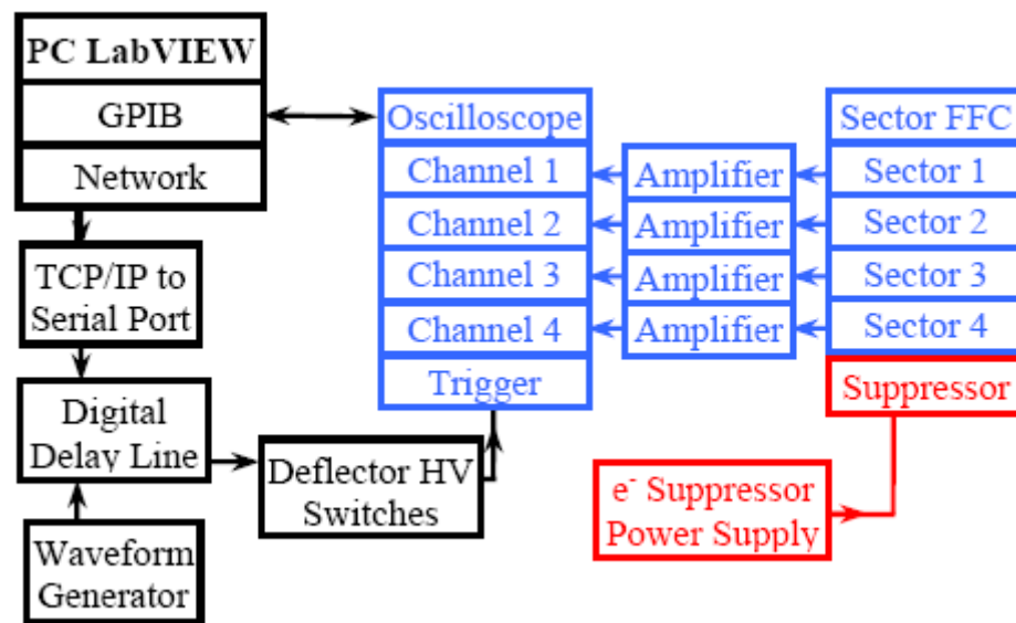
Figure 40: Layout of the sector fast faraday cup and its associated electronics.
