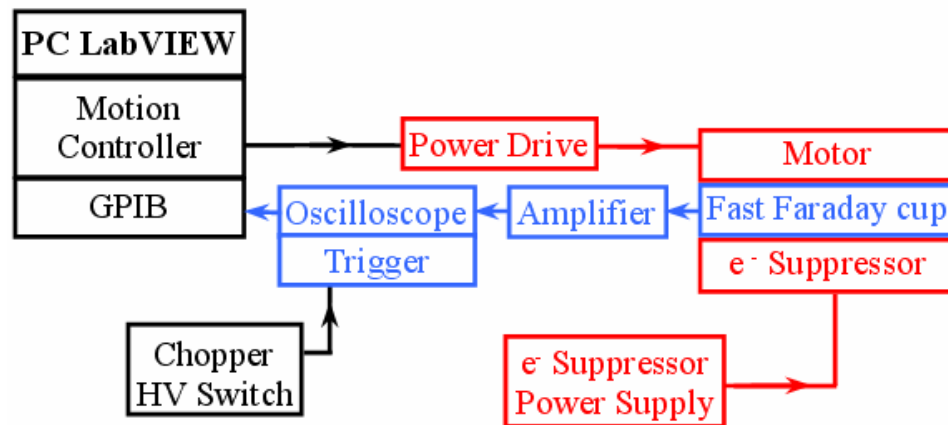
Figure 39: Layout of the fast faraday cup and its associated control electronics.
