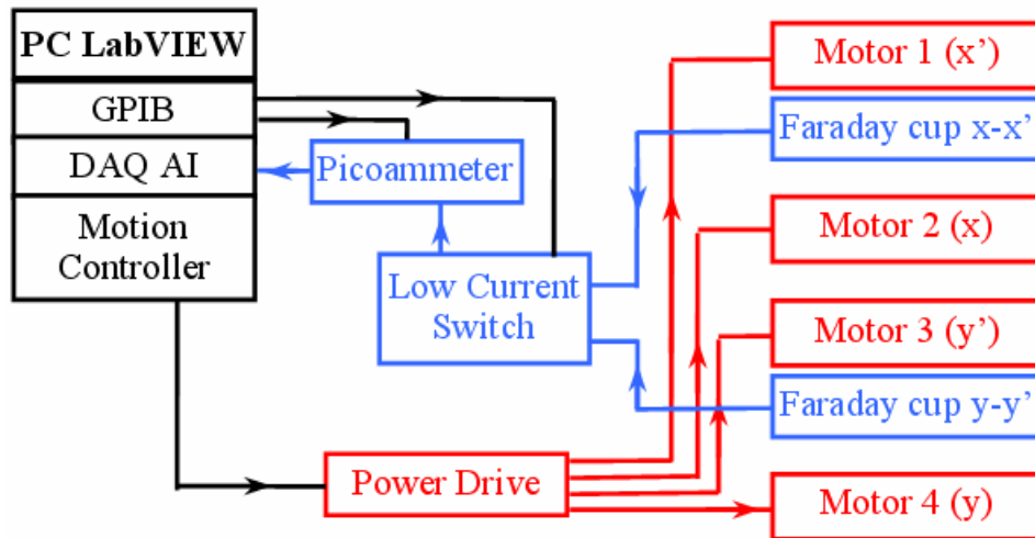
Figure 35: Layout of the emittance measurement system and its associated control electronics.
