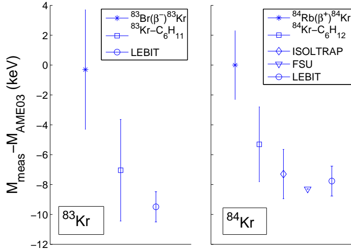
Fig. 7. Deviation of individual mass measurements of ^{83,84}\text{Kr} from AME03. Values obtained from \beta decays use AME03 values for the masses of the parent nuclei.
