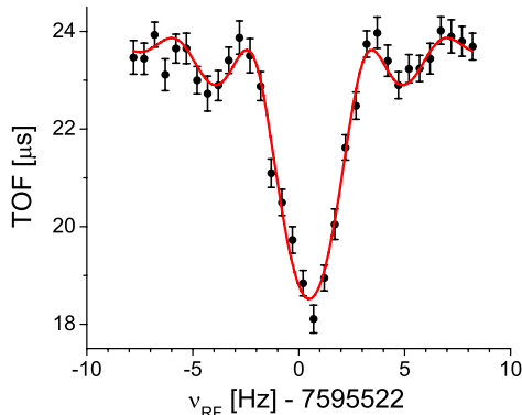
Fig. 8. ^{38}\text{Ca}^{2+} cyclotron resonance taken with 300 ms RF excitation. The observed linewidth corresponds to a resolving power of R \approx 2,000,000
