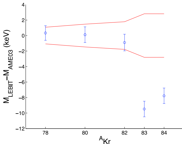
Fig. 6. The difference between mass values measured with LEBIT and AME03 [23] for the stable krypton isotopes. The error band corresponds to the uncertainty of the literature values, the error bars to the uncertainty of the mass values determined with LEBIT.
