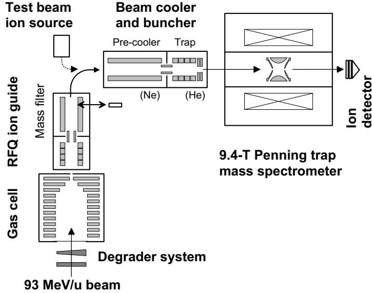
Fig. 1. Layout of the LEBIT facility at the NSCL/MSU.
