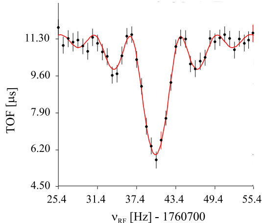
Fig. 5. Cyclotron resonance curve of ^{82}\text{Kr}^+ ions with a fit of the theoretical line shape. An excitation time of 200 ms was used in this measurement.
