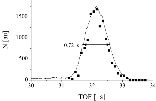
Fig. 2. Time-of-flight distribution of ions accumulated in the buncher and extracted as pulses measured with an MCP detector. The experimental result (solid curve) is compared with that of corresponding simulations (square dots). The latter is corrected for a 0.4 \mu\text{s} electronic time delay.
