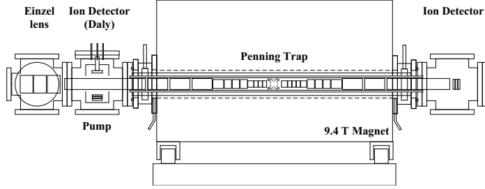
Fig. 3. Schematic layout of the LEBIT Penning trap system. Ions enter from the left.
