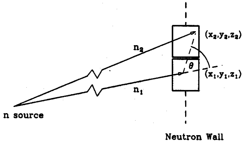
Fig. 6. Side view of two neutrons detected in neighboring cells. Because it is impossible to determine the exact positions where the neutrons scattered, \theta can vary from almost 0^\circ to 180^\circ .
