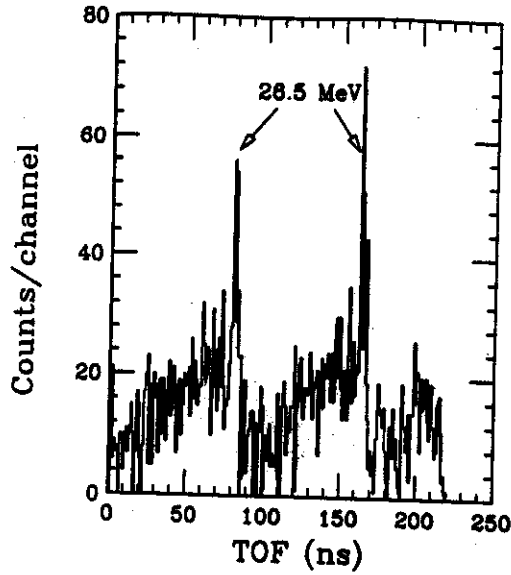
Fig. 9. Time-of-flight spectrum for neutrons detected in cell #7 in the {}^7\text{Li}(p,n) experiment. The signal of cell #7 gave the start and the downscaled cyclotron radio frequency signal gave the stop. The sharp peaks are from neutrons produced in the reactions leading to either the ground state or the first excited state of {}^7\text{Be} .
