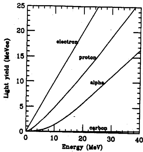
Fig. 3. The light response for electrons, protons, alphas, and carbon nuclei in liquid scintillator. 1-MeVee is equal to the light produced by a 1-MeV electron. The data are from Verbinski et al. [8]
