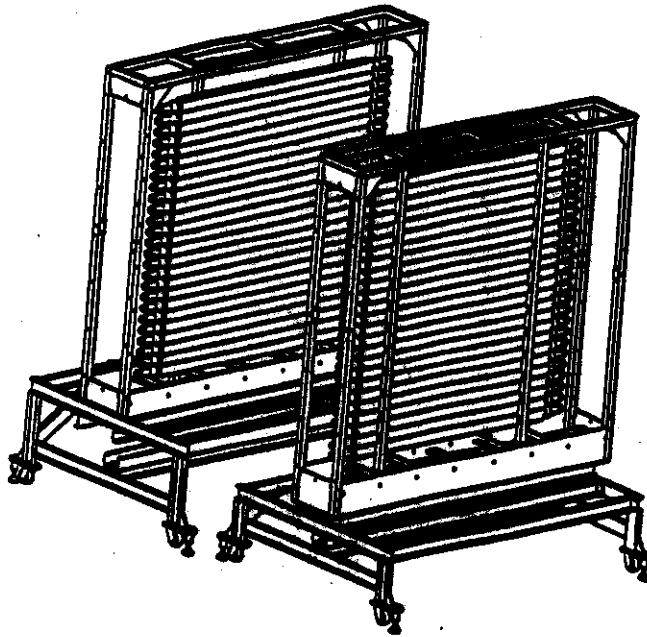
Fig. 1. Picture of the neutron walls without their aluminum covers. Each wall consists of 25 rectangular cells filled with NE-213 liquid scintillator. Each cell, with photomultipliers at the ends, has a dimension of 7.62 \times 6.35 \times 200 cm 3 . The walls are movable so that they can be set at the desired positions.
