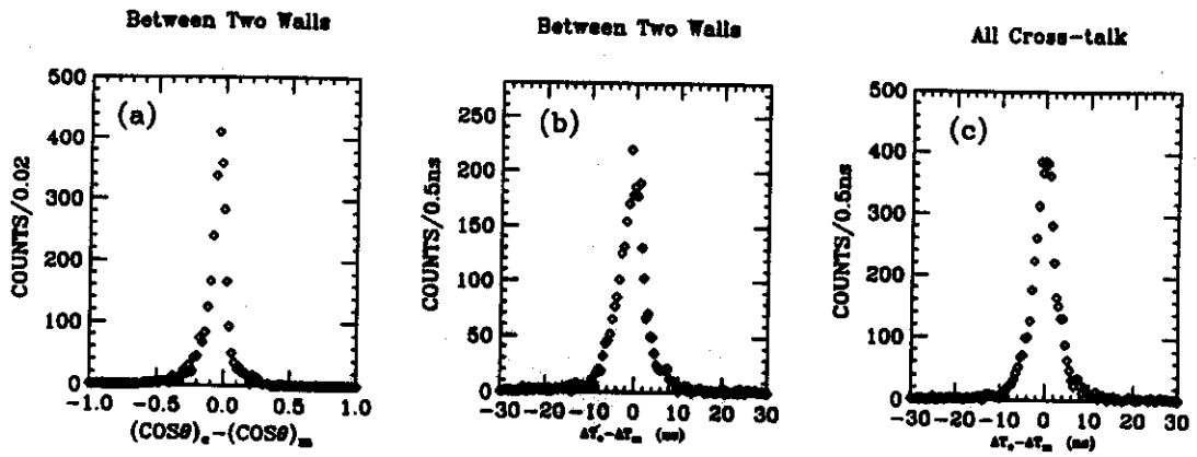
Fig. 11. Cross-talk distributions for all the neutrons from the {}^7\text{Li}(p,n) experiment---those from the 2-body reaction (eq. 8) and those from the 3-body reaction (eq. 9). (a) (\text{COS}\theta)_e - (\text{COS}\theta)_m distribution for the cross-talk events between the two walls. (b) \Delta T_e - \Delta T_m distribution for the same events in (a). (c) \Delta T_e - \Delta T_m distribution for all the cross-talk events.
