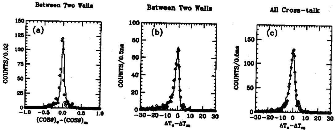
Fig. 10. Cross-talk distributions for the neutrons under the sharp peaks in Fig. 9 from the {}^7\text{Li}(p,n) experiment. The experimental data are given by open symbols. The histograms are the results of our simulation. (a) (\text{COS}\theta)_e - (\text{COS}\theta)_m distribution for the cross-talk events between the two walls. (b) \Delta T_e - \Delta T_m distribution for the same events in (a). (c) \Delta T_e - \Delta T_m distribution for all the cross-talk events
