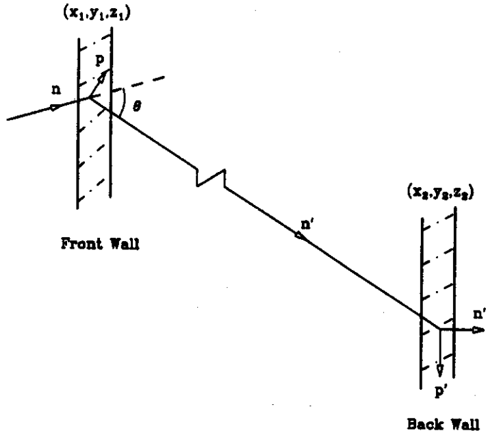
Fig. 4. An example of cross-talk between the front wall and the back wall. The neutron makes one signal in a cell of the front wall and another one in a cell of the back wall. The position of each scattering is expressed by (x,y,z) . The scattering in the front wall follows the two-body kinematics given by eqs. 1 and 2 in text
