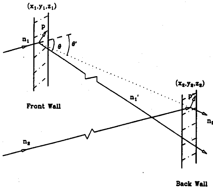
Fig. 5. An example of a real 2-n events between the front wall and the back wall. If we assume this is a cross-talk event, \theta should be the neutron's scattering angle according to 2-body kinematics. However, the positions of the two scatterings give \theta' . Unlike cross-talk events, the two angles are not correlated for real 2-n events.
