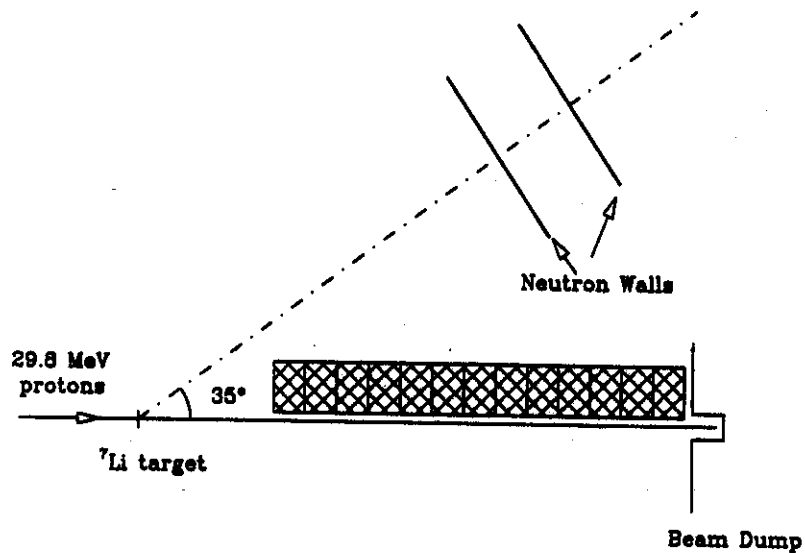
Fig. 8. Layout of the ^7\text{Li}(p,n) experiment. The front wall was placed 5 meters from the target, 35^\circ relative to the beamline. The second wall was 1 meter behind the first one. The shaded area was a stock of concrete blocks
