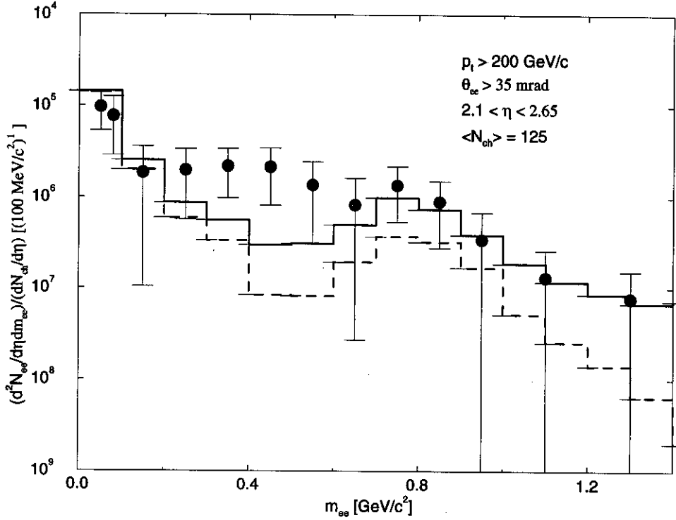
Figure 1: Total dilepton invariant mass distributions: primary meson decays alone (dashed line) and primary meson decays with secondary scattering (solid line) as compared with CERES data for S+Au collisions.
