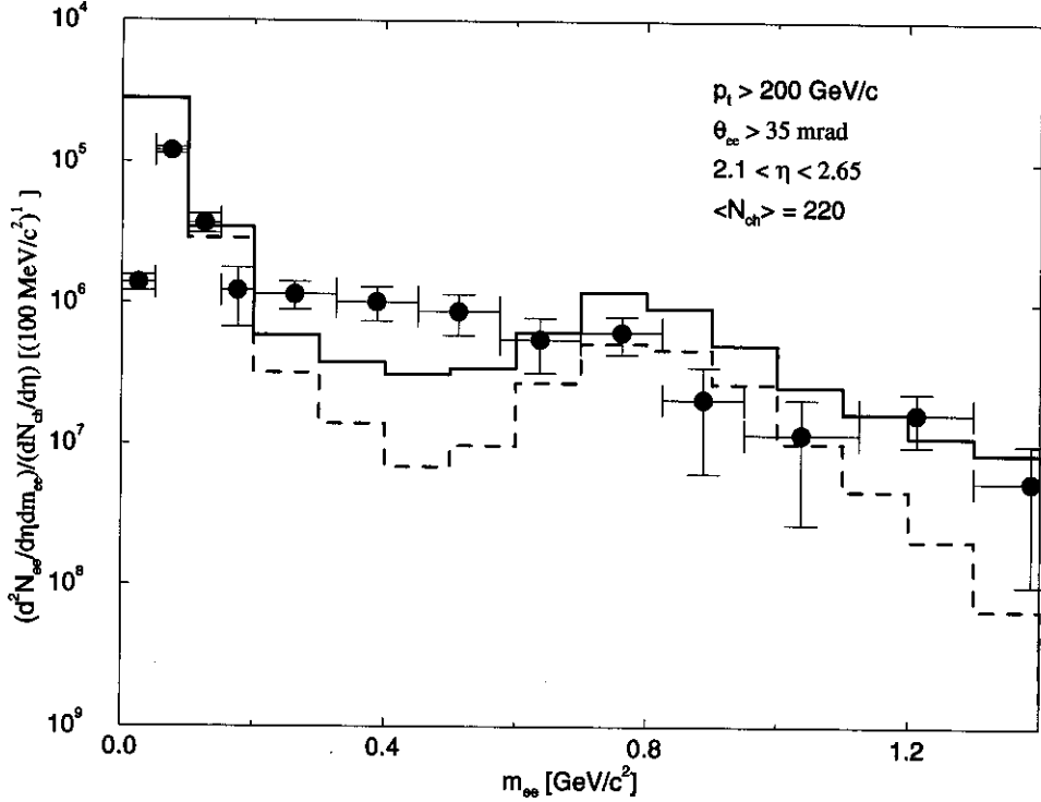
Figure 2: Total dilepton invariant mass distributions: primary meson decays alone (dashed line) and primary meson decays with secondary scattering (solid line) as compared with CERES data for Pb+Au collisions.
