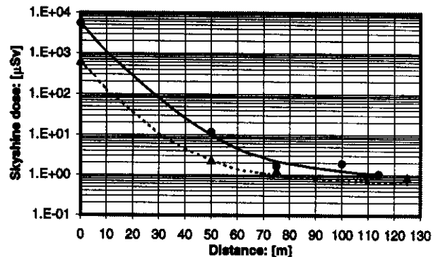
Figure 5: Neutron skyshine dose along the NSCL High bay evaluated with BD 100R bubble dosimeters for 140 MeV/n ^4\text{He} (full line) and 80 MeV/n ^{22}\text{Ne} (broken line) ion irradiation at the K1200 Cyclotron are shown as functions of the distance from the reference point (Figure 1).
