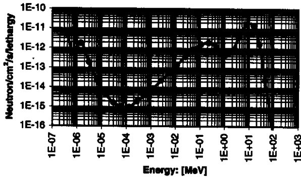
Figure 3: Neutron energy spectrum at the reference point during the bombardment of the aluminium stopping bar with the 140 MeV/nucleon ^4\text{He} ions in the Analysis Hall. The average neutron energy was calculated to be 2.5 MeV.
