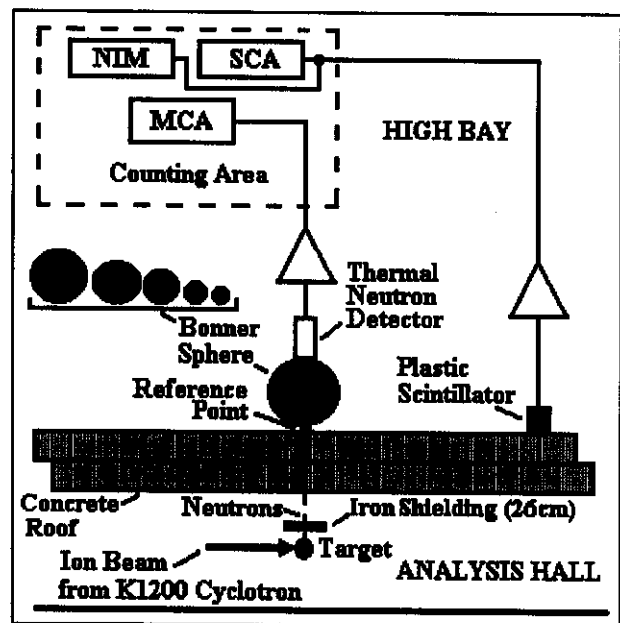
Figure 2: Schematic diagram of the experimental set up at the NSCL High Bay for neutron flux monitoring and spectrometry using a plastic scintillator and a set of polyethylene Bonner spheres respectively.
