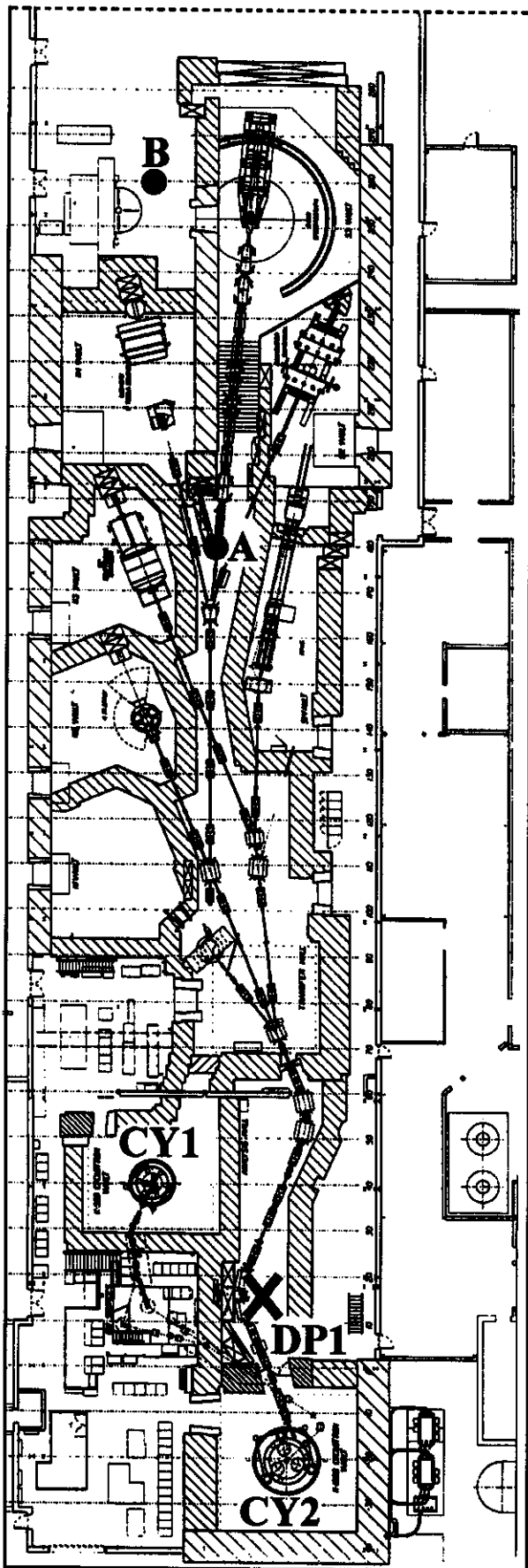
Figure 1: The plan view of the NSCL Facility showing the K500 (CY1) and K1200 (CY2) cyclotrons and associated experimental devices housed in the concrete shielded vaults.
