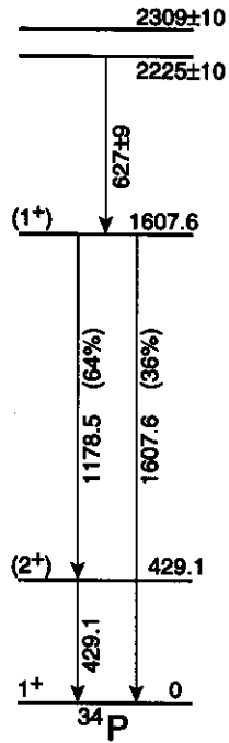
FIG. 2. Level scheme of ^{34}\text{P} relevant to the present study. All four excited states were previously identified in [17]. The excitation energies of the levels below 2 MeV and the branch ratio for the 1607.6 keV state are taken from [16].
