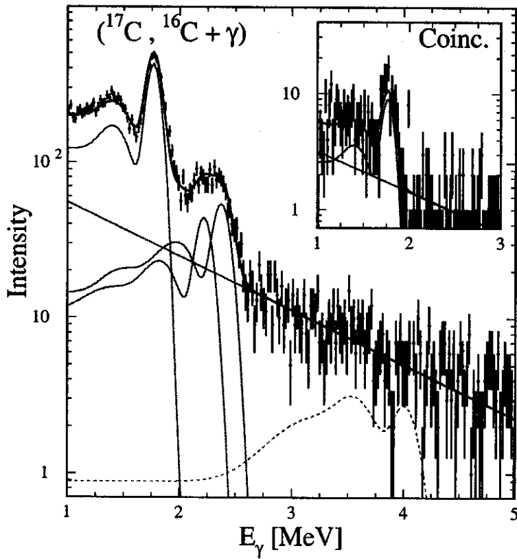
FIG. 4. Doppler-corrected \gamma -ray spectrum measured in {}^9\text{Be}({}^{17}\text{C}, {}^{16}\text{C}+\gamma)\text{X} . The black curve is a fit to the spectrum using an exponential curve for the background and response functions (grey curves) for each of the \gamma -ray transitions shown in the simplified level scheme of Fig. 5. The dashed line corresponds to an estimated upper limit of 2% for the direct transition from the J = 2 level at 3.99 MeV to the ground state. Inset: \gamma spectrum gated on the transitions between the levels at \simeq 4 MeV and the 2^+ level at 1.77 MeV. The spectrum was fitted using the same procedure described above.
