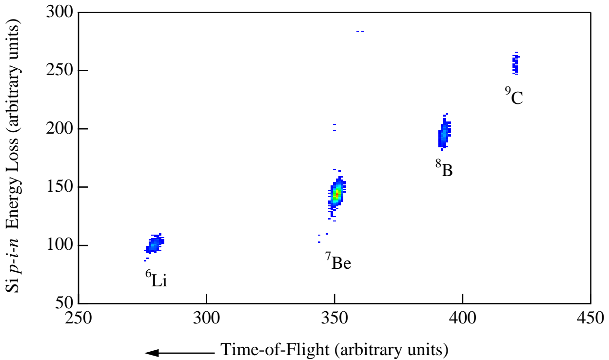
FIG. 2. Typical Si p-i-n diode versus time-of-flight spectrum illustrating the secondary beam composition.
