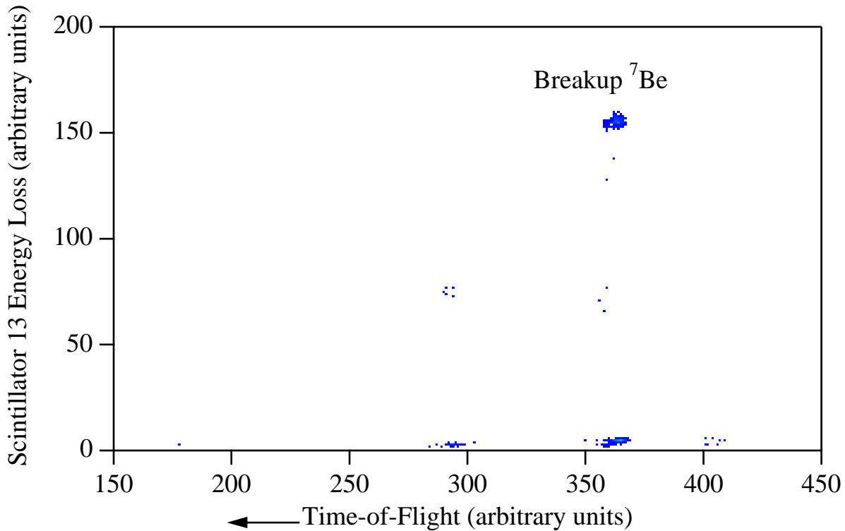
FIG. 6. Typical ^7\text{Be} scintillator bar energy loss versus time-of-flight spectrum. The events with small scintillator signals are due to light produced in adjacent scintillator bars.
