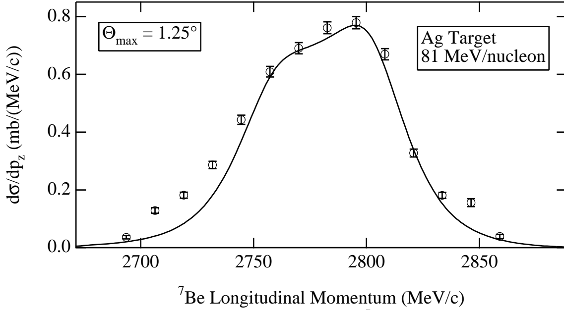
FIG. 11. Laboratory frame longitudinal momentum distribution of ^7\text{Be} fragments with maximum scattering angles of 1.25^\circ emitted in the Coulomb dissociation of 81 MeV/nucleon ^8\text{B} on Ag. The curve is a 1st-order perturbation theory calculation convoluted with the experimental resolution.
