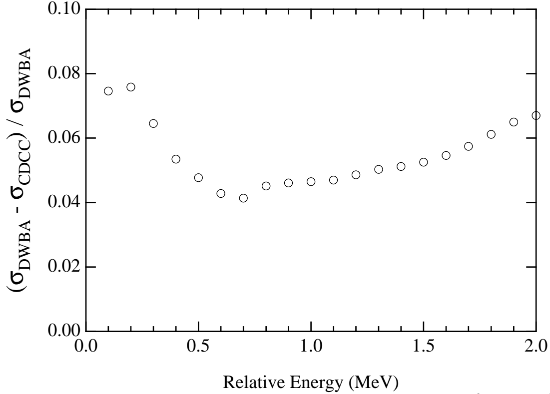
FIG. 18. Difference between the cross section for Coulomb breakup of 83 MeV/nucleon {}^8\text{B} on Pb for {}^8\text{B} scattering angles of 1.77^\circ and less predicted by DWBA (1st-order) and CDCC (all orders) calculations using the same structure model, expressed as a fraction of the DWBA prediction. Only Coulomb matrix elements were included in these calculations. No significant energy dependence of the higher-order electromagnetic effects is evident.
