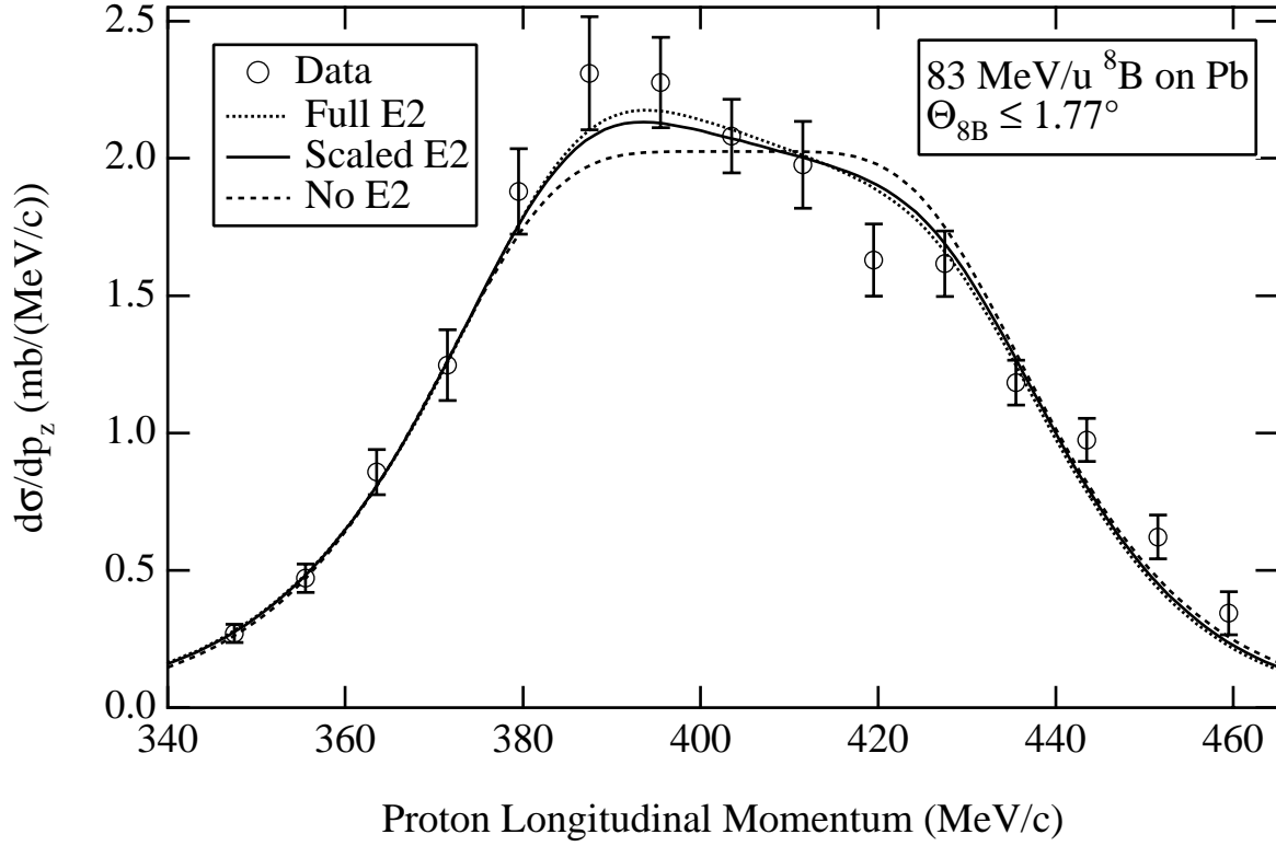
FIG. 13. Measured longitudinal momentum distribution of protons from the Coulomb dissociation of 83 MeV/nucleon {}^8\text{B} on Pb with {}^8\text{B} scattering angles \leq 1.77^\circ . Only relative errors are shown. Also depicted are 1st-order perturbation theory calculations with different E2 strengths, convoluted with the experimental resolution.
