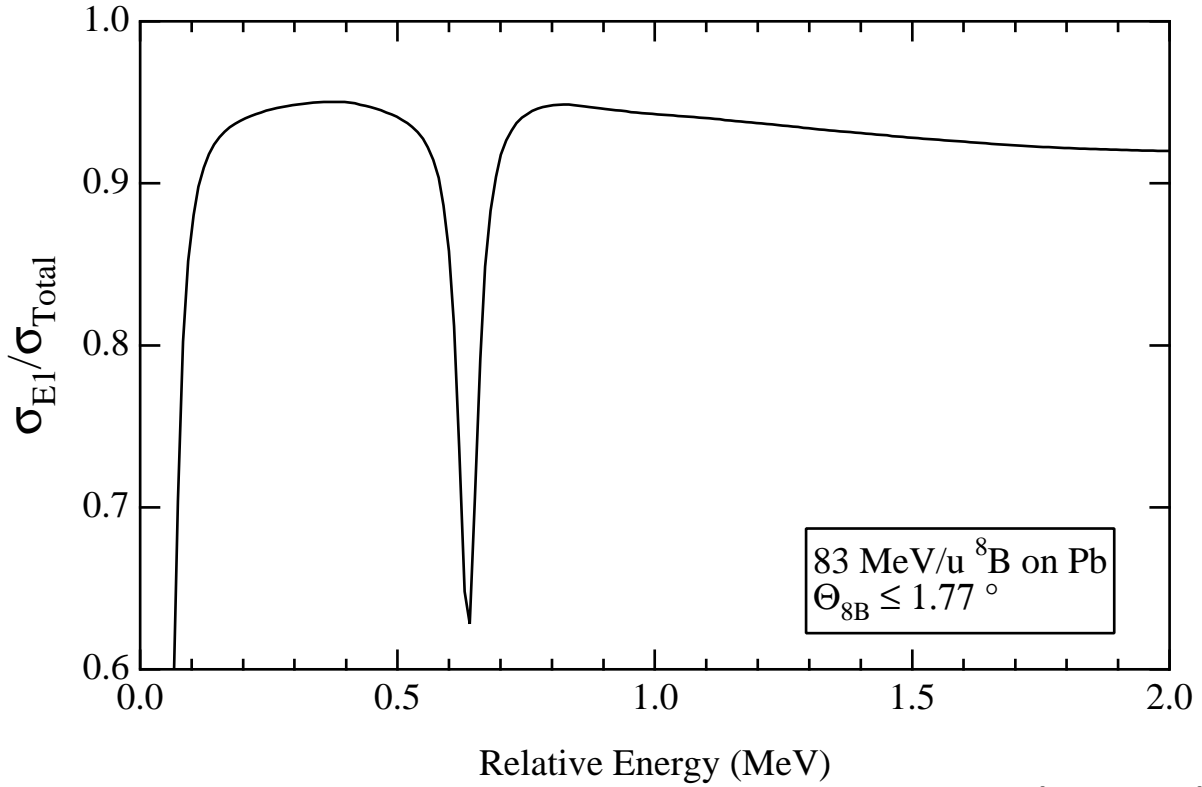
FIG. 16. Fraction of the calculated cross section for the Coulomb dissociation of 83 MeV/nucleon {}^8\text{B} on Pb with {}^8\text{B} scattering angles \leq 1.77^\circ ( b \geq 30 fm) accounted for by E1 transitions in 1st-order perturbation theory. As the energy falls below 130 keV, E2 transitions become increasingly important.
