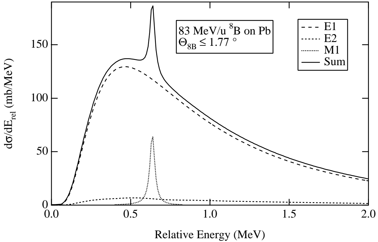
FIG. 15. Contributions of E1 , E2 , and M1 transitions to the cross section for the Coulomb dissociation of 83 MeV/nucleon ^8\text{B} on Pb with ^8\text{B} scattering angles \leq 1.77^\circ in 1st-order perturbation theory. The M1 cross section is calculated by folding the M1 S factor measured in ref. [8] with the virtual photon spectrum. The E1 and E2 cross sections are calculated using the model of ref. [25], scaling the E2 matrix elements by the factor 0.7 required to reproduce the measured ^7\text{Be} longitudinal momentum distributions.
