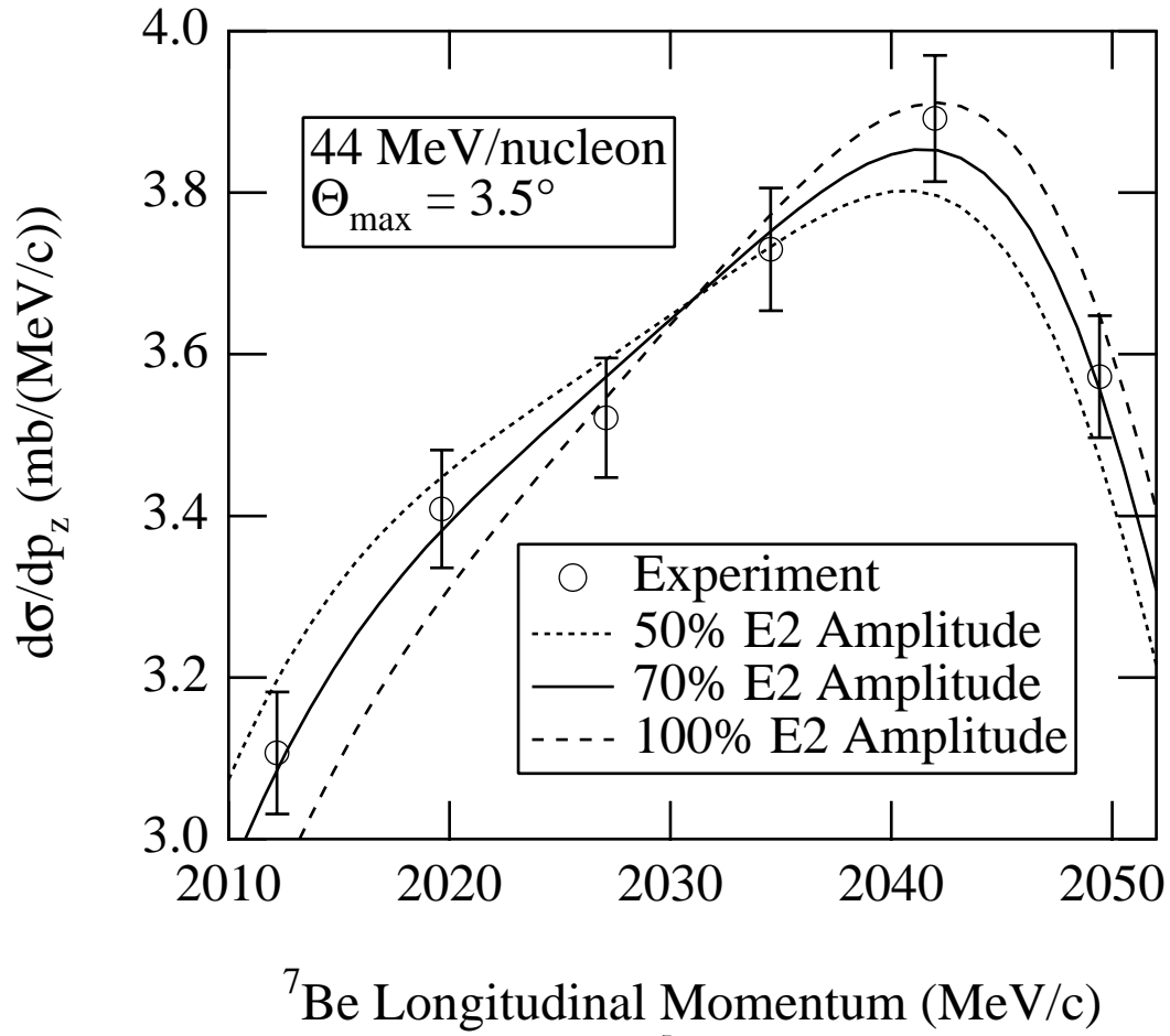
FIG. 14. Central region of the 3.5^\circ angle cut of the {}^7\text{Be} longitudinal momentum distribution from the breakup of 44 MeV/nucleon {}^8\text{B} on Pb. The curves are calculations performed with different E2 matrix elements, expressed in terms of the E2 amplitude of the model of [25], normalized to the center of the distribution.
