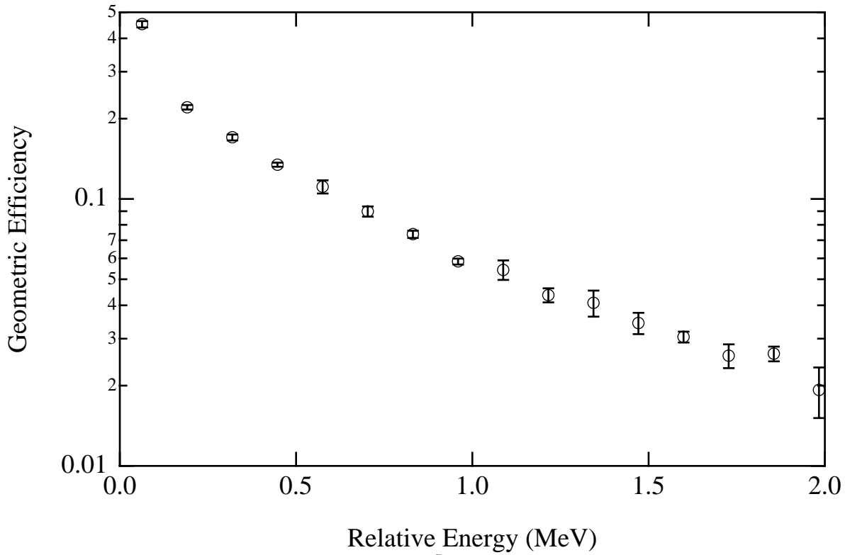
FIG. 7. Geometric efficiency for detecting protons and {}^7\text{Be} fragments in coincidence from the Coulomb dissociation of 83 MeV/nucleon {}^8\text{B} with impact parameters \geq 30 fm. The relative errors shown are statistical uncertainties from the simulation and theoretical uncertainties from the size of the E2 component, added in quadrature.
