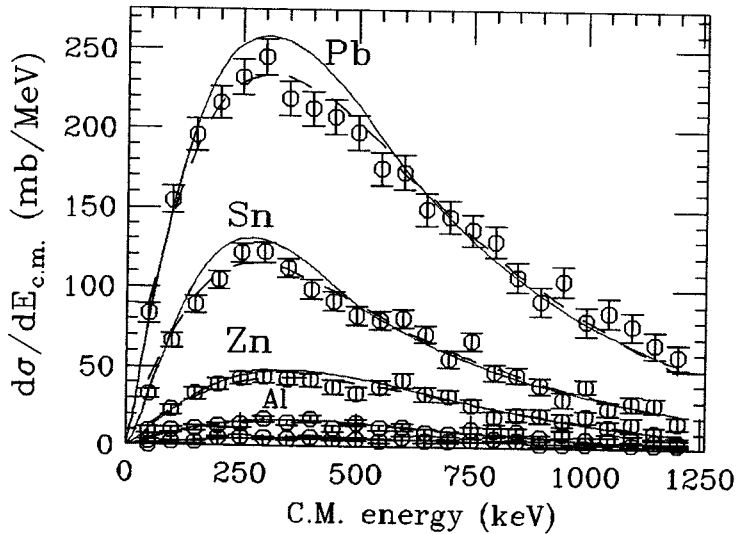
Fig. 5.—Dissociation excitation functions for C, Al, Zn, Sn, Pb targets (C at bottom). Open circles are the data with statistical error bars. When the solid lines, the intrinsic (true) functions, are folded with the instrumental resolution functions of Fig. 6, the dashed-line fits result.
