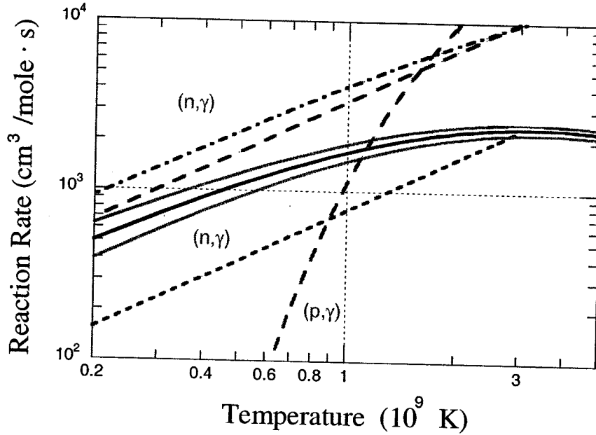
Fig. 9.—Reaction rates. Solid line enclosed by the gray error curves represents results of the present experiment. Dot-dashed curve (Descouvemont 2000), upper dashed curve (Wiescher, Görres & Thielemann 1990), and the (p,γ) curve (Kawano et al. 1991) result from calculations. Dotted curve is derived from measured \sigma_{n,\gamma} at 23 keV by Beer et al. 1992.
