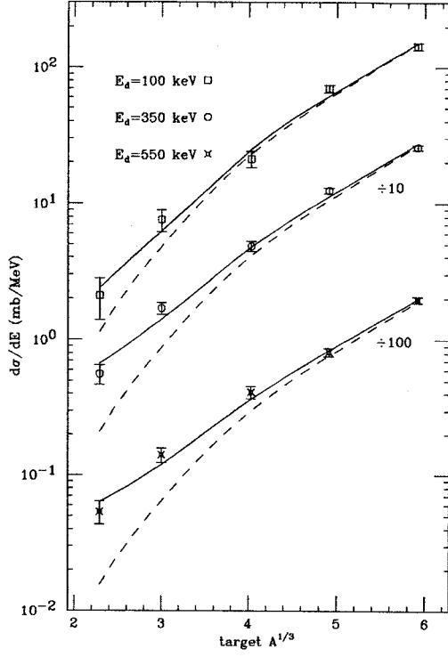
Fig. 7.—Total cross sections and Coulomb components of the dissociation at E_d=100 keV, 350 keV and 550 keV. Symbols are measured cross sections. Solid curves represent fits using Eq. 2. Dashed curves are the Coulomb parts of the measured cross sections. The bottom two sets of points and fits have been displaced downward for clarity.
