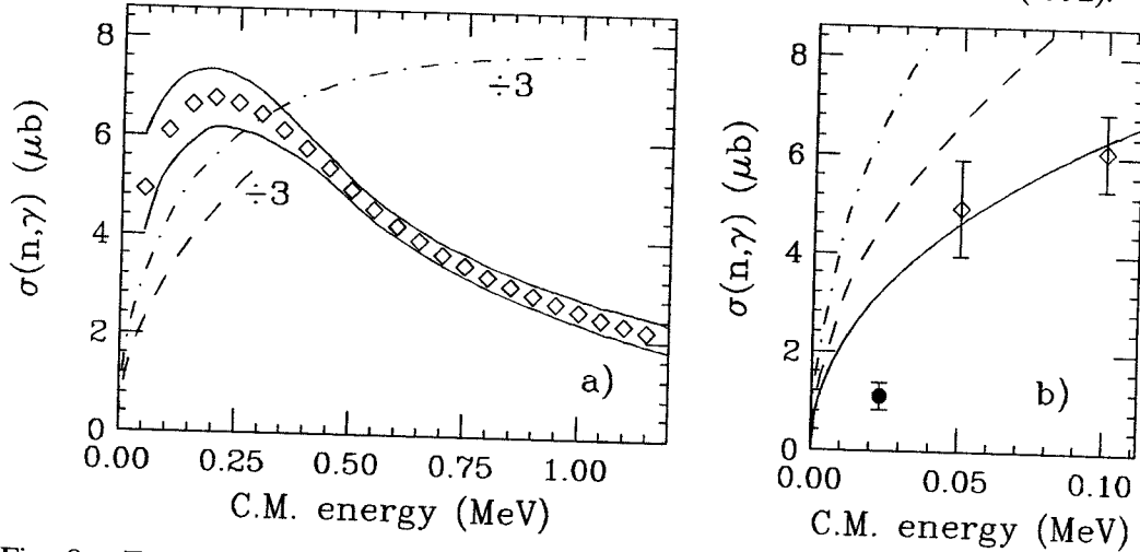
Fig. 8.—Excitation function for the ^{14}\text{C}(n,\gamma) cross section. (a) Points enclosed by two solid curves define the region of the experimental results. Plotted as 1/3 of actual values, the dashed curve is a prediction of Wiescher, Görres & Thielemann (1990), and the dot-dashed curve is a prediction of Descouvemont (2000). (b) Blowup of low-energy region showing same theoretical curves, but not \div 3 , the 1990 result of Beer et al. (solid point) and our lowest-energy points (diamonds) with a kinematical fit (solid curve).
