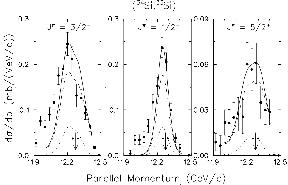
FIG. 4. Measured momentum distribution (full points) compared with predictions within the transfer-to-the-continuum model according to [20] for the ( ^{34}\text{Si}, ^{33}\text{Si} ) reaction leading to the ground state (left), the 1.01 MeV state (middle), and the 4.32 MeV state (right). The full curves show the total neutron removal cross section in comparison to stripping (dashed) and diffraction breakup (dotted), all calculated for the same incident beam energy of 70.6 A MeV corresponding to a momentum of 12.192 GeV/c in this figure. For the proposed d_{3/2} removal the theoretical distribution has been scaled to match the data by a factor of 1.32, for d_{5/2} by 0.7. The arrows indicate the momentum corresponding to experimental projectile velocity.
