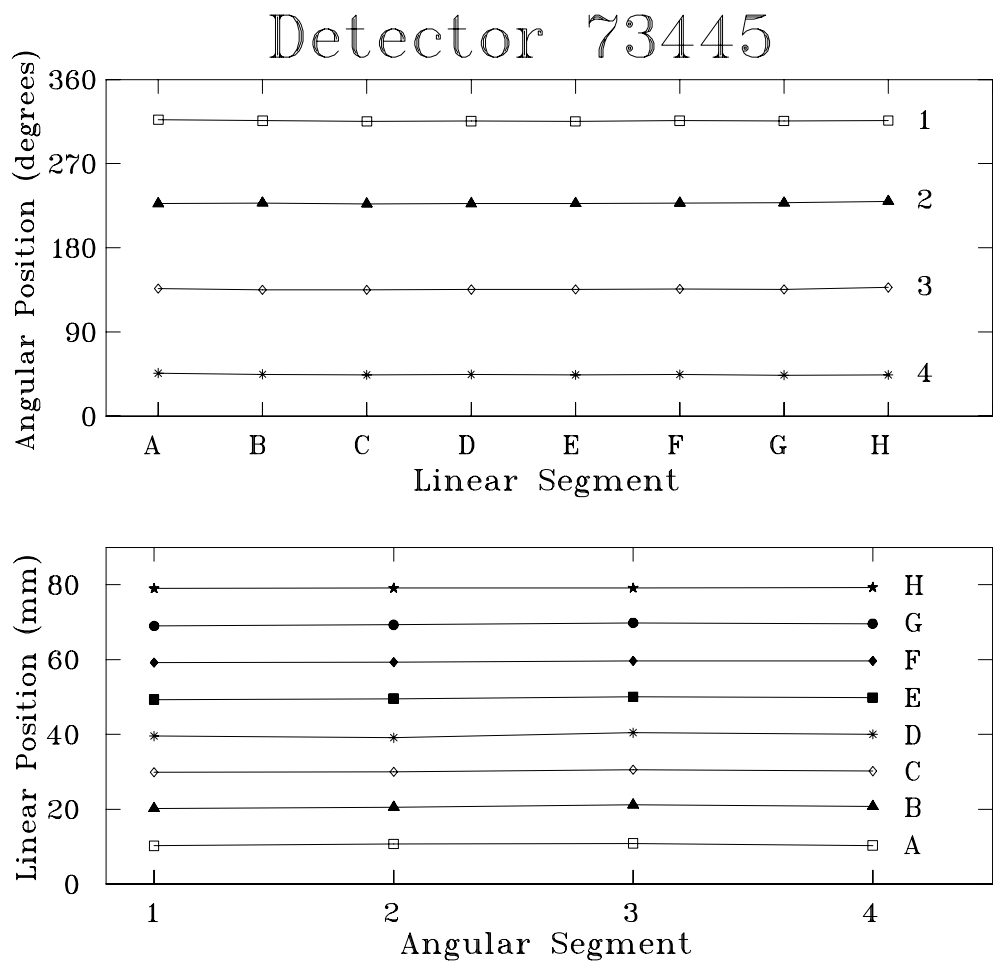
Fig. 5. Angular and linear center positions for the thirty-two segments of detector 73445. Error bars for both linear and angular positions are smaller than the plotting symbol.
