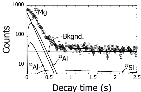
Fig. 3. ^{33}\text{Mg} decay curve, showing fit components.
