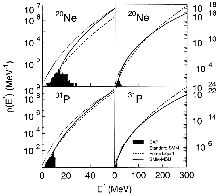
FIG. 4: Level densities as a function of excitation energy for ^{20}\text{Ne} and ^{31}\text{P} . Two energy ranges are plotted to show the behaviors of level densities at both low (left panels) and high energy (right panels) ends. The density of experimentally known levels is shown as bars in the low energy region. The dashed lines are the extrapolations of the empirical values according to Eq. 25. The dotted lines are the level density (Eq. 20) parametrized from the SMM85. The solid lines are the level density adopted in this work (Eqs. 31-34).
