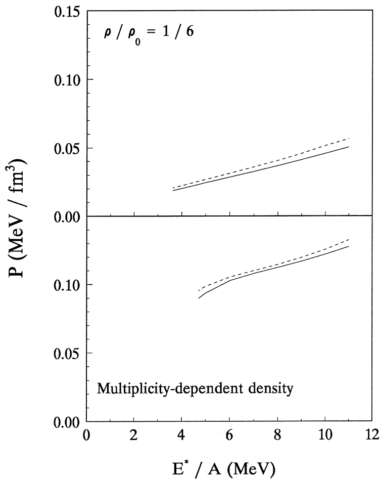
FIG. 8: Pressure curves due to kinetic motion and Coulomb interaction (see Eq. 40) are plotted for the system of A=168 and Z=75 at fixed breakup density and multiplicity-dependent density. The dotted lines are calculated from the SMM85 while the ISMM presents the solid lines.
