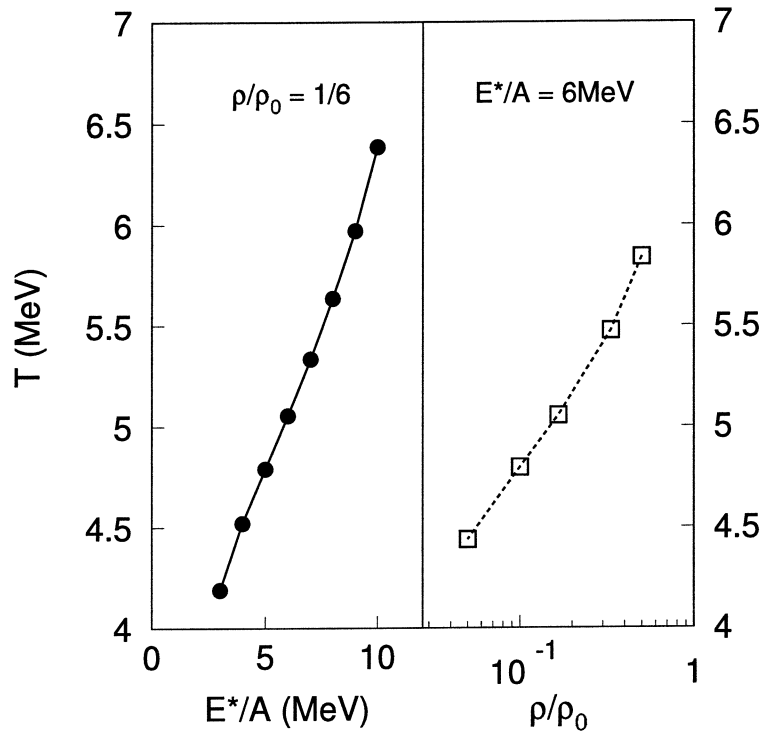
FIG. 10: Dependences of temperature on excitation energy and breakup density are shown for the system of A=168 and Z=75 . Calculations as function of excitation energy at fixed density of 1/6 normal density are shown as solid circles in the left panel. Calculations as function of density at fixed excitation energy are shown as open squares in the right panel.
