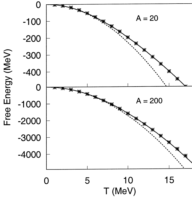
FIG. 3: Internal free energies for A = 20 (upper panel) and A = 200 (lower panel). The SMM85 expression [Eq. (16)] is represented by the full line whereas the dashed lines stand for the results obtained with the Taylor expansion [Eq. (18)]. The Free energy calculated through the level density given by Eq. (20) is depicted by the symbols.
