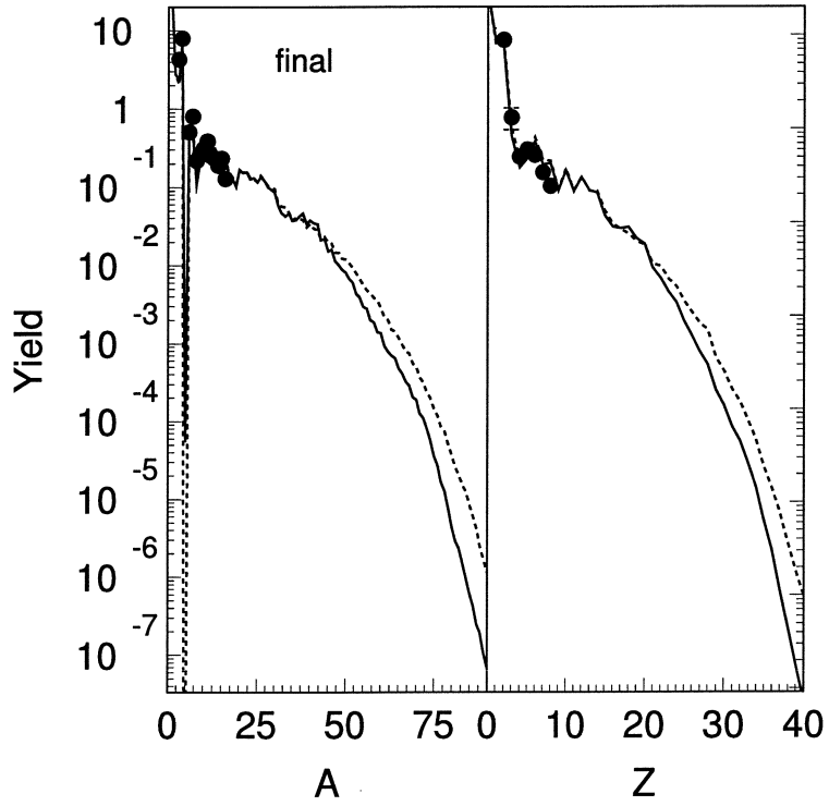
FIG. 12: Final mass and charge distributions after applying MSU-DECAY, the empirical secondary decay procedure discussed in Sect. III. The dashed lines are calculated from the primary results of the SMM85 while the solid lines are from ISMM.
