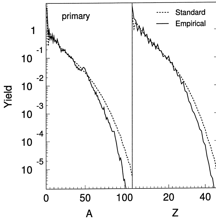
FIG. 11: Mass and charge distributions for the system of A=186 and Z=75 . The dashed lines are the calculations from the SMM85. The solid lines are calculated using the improved model ISMM.
