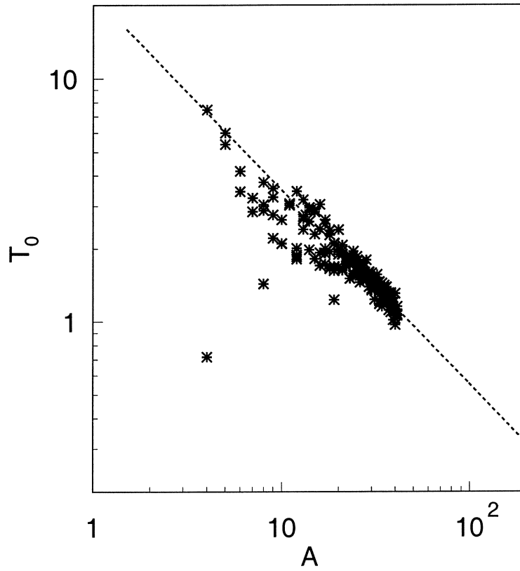
FIG. 6: Best fit values of T_0 for different nuclei (symbols). The dashed line corresponds to Eq. 36 used for Z > 15 .
