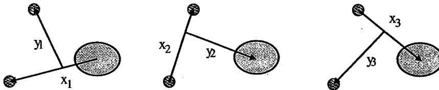
Figure 1. Jacobi coordinates for the three-body problem.
