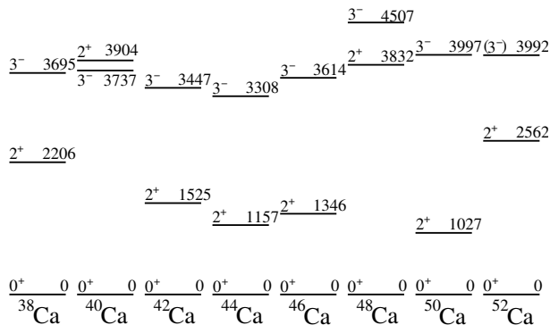
FIG. 3: Systematics of the first 2^+ and 3^- excitations along the even-even Ca isotopic chain (data from Ref. [17–19]).
