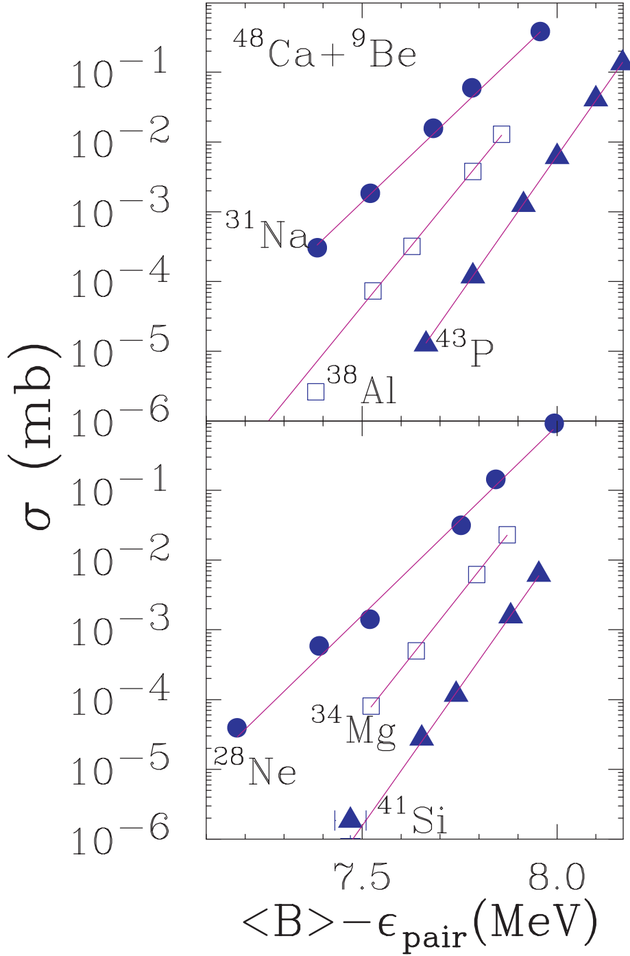
FIG 3: (Color online) Fragmentation cross sections of neutron rich isotopes of Ne, Na, Mg, Al, Si, and P elements produced from ^{48}\text{Ca}+^9\text{Be} reaction, plotted as a function of binding energy per nucleon with pairing corrections. Odd Z isotopes are plotted in the top panel and even Z isotopes in the bottom panel. Lines show the best fits of Eq (2) using the parameters listed in Table 1.
