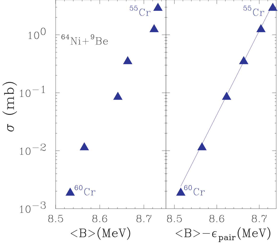
FIG 4: (Color online) Fragmentation cross section plotted as a function of average binding energy for neutron-rich chromium isotopes produced from the fragmentation of ^{64}\text{Ni} + ^9\text{Be} reaction. In the right panel, pairing energy has been subtracted from ^{56,58,60}\text{Cr} isotopes to minimize the odd-even effects. The line is the best fit through the data points using Eq. (2) with the parameters listed in Table 2.
