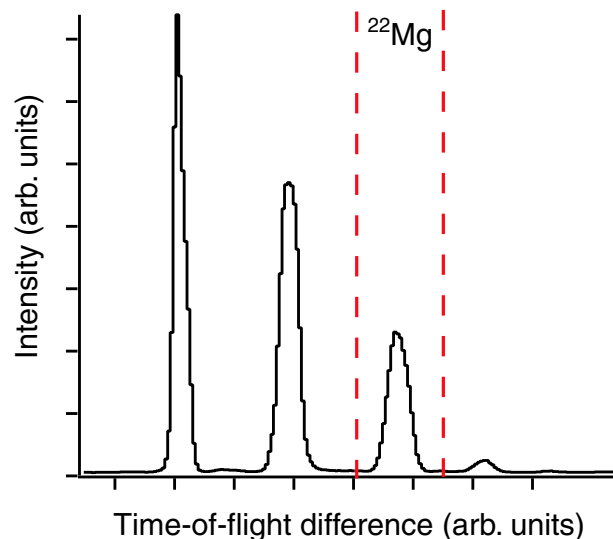
FIG. 2: (Color online) Time-of-flight (TOF) difference taken between two plastic scintillators positioned before the reaction target. The constituents of the cocktail beam are well separated in TOF. A software gate is then applied to unambiguously select reaction residues produced by one incoming species only, here ^{22}\text{Mg} .
