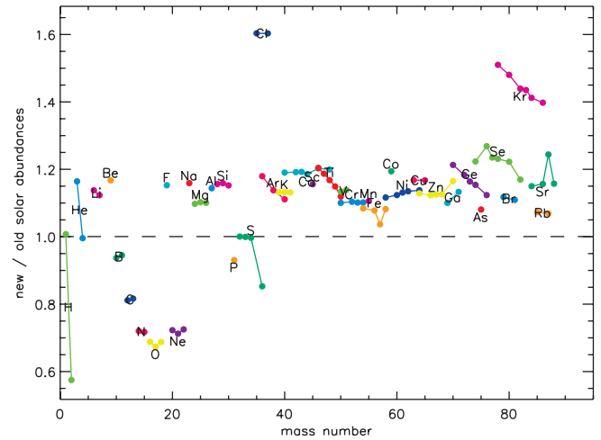
FIG. 2.—Ratio of the Lodders (2003) abundances to the Anders & Grevesse (1989) abundances as a function of mass number (up to strontium). Isotopes of each element have the same color and are connected by lines.
