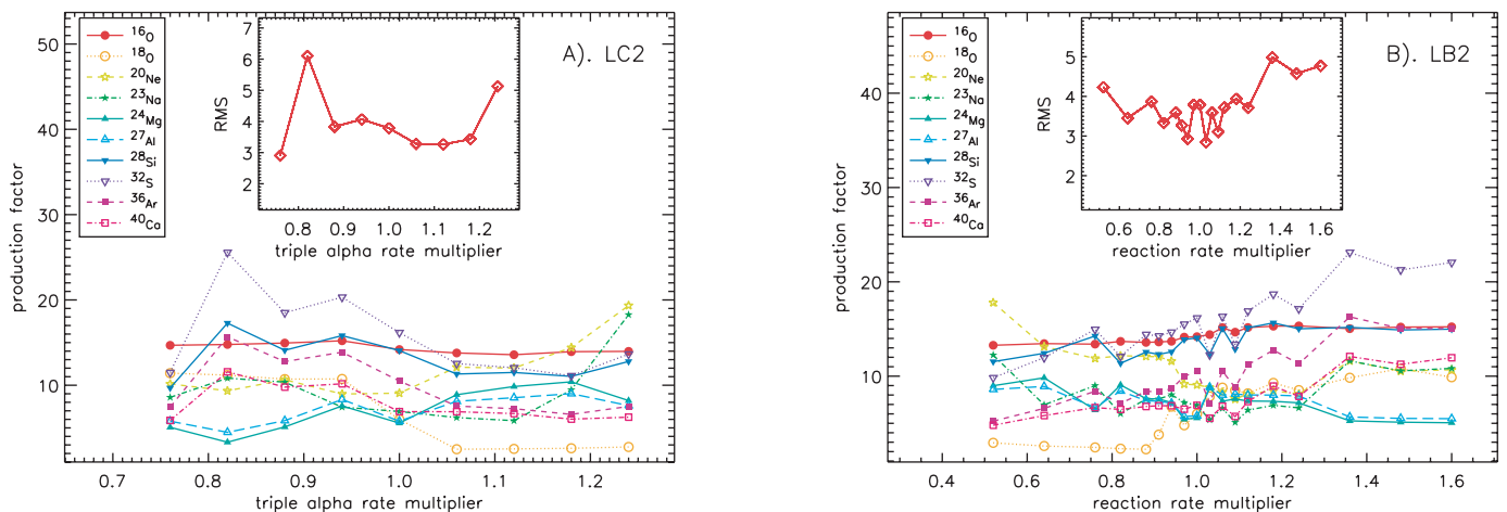
FIG. 6.—(a) Production factors and their rms deviations from the mean for some medium-weight isotopes (the same set as M. Boyes et al. 2002, unpublished) for LC2. (b) Same as (a), but for LB2.
