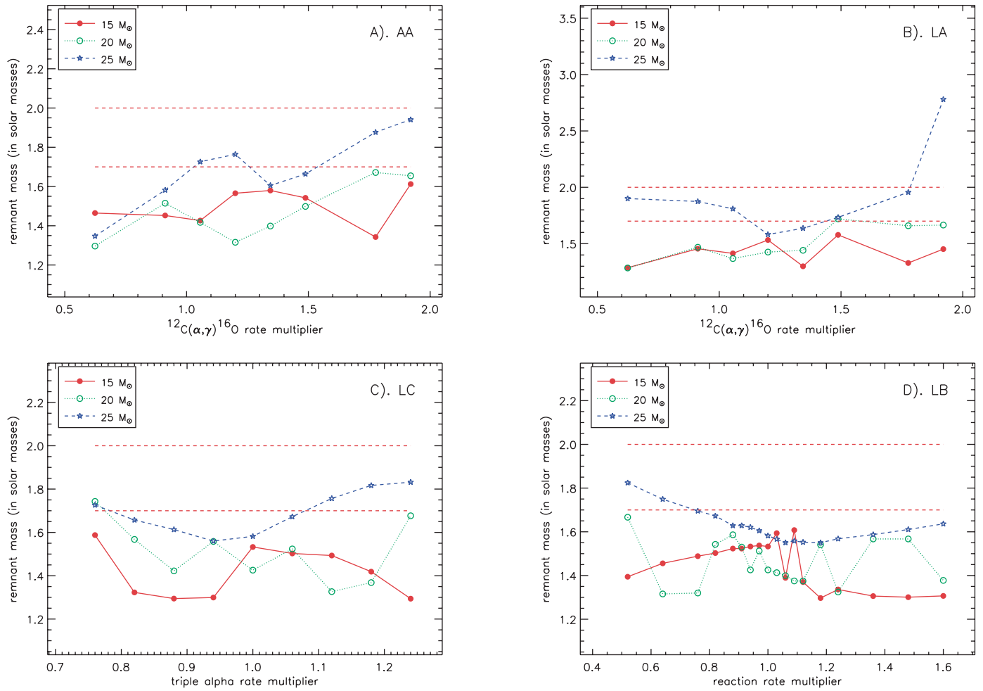
FIG. 5.—Gravitational mass of the remnant (neutron star or black hole) after explosion for 15, 20, and 25 M_{\odot} stars. The dotted lines at 1.7 and 2.0 M_{\odot} mark possible maximum masses for neutron stars (Lattimer & Prakash 2007); for heavier masses, black holes may be formed. (a) AA series. (b) LA series. (c) LC series. (d) LB series.
