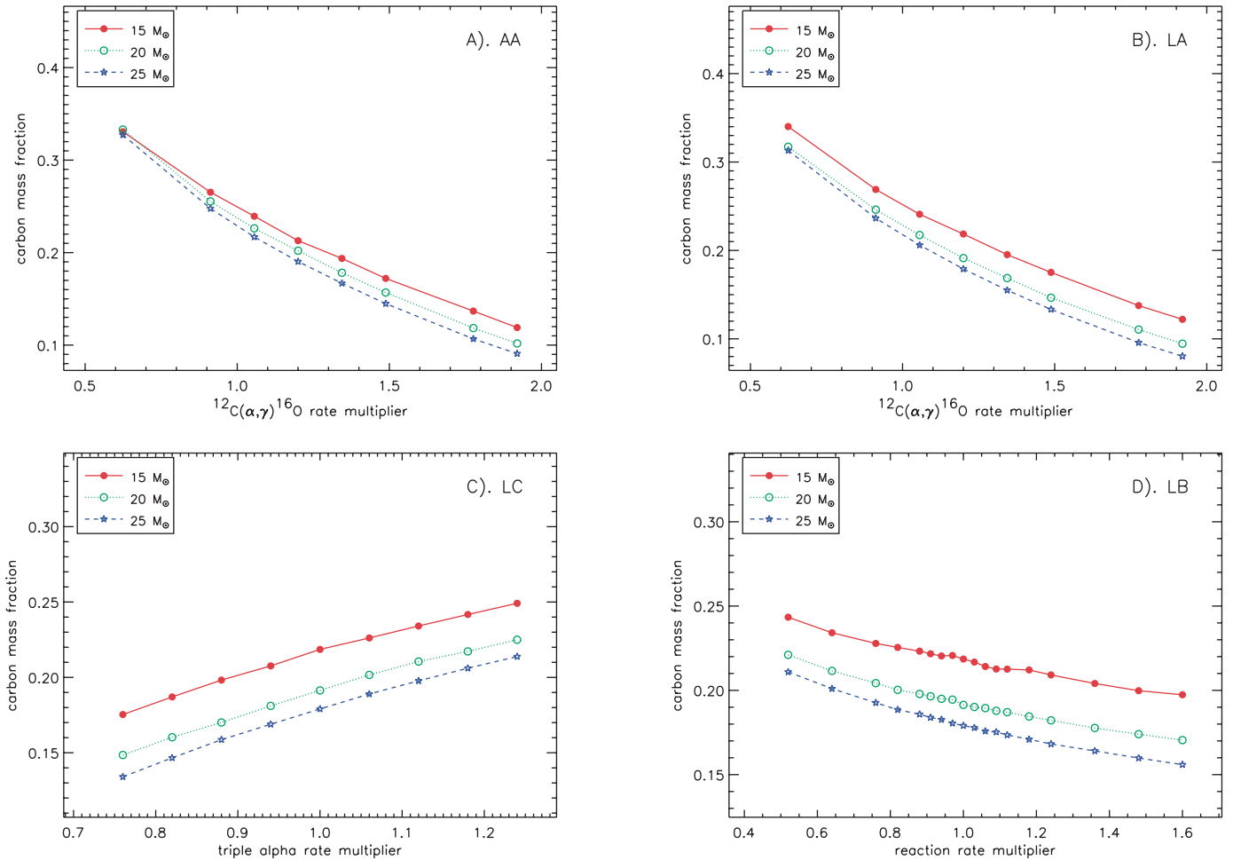
FIG. 4.— (a) Carbon mass fraction at the center of the star at core carbon ignition for 15, 20, and 25 M_{\odot} stars and for the AA series. (b) Same as (a), but for LA. (c) Same as (a), but for LC. (d) Same as (a), but for LB.
