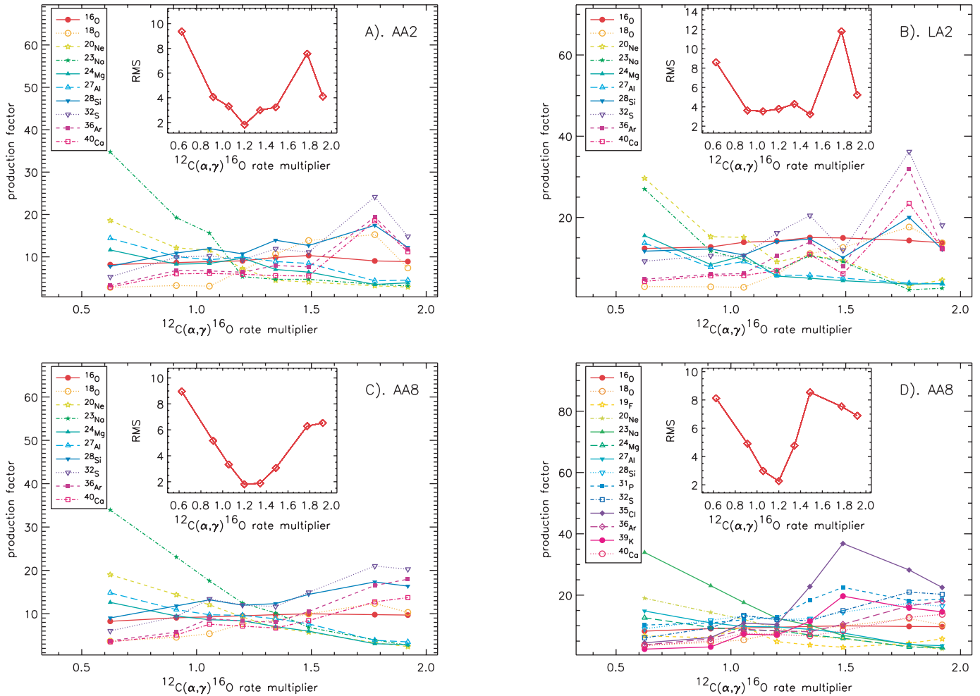
FIG. 3.—(a) Production factors for AA2 and their rms deviations from the mean for the same set of isotopes as those selected by M. Boyes et al. (2002, unpublished). A multiplier of 1 means a rate of 1 times the rate recommended by Buchmann (1996). (b) Same as (a), but for LA2. (c) Same as (a), but for AA8. (d) Same as (c), but with the addition of the production factors for ^{19}\text{F} , ^{31}\text{P} , ^{35}\text{Cl} , and ^{39}\text{K} .
