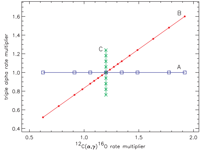
FIG. 1.— Lines and dots show the three sets of simulations done for each star of a given initial mass and a given initial solar abundance distribution. For the blue squares, R_{3\alpha} is held constant (at its value by Caughlan & Fowler 1988) and R_{\alpha,12} is varied (A). For the red dots, both reaction rates are varied by the same percentage, so their ratio remains constant (B). For the green crosses, R_{\alpha,12} is held constant at 1.2 times the rate recommended by Buchmann (1996) and R_{3\alpha} is varied (C).
