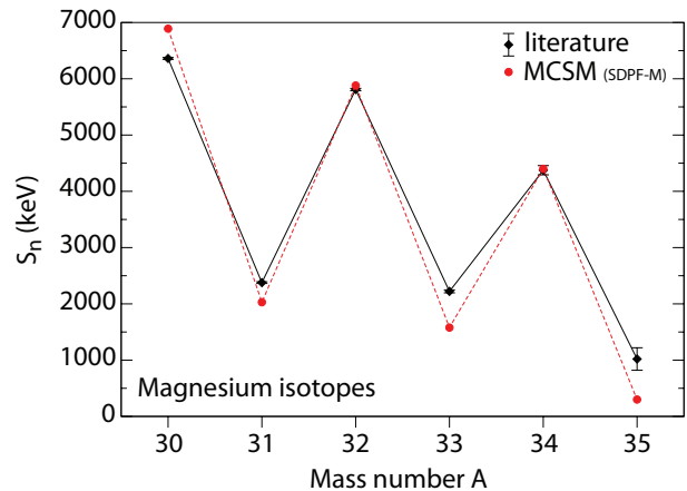
FIG. 4: (Color online) Neutron separation energies, S_n , for neutron-rich magnesium isotopes from literature ( A = 30 - 33 taken from [32], A = 34, 35 based on the mass excess reported in [31]) compared to the MCSM (SDPF-M) calculations. The overestimated odd-even staggering supports the assumption that pairing effects are overestimated, leading to an underestimation of S_n for the odd- A isotopes by several hundred keV.
