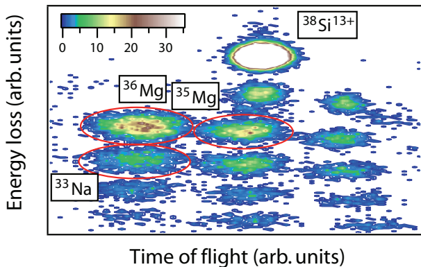
FIG. 1: (Color online) Identification spectrum for the reaction residues produced in {}^9\text{Be}({}^{38}\text{Si}, {}^A\text{Z})\text{X} at 83 MeV/u mid-target energy. All reaction residues can be unambiguously identified by plotting the energy loss measured in the S800 ionization chamber versus the ion's time of flight. The magnetic rigidity of the S800 spectrograph was set to center {}^{36}\text{Mg} in the focal plane (see [13]). The H-like charge state of the projectile beam - produced by electron pickup of the originally fully-stripped {}^{38}\text{Si} passing through the reaction target - is the most intense constituent of the reacted beam.
