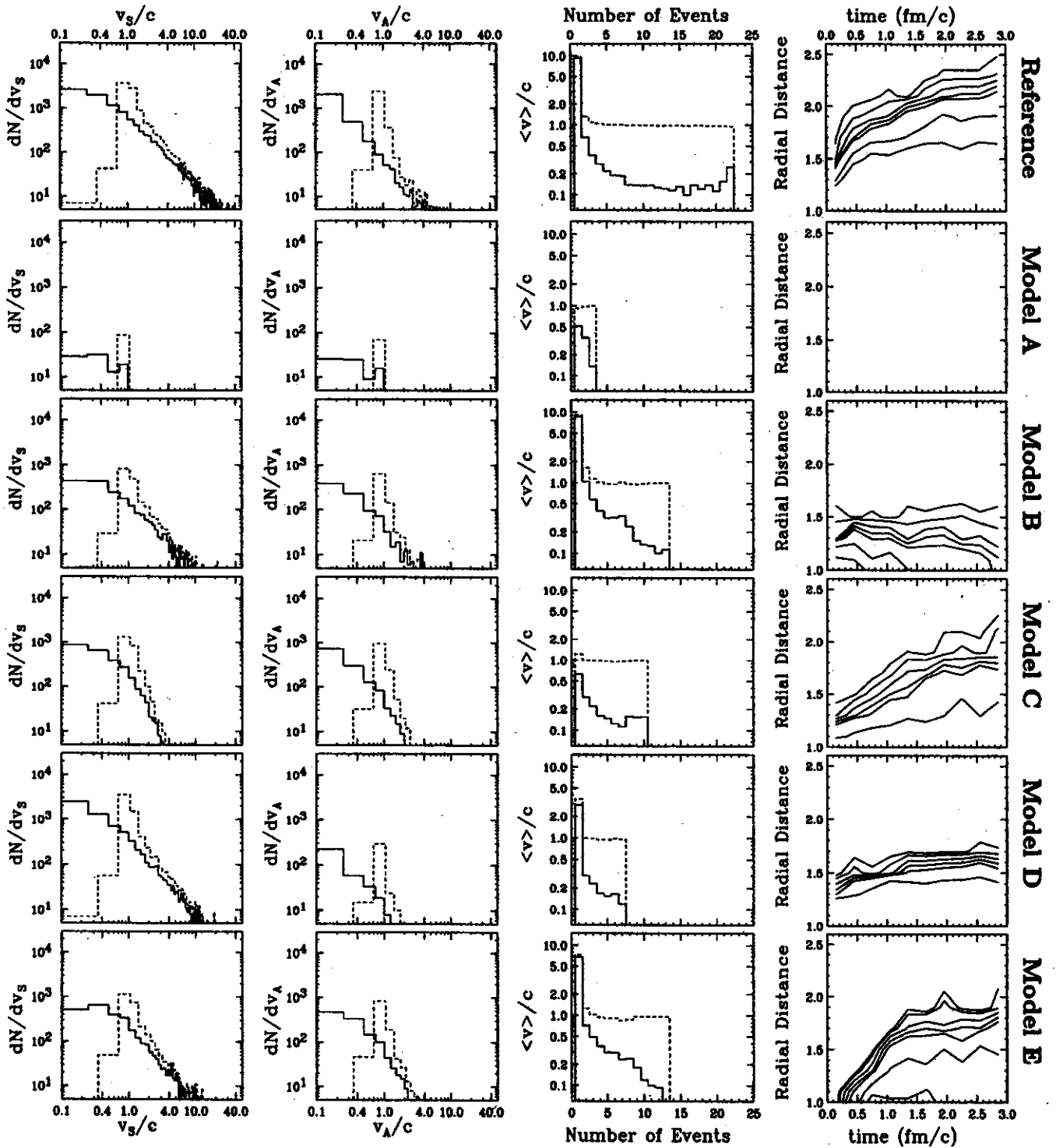
FIG. 7. Results of simulations with different mechanisms to suppress superluminal signal transport. The leftmost histogram shows the signal velocity distribution regarding directly subsequent collisions, v_s ; see Fig. 1. The solid histogram shows the radial component of those velocities, the dashed histogram includes the longitudinal component. The second panel shows a more general impression of the signal velocities, in this histogram the signal velocity v_A from the very first to the very last scattering event that a parton was involved in is calculated. Again, the solid histogram shows the radial component of the signal velocities, the dashed histogram also takes into account the longitudinal components. The third panel shows how subsequent scattering events are leading to this overall damping of peak velocities occurring in single scattering events: again starting from the very first scattering event of a parton, the average signal velocity ( v ) to the i th following scattering event of the partons is calculated; both the total and only the radial component of the velocities are shown. Finally, the rightmost panel shows the outgoing shock wave, in a plot of distance from the beam axis versus simulation time the contour lines of the scattering event distribution are given. For model A, the rejection of any individual scattering events that would lead to superluminal signal transport, the shock wave was so strongly damped that it did not even go beyond the radius of the incoming proton.
