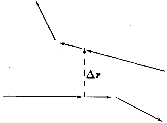
FIG. 8. A first step to the introduction of retarded interactions: After the scattering took place, the partons maintain their momentum for a time period of |\Delta r|/(2c) in which they are not able to scatter with other partons. Only after this time the momenta are transferred to the partons.
