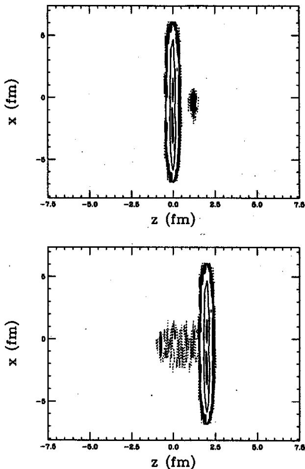
FIG. 9. Initial configuration and configuration after 2 fm/c for a simulation with wee partons.
