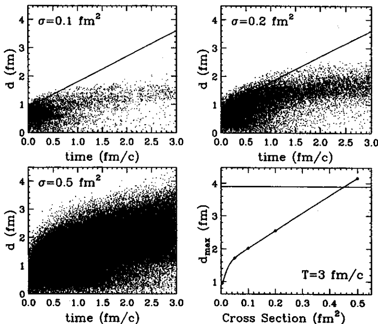
FIG. 2. Distance d of scattering events versus simulation time at constant cross sections of \sigma = 0.1, 0.2, \text{ and } 0.5 \text{ fm}^2 . The solid line indicates the distance that could be reached by a signal that travels with the speed of light. One can clearly see the outwards traveling shock wave and how it gets damped out with time. For the smaller cross sections the causality violation is rather small and only present in the initial stages of the interaction. One should note that for realistic energy-dependent cross sections the initial scattering events take place with a lower cross section than the later ones because the c.m. energy is much higher. In the lower right panel the maximum distance d_{\text{max}} of scattering events from the beam axis is plotted versus the cross section \sigma . The horizontal line indicates a distance that during the simulation time could only be reached with the speed of light.
