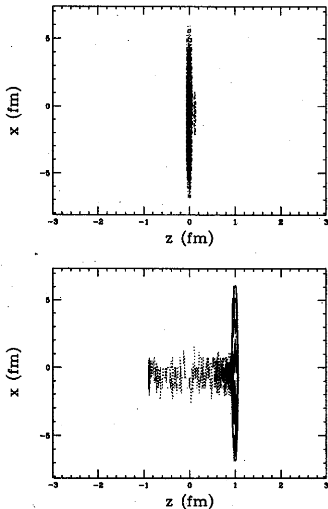
FIG. 6. In the top panel the projection of the initial parton configuration on the (x, z) plane is depicted. The highly Lorentz-contracted proton is moving to the left into the equally contracted gold nucleus which is moving to the right. The bottom panel shows the configuration 1 fm/c later.
