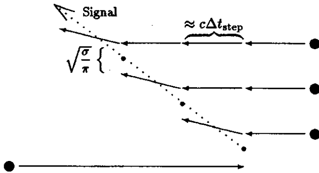
FIG. 1. One particle coming from the left scatters with another particle coming from the right. As part of the model the scattered particles cannot scatter again in this time step. However, one time step later that scattered particle from the right scatters with another particle coming from the right. As a result information from the first scattering, such as particle momenta and type, has traveled to the second one. This kind of information transport can continue over several scattering events.
