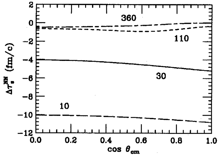
Figure 3: Spin-isospin averaged time delay for NN scattering as a function of the cosine of c.m. scattering angle, at several values of laboratory kinetic energy indicated in the figure in MeV.
