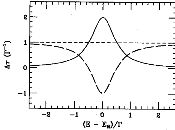
Figure 1: Time delays in the case of a Breit-Wigner resonance as a function of energy from the resonance divided by the width. The solid line represents the time for the scattered wave \Delta\tau_s . The short-dashed line represents the time \Delta\tau'_s which is ergodically consistent when the delay for forward wave or mean field are neglected. Finally, the long-dashed line shows the time delay for the forward wave divided by the fraction of the incoming wave that is scattered, \Delta\tau'_s - \Delta\tau_s (cf. Eq. (5.3)).
