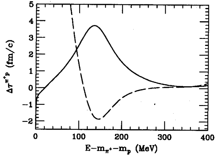
Figure 2: Time delays for a \pi^+p system as a function of c.m. kinetic energy. The solid line represents the time delay for the scattered wave averaged over angles and spin directions, \Delta\tau_s . The dashed line represents the forward time delay averaged over spin directions and divided by the fraction of the incoming wave that is, on the average, scattered, \Delta\tau'_s - \Delta\tau_s .
