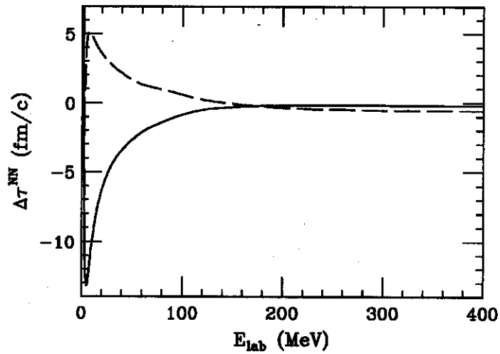
Fig 4: Time delays for NN system as a function of laboratory kinetic energy. The solid line represents the time for the scattered wave \Delta\tau_s averaged over the scattering angle and the spin and isospin directions. The dashed line represents the time for the forward wave, averaged over spin and isospin directions and divided by the fraction of incident wave scattered, \Delta\tau_s^f - \Delta\tau_s .
