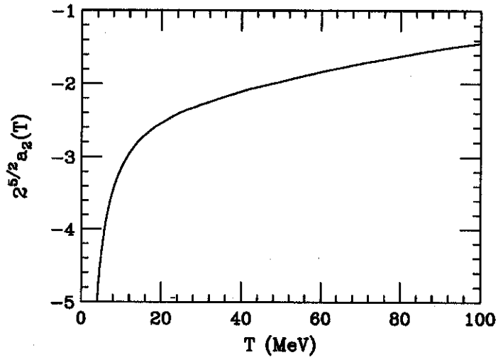
Fig. 5: Second virial coefficient for nuclear matter, multiplied by 2^{5/2} , from Eq. (6.7), as a function of temperature.
