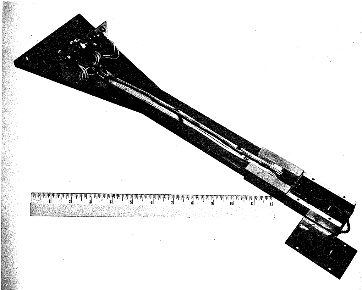
Fig. 9: The probe mount with one thermocooler and its heat sink removed to show the position of the module.
