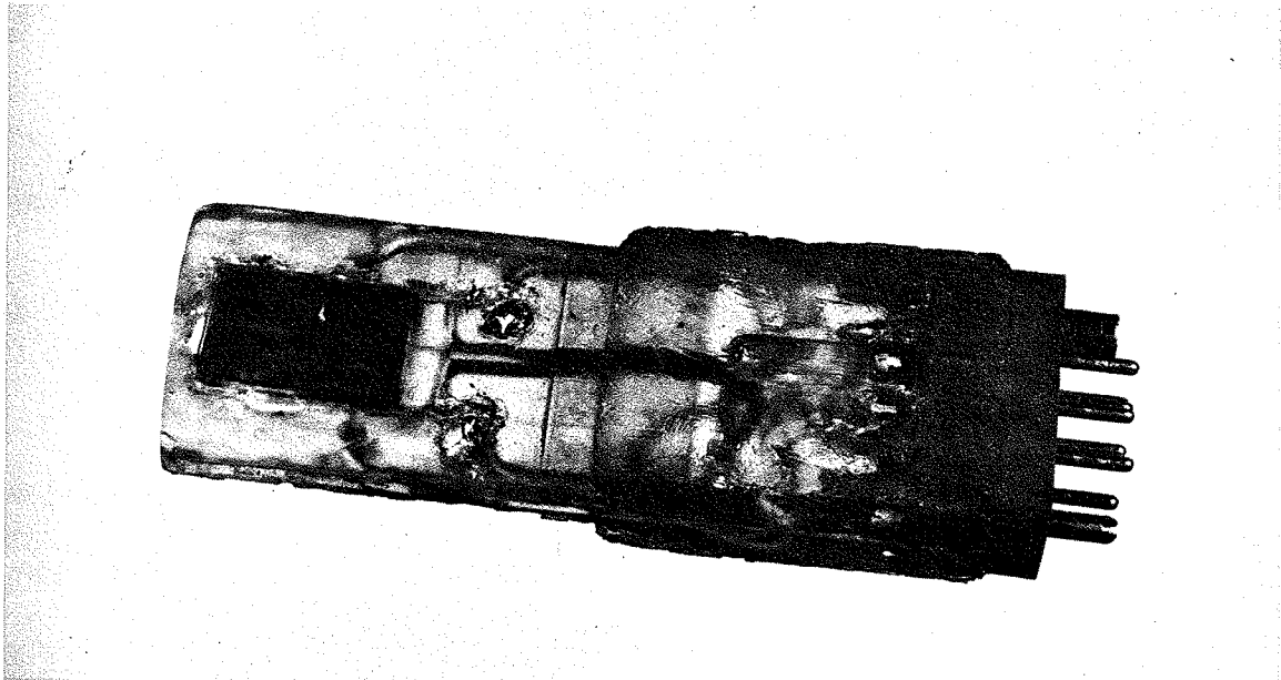
Fig. 8: The epoxy module containing Hall probe and thermistors.
