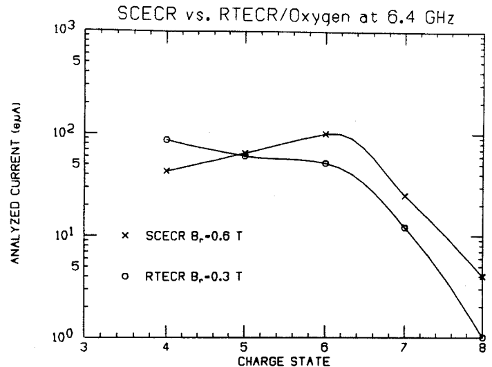
Figure 4. A comparison of the oxygen ion production of the RTECR and SCECR ion sources operated at 6.4 GHz. See text for details.
