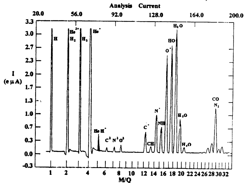
Figure 3. The He+H charge state distribution of the CPECR, showing the presence of the HeH + molecule, used to produce low energy H beams in the K1200 cyclotron.
