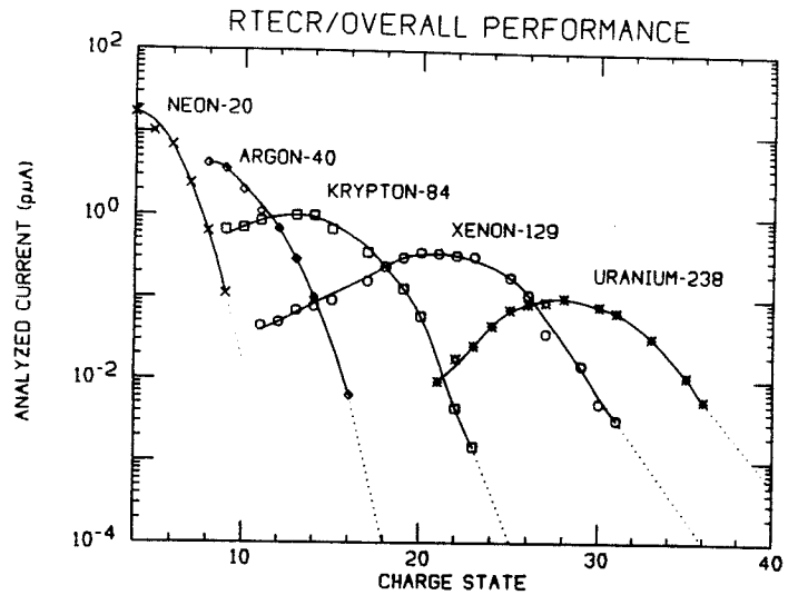
Figure 2. The optimized performance of the RTECR is smooth in Q and Z.
