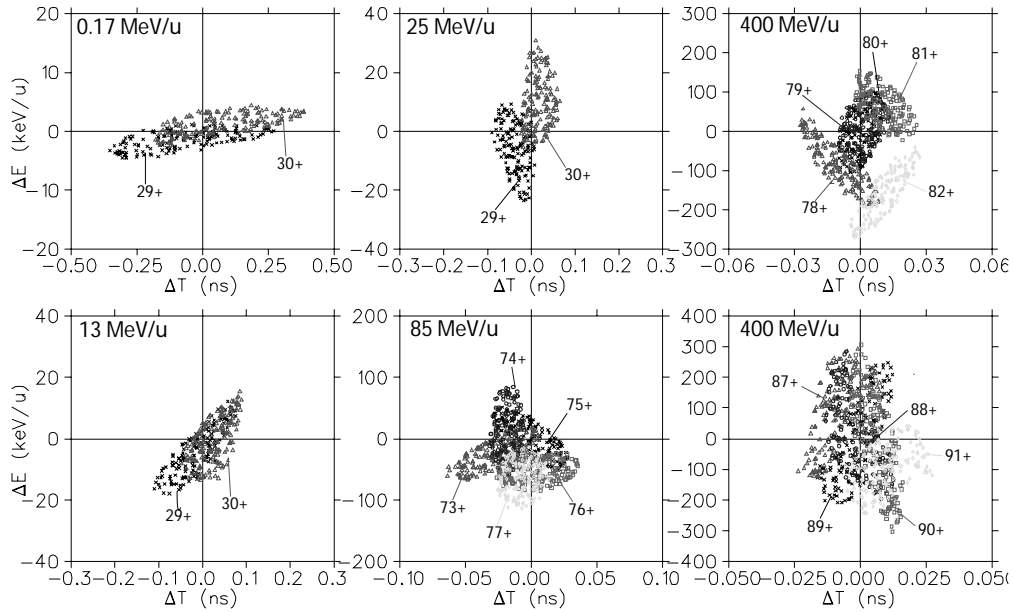
Figure 2: Longitudinal phase spaces at several stages of the linac. Upper plots: single charge stripping station at 25 MeV/u. Lower: two charge stripping stations at 13 and 85 MeV/u.
