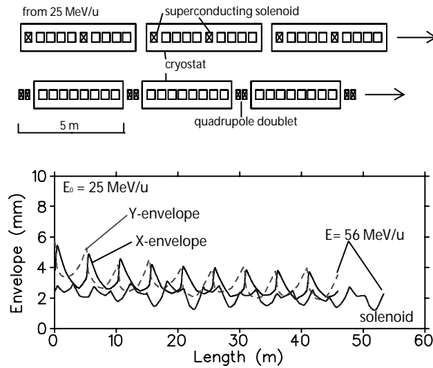
Figure 3: Upper: Two different layouts of focusing elements downstream of the charge stripping section (25 MeV/u) using either superconducting solenoids or normal-conducting quadrupole doublets. The layouts of the elements and cryostats are generated from the input table used for the beam dynamics calculations. Lower: The beam envelopes for a normalized rms emittance of 0.15 \pi mm-mrad.
