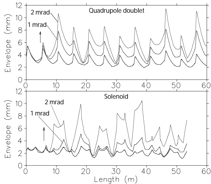
Figure 4: Beam envelopes resulting from rotational misalignment of the focusing elements for values of 0, 1 and 2 mrad. The arrows indicate the locations of misaligned elements.
